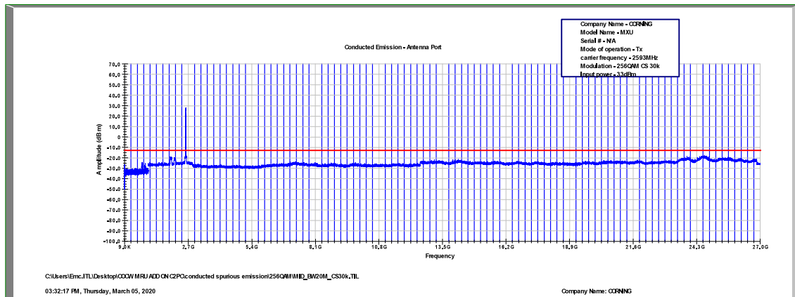
Figure 564: Spurious Emissions at Antenna Terminal 256QAM, 2593.0MHz, B.W. 20MHz, Sub Carrier 30kHz
