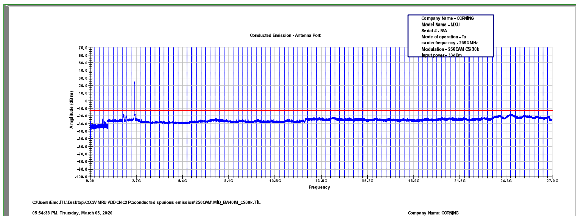
Figure 573: Spurious Emissions at Antenna Terminal 256QAM, 2593.0MHz, B.W. 40MHz, Sub Carrier 30kHz
