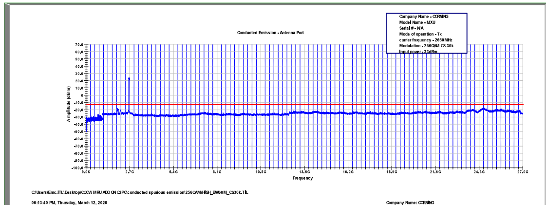
Figure 580: Spurious Emissions at Antenna Terminal 256QAM, 2660.0MHz, B.W. 60MHz, Sub Carrier 30kHz
