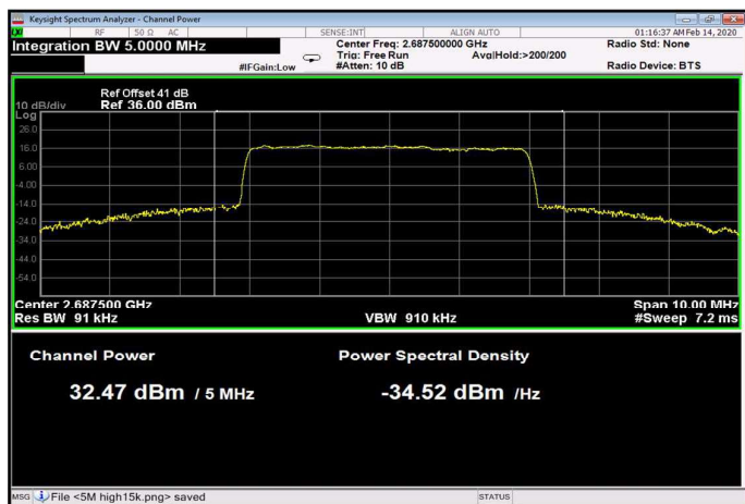
Figure 108: 256QAM 5MHz B.W.; 2687.5MHz, 15kHz
