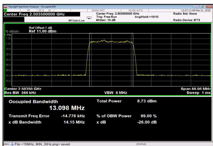
Figure 217: 64QAM 15MHz B.W.; 2503.5 MHz, 60kHz Input
