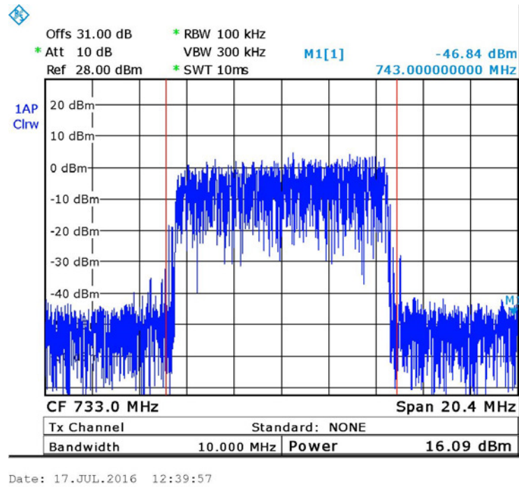
Figure 11. — 64QAM, 733 MHz
