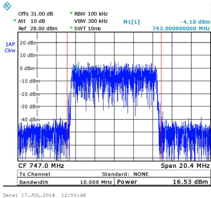
Figure 18. — QPSK 747 MHz
