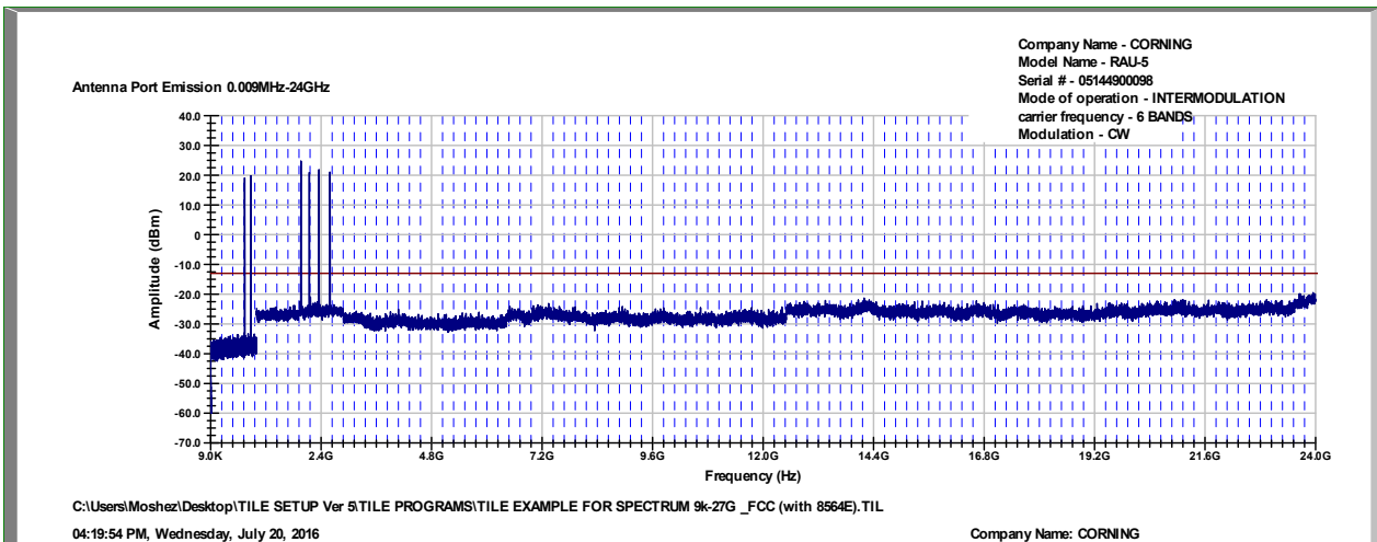
Figure 61 Intermodulation Conducted
