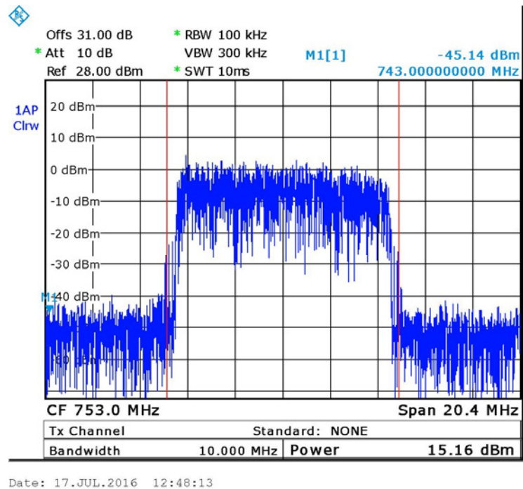
Figure 13. — 64QAM 753 MHz
