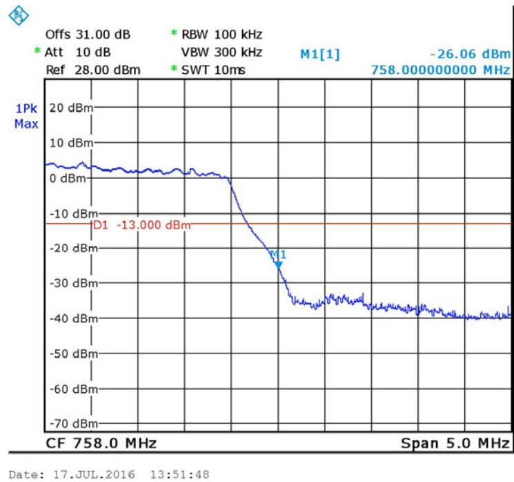
Figure 57. — QPSK 753.0 MHz
