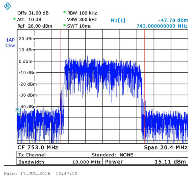
Figure 16. — 16QAM 753 MHz
