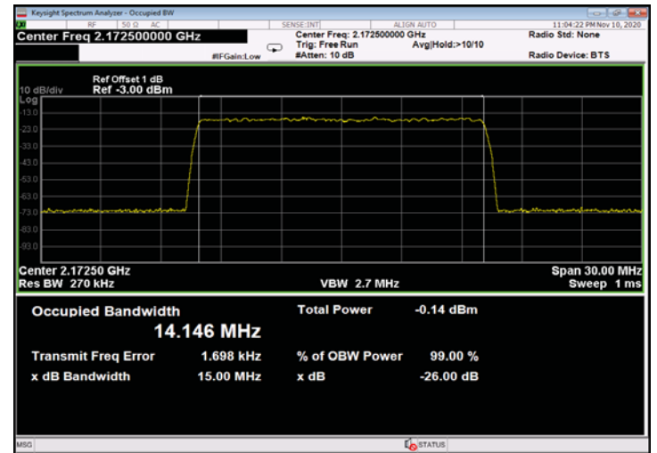
Figure 426: 256QAM 15MHz B.W.; 2172.5MHz, 15kHz - Input
