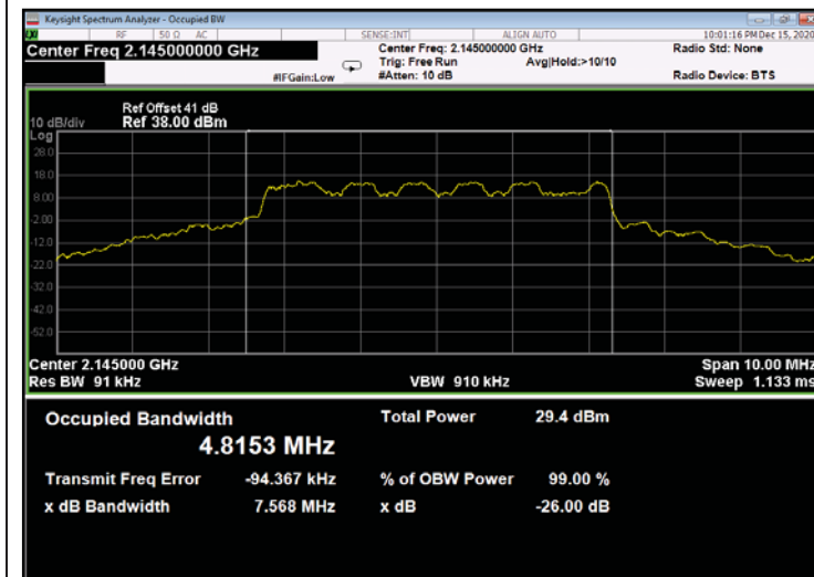
Figure 539: 16QAM 5MHz B.W.; 2145.0MHz, 15kHz - Output
