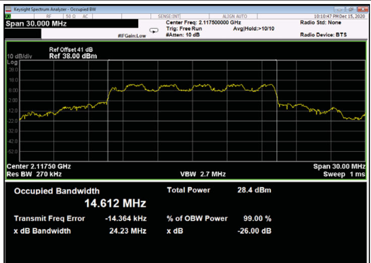
Figure 552: 16QAM 15MHz B.W.; 2117.5MHz, 15kHz - Output
