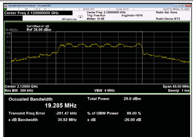
Figure 562: 16QAM 20MHz B.W.; 2120.0MHz, 30kHz - Output
