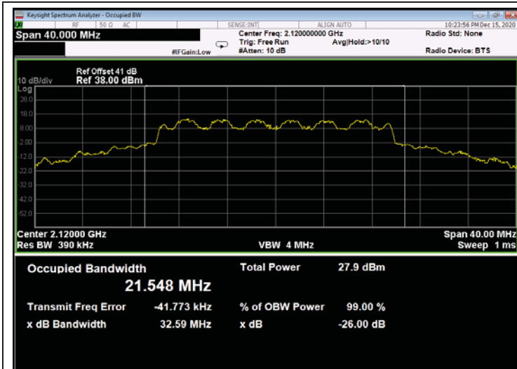
Figure 561: 16QAM 20MHz B.W.; 2120.0MHz, 15kHz - Output
