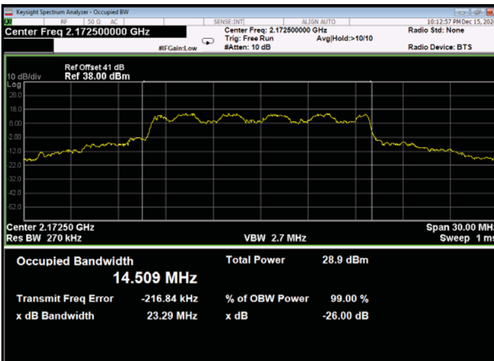
Figure 559: 16QAM 15MHz B.W.; 2172.5MHz, 30kHz - Output
