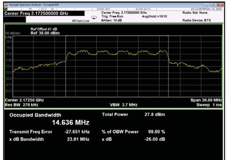
Figure 558: 16QAM 15MHz B.W.; 2172.5MHz, 15kHz - Output
