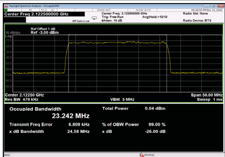
Figure 505: QPSK 25MHz B.W.; 2122.5MHz, 30kHz - Input
