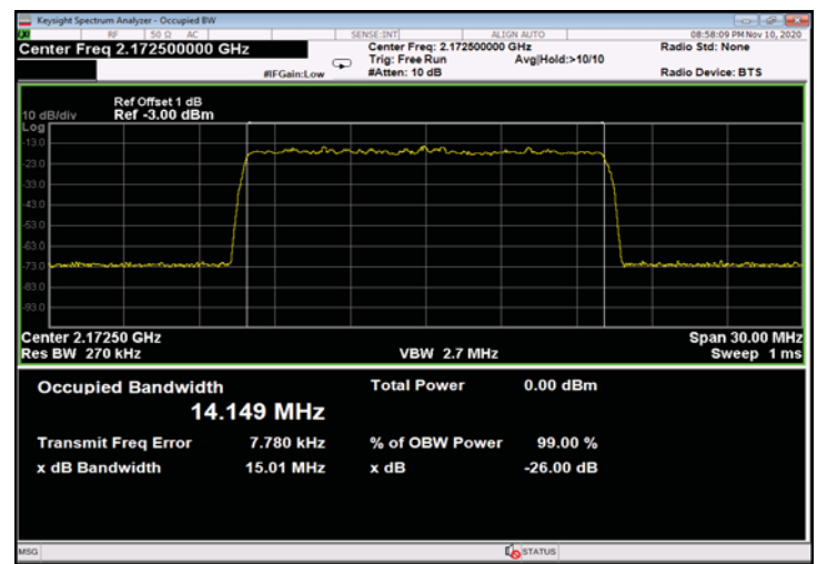
Figure 492: QPSK 15MHz B.W.; 2172.5MHz, 15kHz - Input
