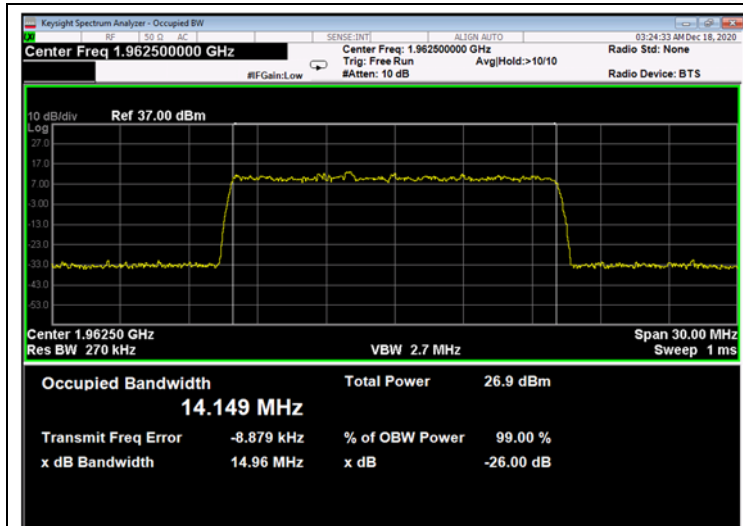
Figure 621: 64QAM 15MHz B.W.; 1962.5MHz, 15kHz - Output
