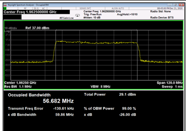
Figure 666: 64QAM 60MHz B.W.; 1962.5MHz, 60kHz - Output
