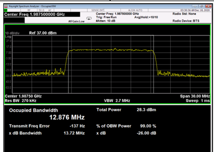
Figure 626: 64QAM 15MHz B.W.; 1987.5MHz, 60kHz - Output
