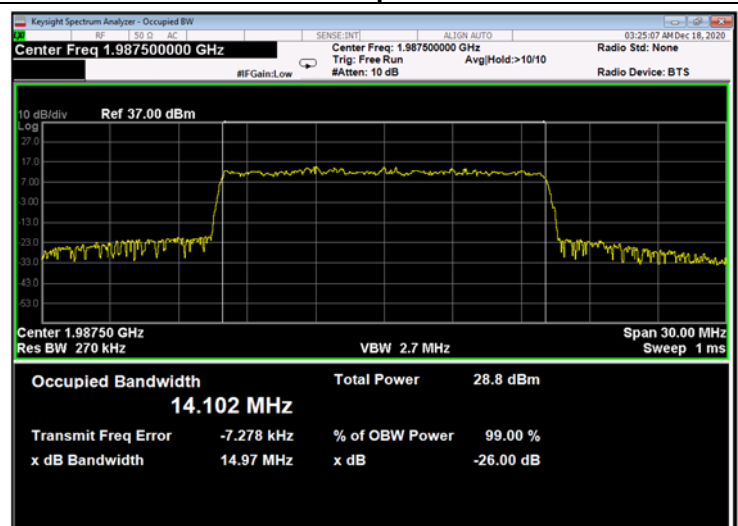
Figure 624: 64QAM 15MHz B.W.; 1987.5MHz, 15kHz - Output
