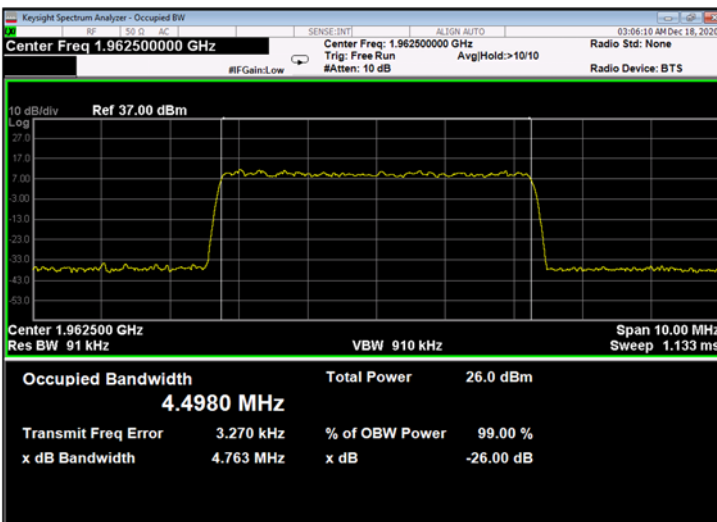
Figure 605: 64QAM 5MHz B.W.; 1962.5MHz, 15kHz - Output
