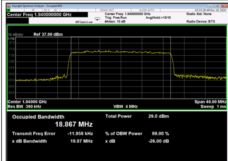
Figure 627: 64QAM 20MHz B.W.; 1940.0MHz, 15kHz - Output
