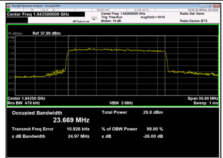
Figure 636: 64QAM 25MHz B.W.; 1942.5MHz, 15kHz - Output
