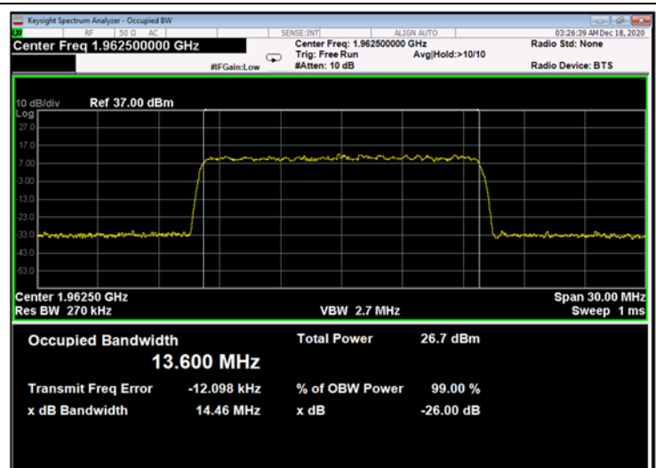
Figure 622: 64QAM 15MHz B.W.; 1962.5MHz, 30kHz - Output
