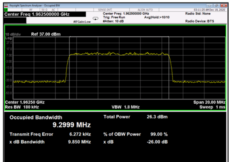
Figure 612: 64QAM 10MHz B.W.; 1962.5MHz, 15kHz - Output
