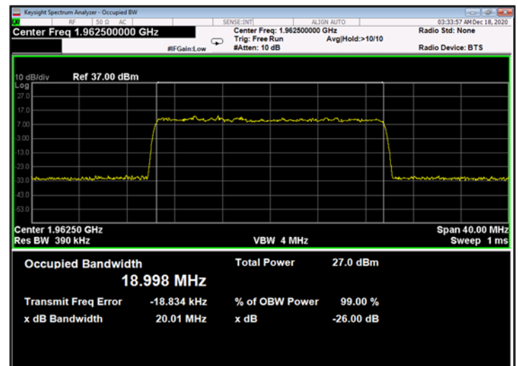
Figure 630: 64QAM 20MHz B.W.; 1962.5MHz, 15kHz - Output
