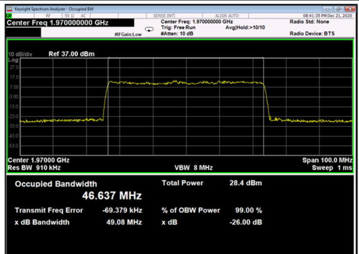
Figure 662: 64QAM 50MHz B.W.; 1970.0MHz, 60kHz - Output
