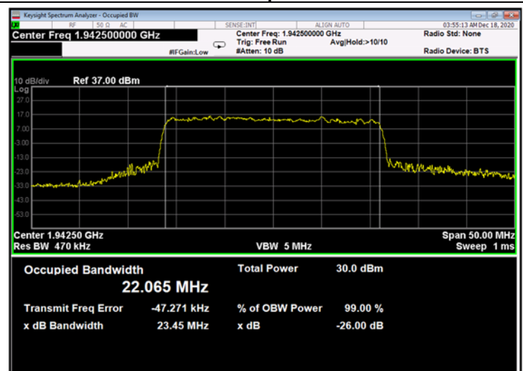
Figure 638: 64QAM 25MHz B.W.; 1942.5MHz, 60kHz - Output
