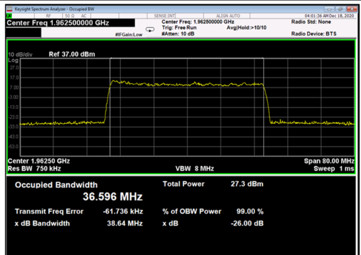
Figure 650: 64QAM 40MHz B.W.; 1962.5MHz, 60kHz - Output
