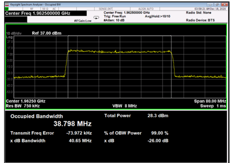
Figure 648: 64QAM 40MHz B.W.; 1962.5MHz, 15kHz - Output
