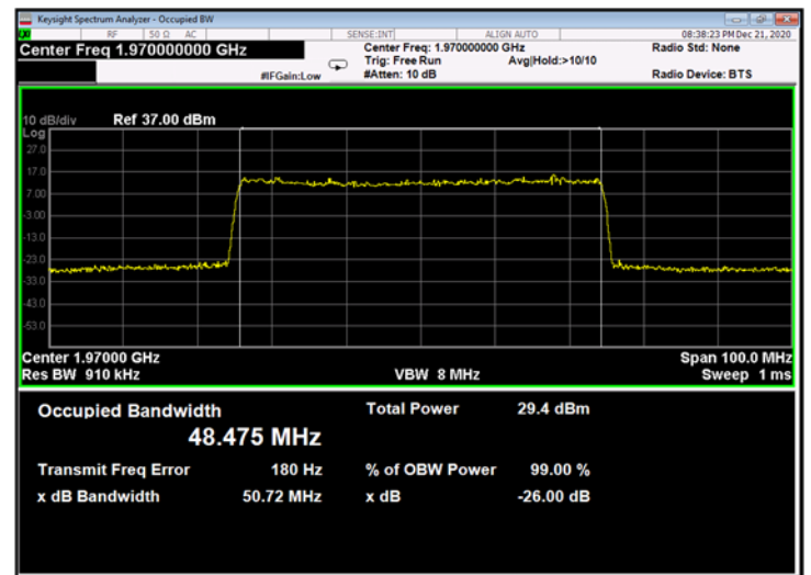
Figure 660: 64QAM 50MHz B.W.; 1970.0MHz, 15kHz - Output
