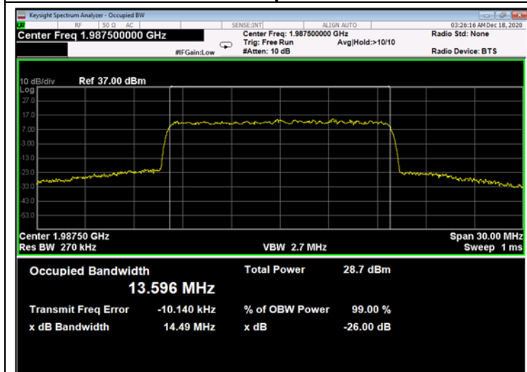
Figure 625: 64QAM 15MHz B.W.; 1987.5MHz, 30kHz - Output
