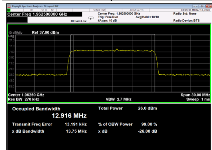
Figure 623: 64QAM 15MHz B.W.; 1962.5MHz, 60kHz - Output
