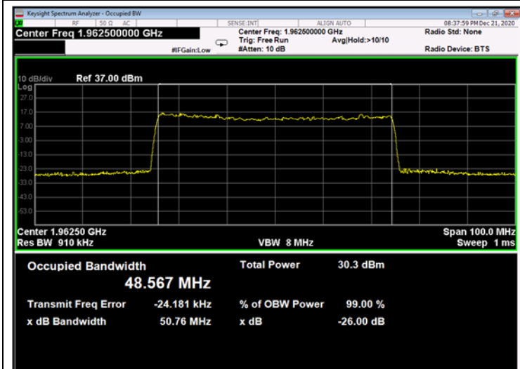
Figure 657: 64QAM 50MHz B.W.; 1962.5MHz, 15kHz - Output
