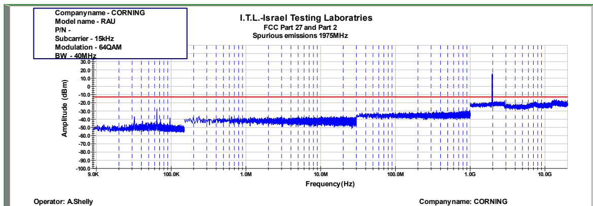
Figure 911: Spurious Emissions at Antenna Terminal 64QAM 40MHz B.W.; 1975.0MHz, 15kHz
