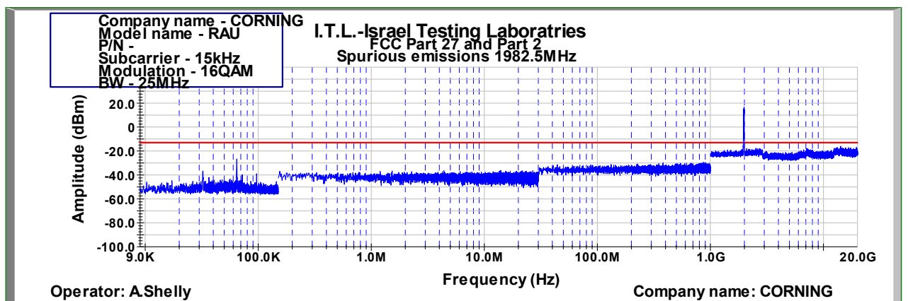
Figure 836: Spurious Emissions at Antenna Terminal 16QAM 25MHz B.W.; 1982.5MHz, 15kHz
