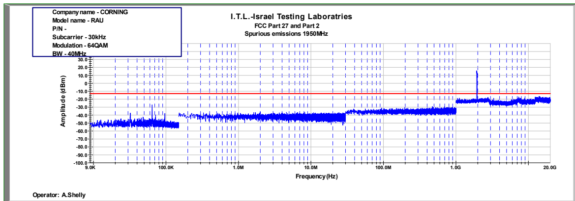
Figure 912: Spurious Emissions at Antenna Terminal 64QAM 40MHz B.W.; 1950.0MHz, 30kHz
