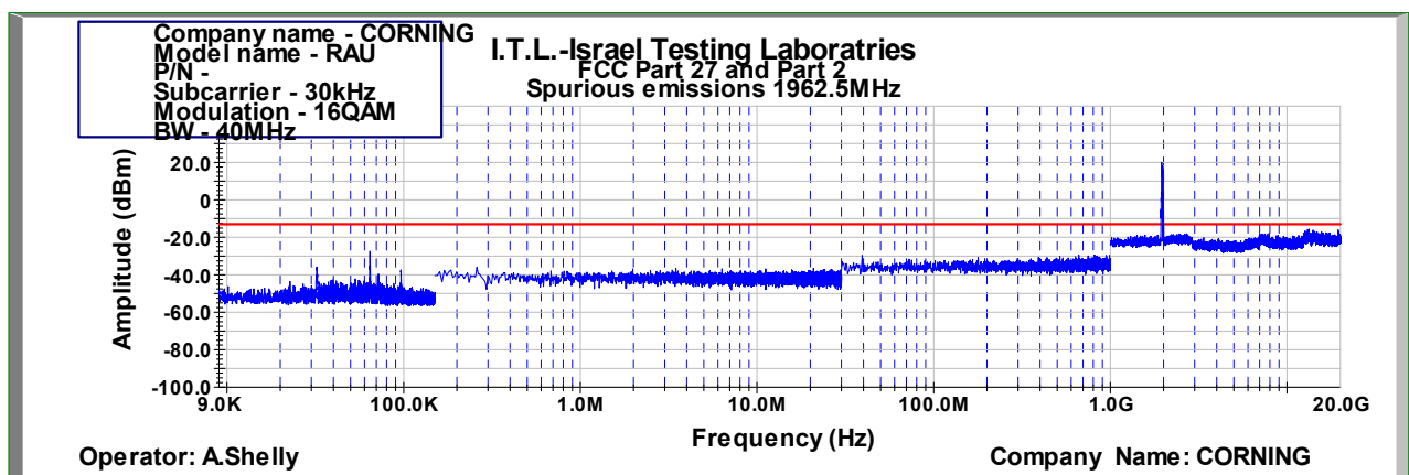
Figure 847: Spurious Emissions at Antenna Terminal 16QAM 40MHz B.W.; 1962.5MHz, 30kHz
