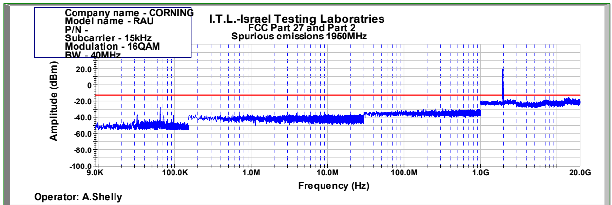
Figure 843: Spurious Emissions at Antenna Terminal 16QAM 40MHz B.W.; 1950.0MHz, 15kHz
