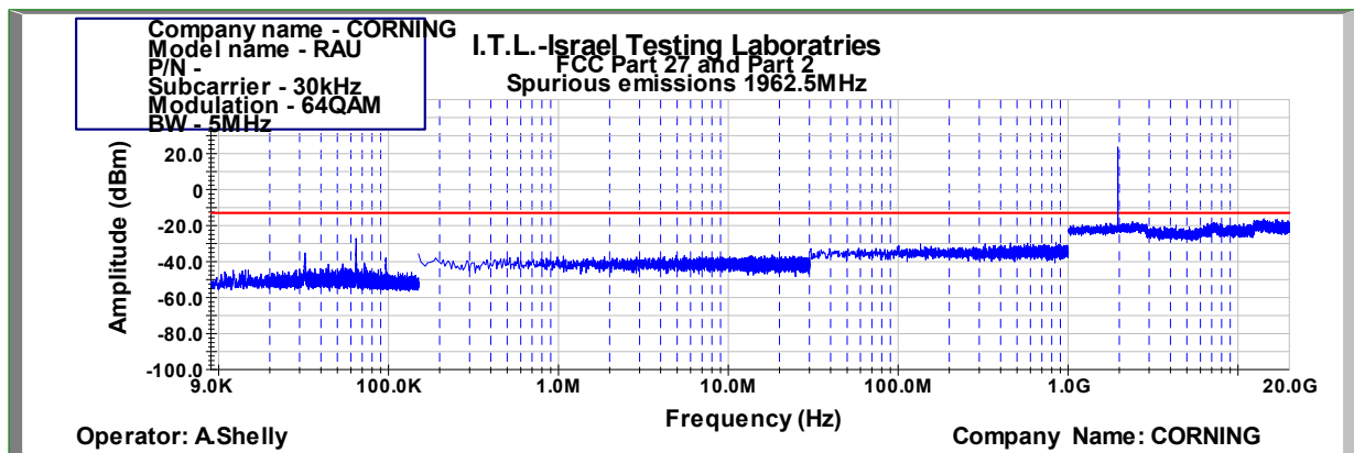
Figure 871: Spurious Emissions at Antenna Terminal 64QAM 5MHz B.W.; 1962.5MHz, 30kHz
