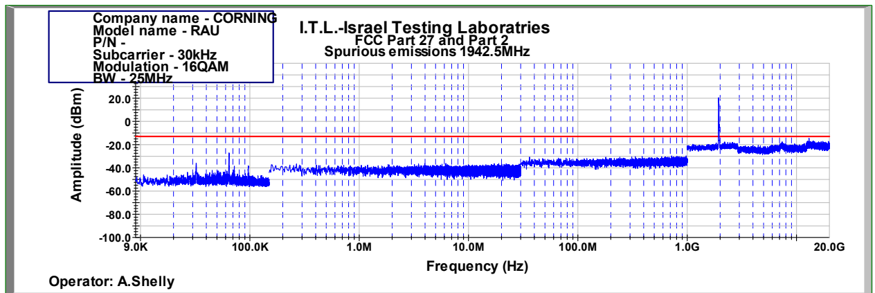
Figure 837: Spurious Emissions at Antenna Terminal 16QAM 25MHz B.W.; 1942.5MHz, 30kHz
