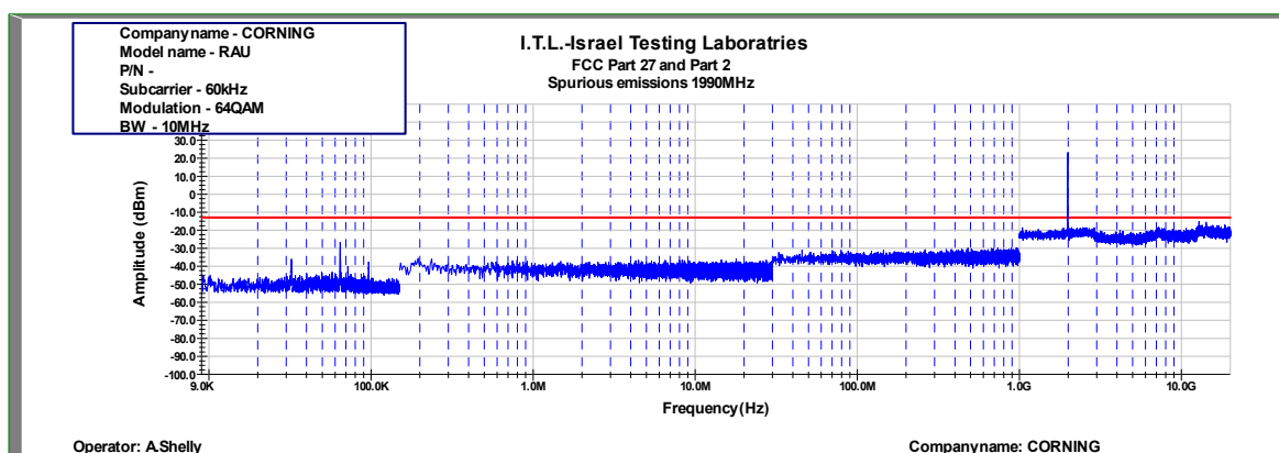
Figure 881: Spurious Emissions at Antenna Terminal 64QAM 10MHz B.W.; 1990.0MHz, 60kHz
