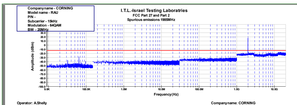
Figure 893: Spurious Emissions at Antenna Terminal 64QAM 20MHz B.W.; 1985.0MHz, 15kHz
