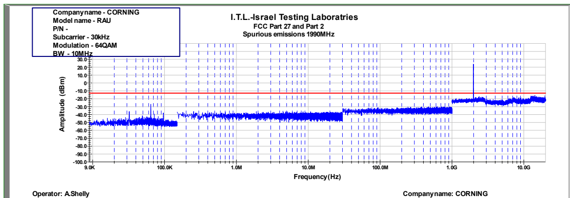
Figure 878: Spurious Emissions at Antenna Terminal 64QAM 10MHz B.W.; 1990.00MHz, 30kHz
