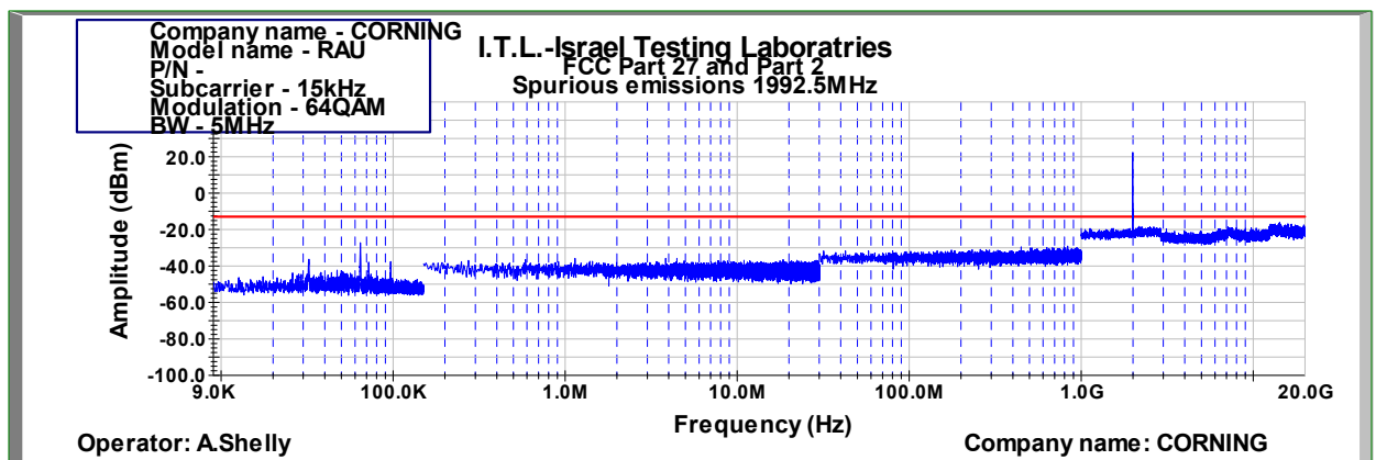
Figure 869: Spurious Emissions at Antenna Terminal 64QAM 5MHz B.W.; 1992.5MHz, 15kHz
