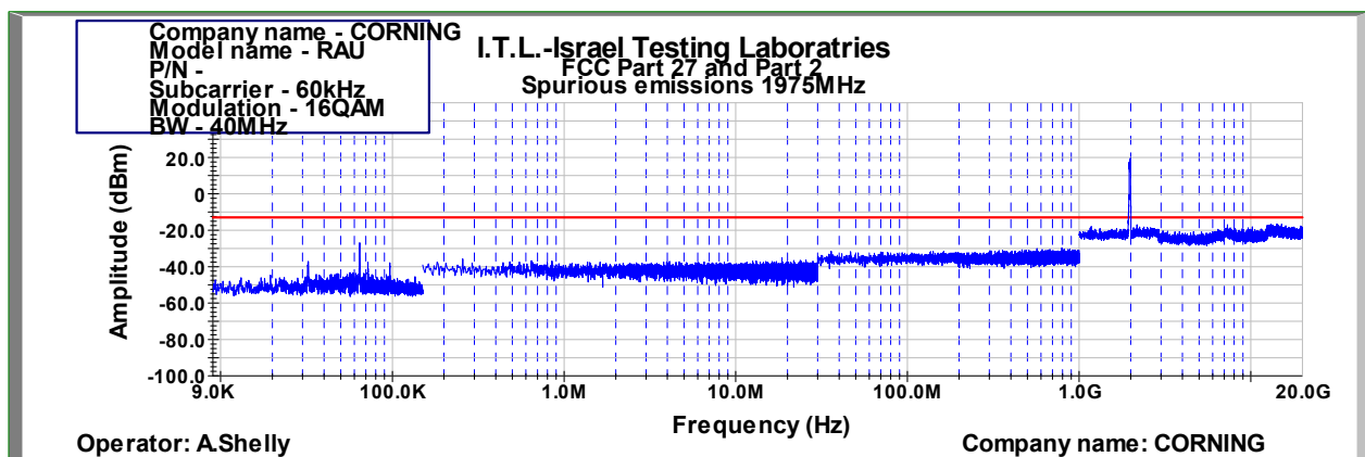
Figure 851: Spurious Emissions at Antenna Terminal 16QAM 40MHz B.W.; 1975.0MHz, 60kHz
