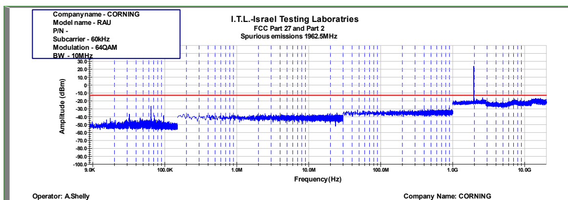
Figure 880: Spurious Emissions at Antenna Terminal 64QAM 10MHz B.W.; 1962.5MHz, 60kHz
