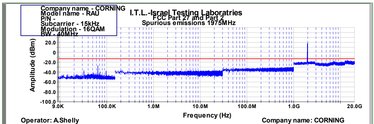
Figure 845: Spurious Emissions at Antenna Terminal 16QAM 40MHz B.W.; 1975.0MHz, 15kHz
