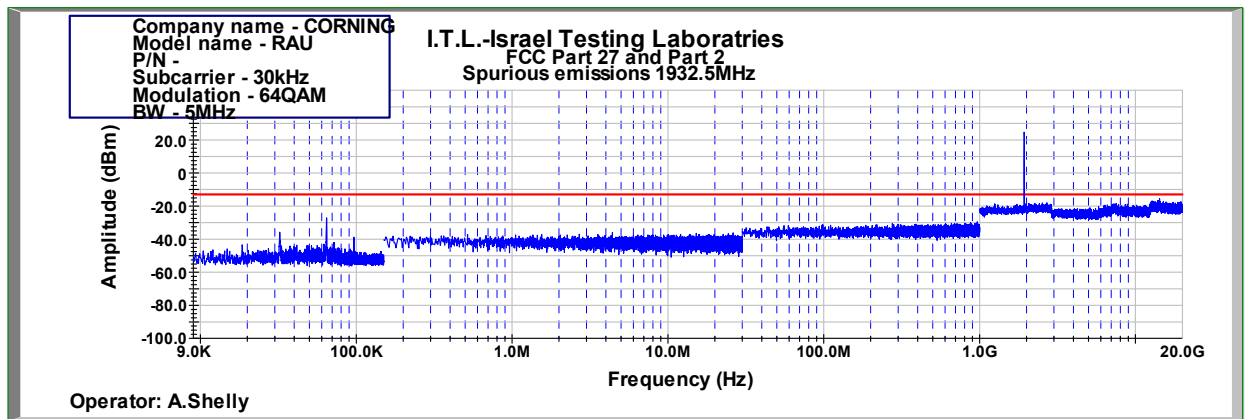
Figure 870: Spurious Emissions at Antenna Terminal 64QAM 5MHz B.W.; 1932.5MHz, 30kHz
