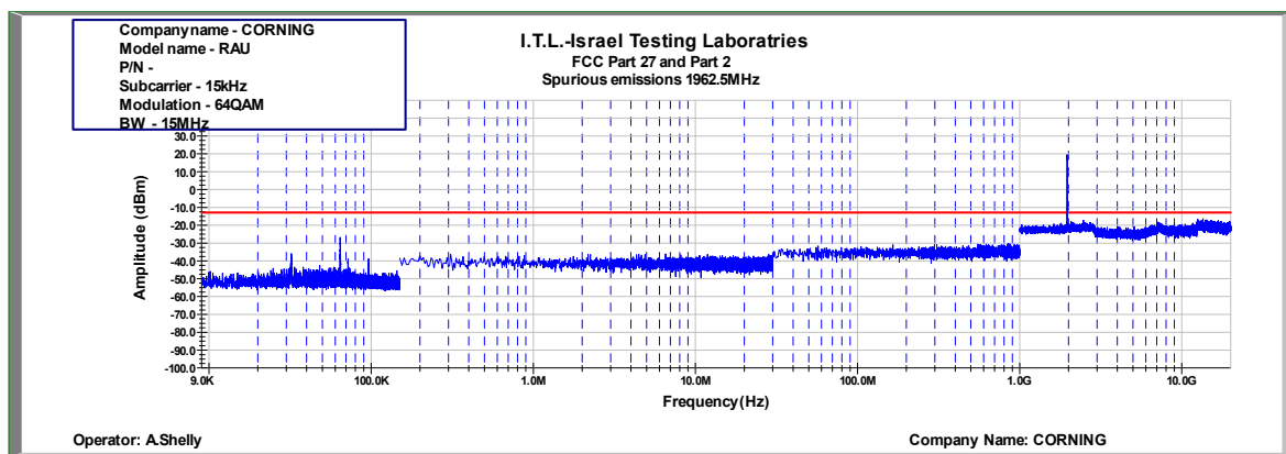
Figure 883: Spurious Emissions at Antenna Terminal 64QAM 15MHz B.W.; 1962.5MHz, 15kHz
