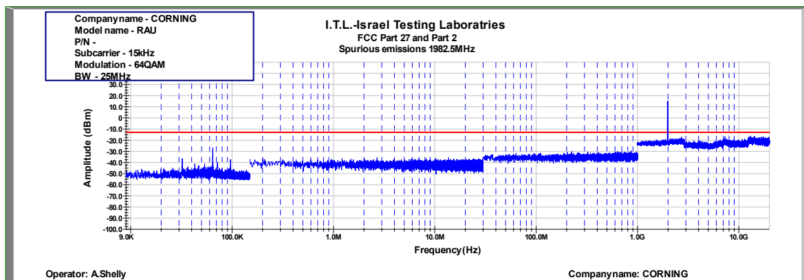
Figure 902: Spurious Emissions at Antenna Terminal 64QAM 25MHz B.W.; 1982.5MHz, 15kHz
