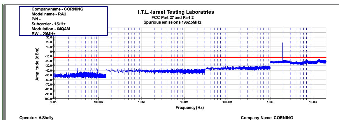
Figure 892: Spurious Emissions at Antenna Terminal 64QAM 20MHz B.W.; 1962.5MHz, 15kHz
