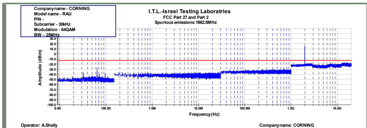
Figure 905: Spurious Emissions at Antenna Terminal 64QAM 25MHz B.W.; 1982.5MHz, 30kHz
