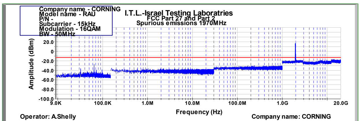
Figure 854: Spurious Emissions at Antenna Terminal 16QAM 50MHz B.W.; 1970.0MHz, 15kHz
