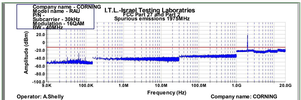
Figure 848: Spurious Emissions at Antenna Terminal 16QAM 40MHz B.W.; 1975.0MHz, 30kHz
