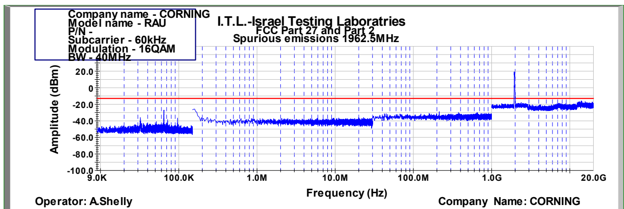
Figure 850: Spurious Emissions at Antenna Terminal 16QAM 40MHz B.W.; 1962.5MHz, 60kHz
