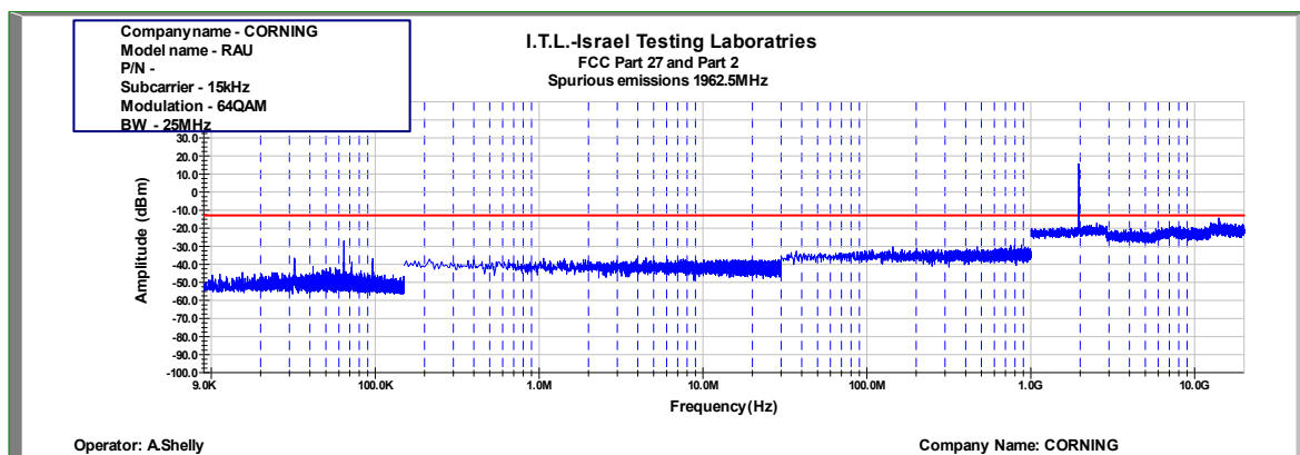
Figure 901: Spurious Emissions at Antenna Terminal 64QAM 25MHz B.W.; 1962.5MHz, 15kHz
