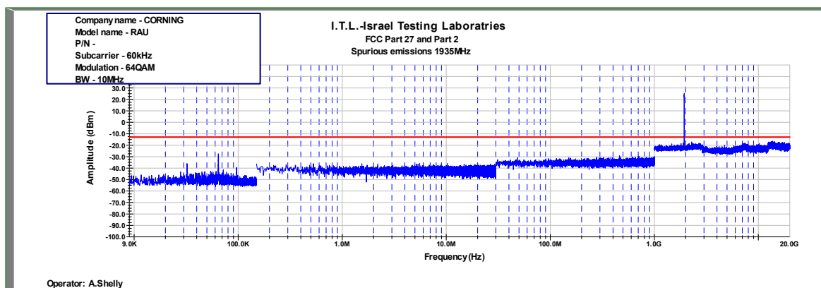
Figure 879: Spurious Emissions at Antenna Terminal 64QAM 10MHz B.W.; 1935.0MHz, 60kHz
