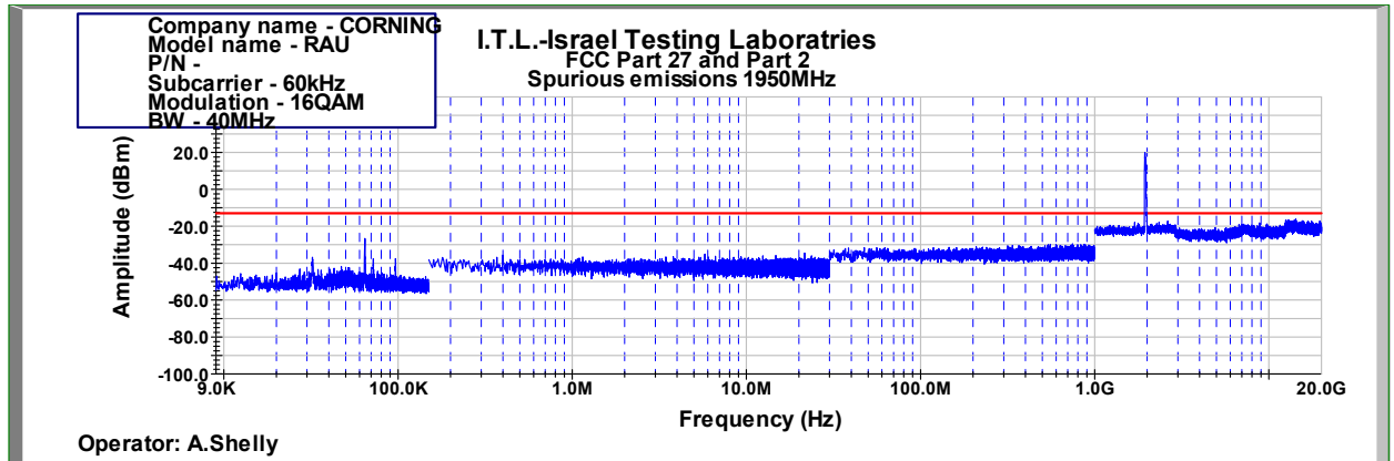
Figure 849: Spurious Emissions at Antenna Terminal 16QAM 40MHz B.W.; 1950.0MHz, 60kHz
