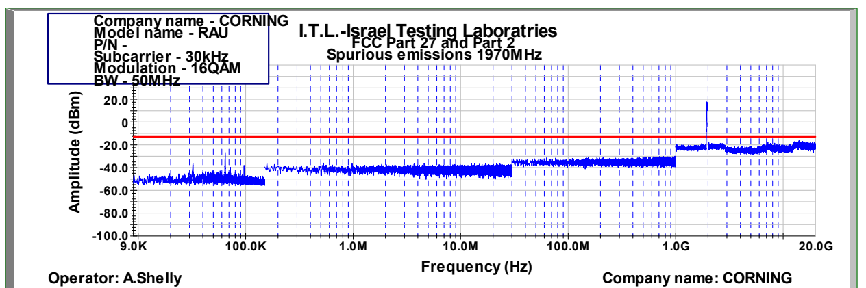
Figure 857: Spurious Emissions at Antenna Terminal 16QAM 50MHz B.W.; 1970.0MHz, 30kHz
