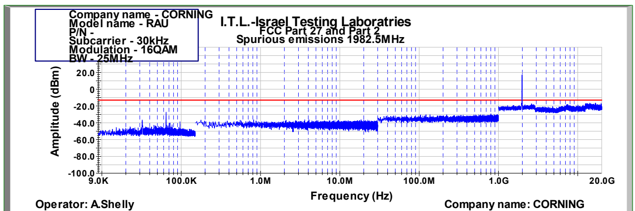
Figure 839: Spurious Emissions at Antenna Terminal 16QAM 25MHz B.W.; 1982.5MHz, 30kHz
