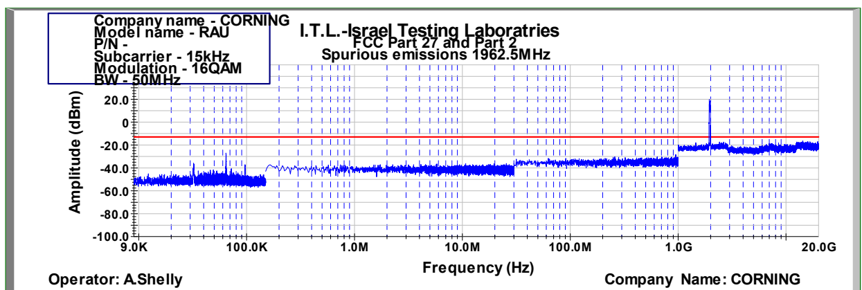
Figure 853: Spurious Emissions at Antenna Terminal 16QAM 50MHz B.W.; 1962.5MHz, 15kHz
