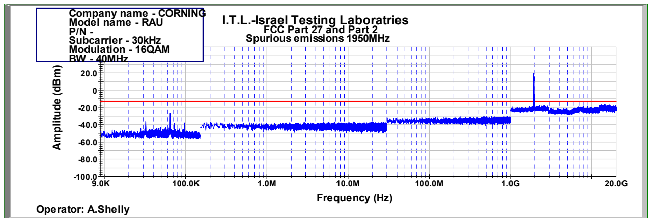
Figure 846: Spurious Emissions at Antenna Terminal 16QAM 40MHz B.W.; 1950.0MHz, 30kHz
