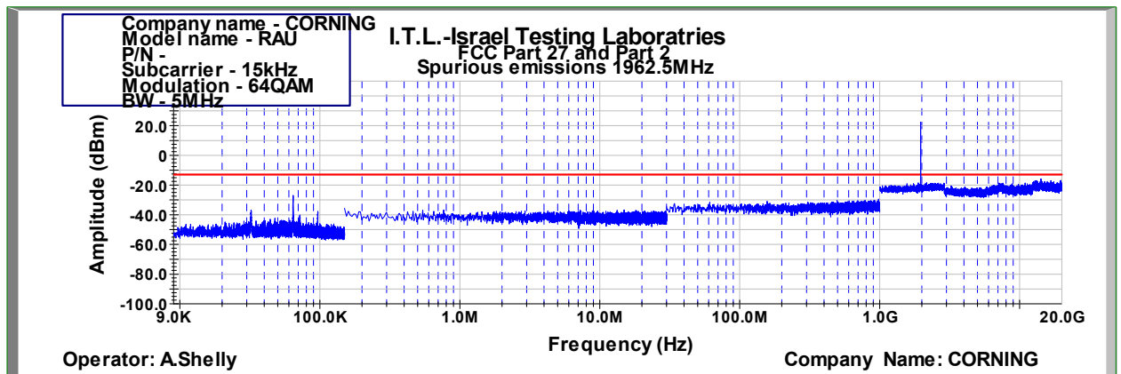
Figure 868: Spurious Emissions at Antenna Terminal 64QAM 5MHz B.W.; 1962.5MHz, 15kHz
