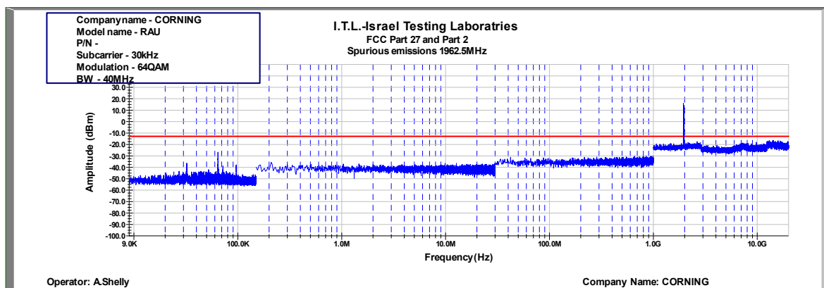
Figure 913: Spurious Emissions at Antenna Terminal 64QAM 40MHz B.W.; 1962.5MHz, 30kHz
