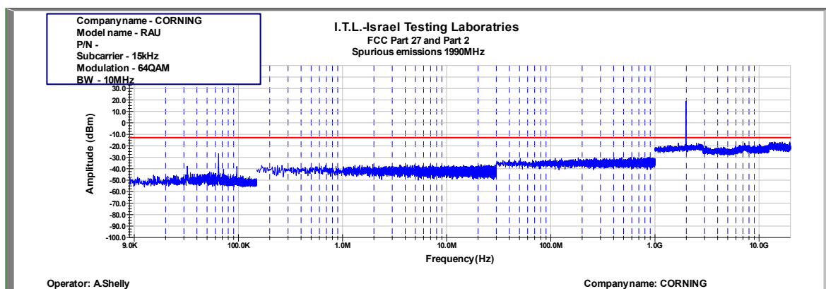
Figure 875: Spurious Emissions at Antenna Terminal 64QAM 10MHz B.W.; 1990.00MHz, 15kHz
