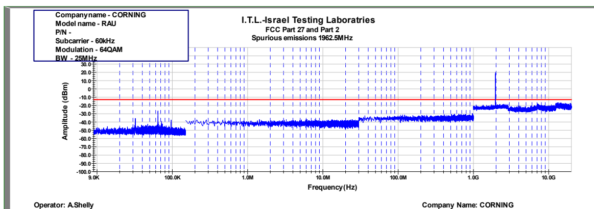
Figure 907: Spurious Emissions at Antenna Terminal 64QAM 25MHz B.W.; 1962.5MHz, 60kHz
