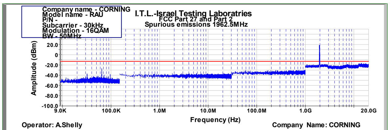
Figure 856: Spurious Emissions at Antenna Terminal 16QAM 50MHz B.W.; 1962.5MHz, 30kHz
