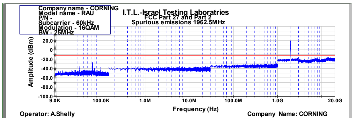
Figure 841: Spurious Emissions at Antenna Terminal 16QAM 25MHz B.W.; 1962.5MHz, 60kHz
