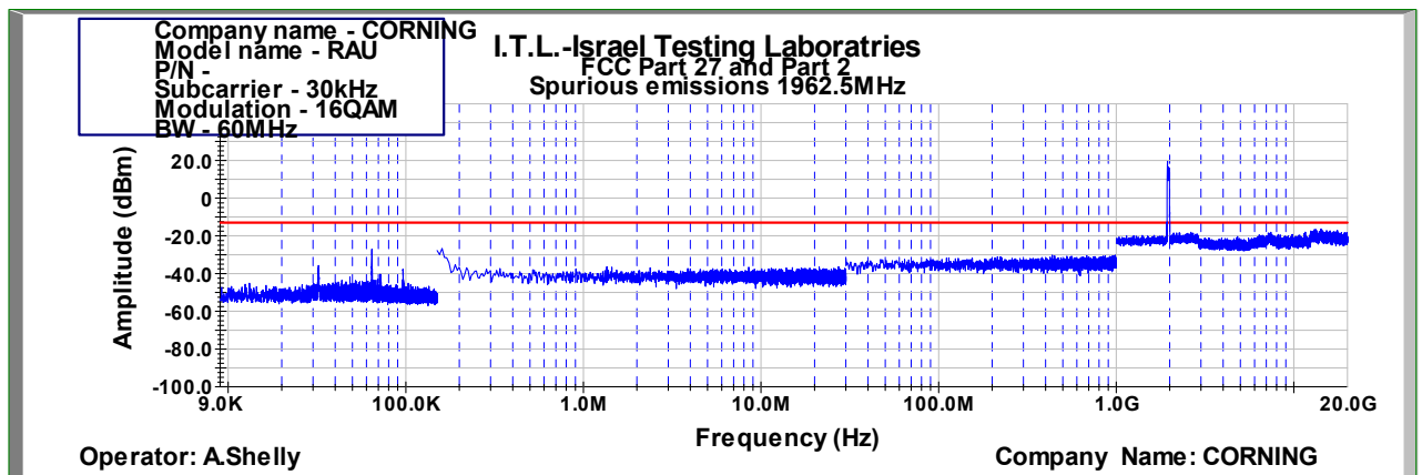
Figure 862: Spurious Emissions at Antenna Terminal 16QAM 60MHz B.W.; 1962.5MHz, 30kHz
