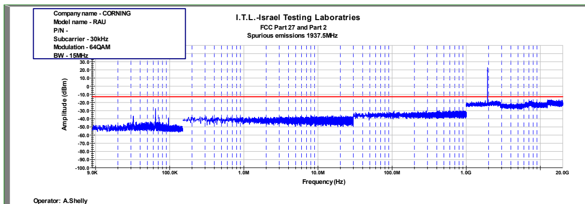
Figure 885: Spurious Emissions at Antenna Terminal 64QAM 15MHz B.W.; 1937.5MHz, 30kHz
