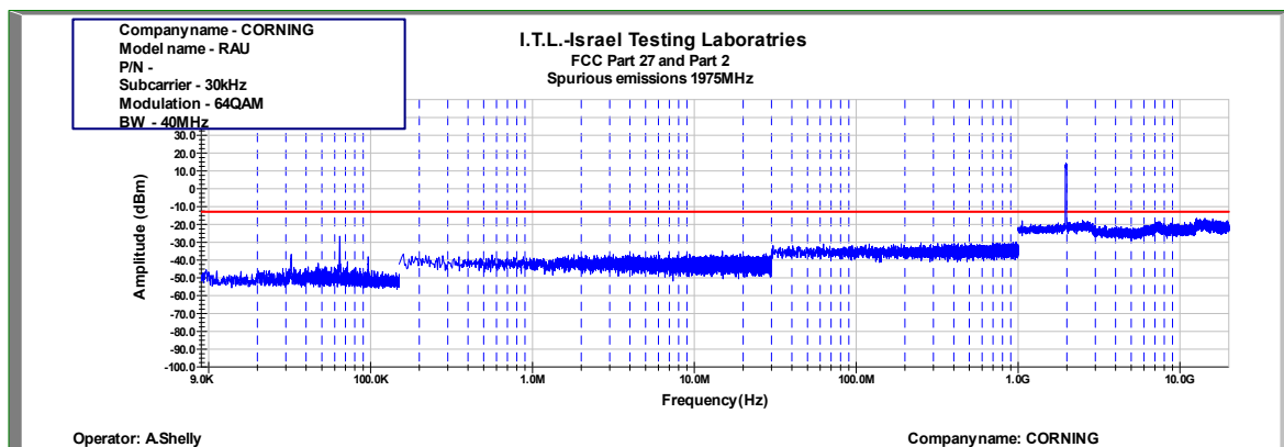
Figure 914: Spurious Emissions at Antenna Terminal 64QAM 40MHz B.W.; 1975.0MHz, 30kHz
