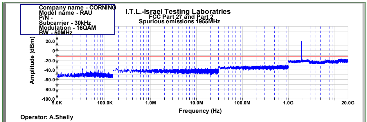
Figure 855: Spurious Emissions at Antenna Terminal 16QAM 50MHz B.W.; 1955.0MHz, 30kHz
