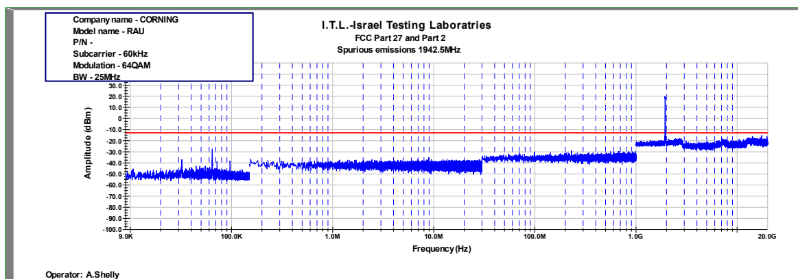
Figure 906: Spurious Emissions at Antenna Terminal 64QAM 25MHz B.W.; 1942.5MHz, 60kHz
