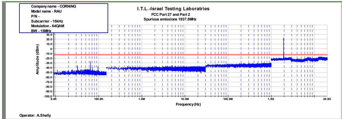
Figure 882: Spurious Emissions at Antenna Terminal 64QAM 15MHz B.W.; 1937.5MHz, 15kHz
