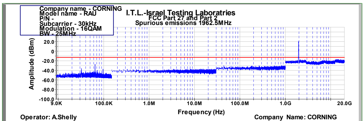
Figure 838: Spurious Emissions at Antenna Terminal 16QAM 25MHz B.W.; 1962.5MHz, 30kHz
