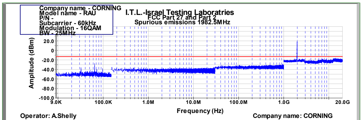
Figure 842: Spurious Emissions at Antenna Terminal 16QAM 25MHz B.W.; 1982.5MHz, 60kHz
