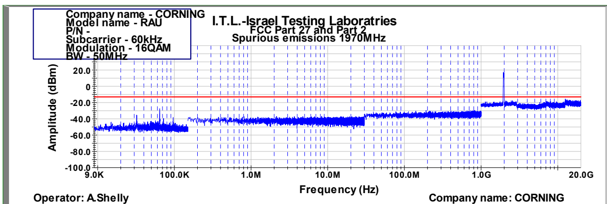
Figure 860: Spurious Emissions at Antenna Terminal 16QAM 50MHz B.W.; 1970.0MHz, 60kHz
