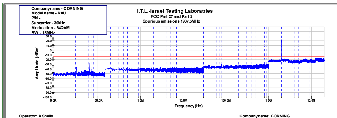
Figure 887: Spurious Emissions at Antenna Terminal 64QAM 15MHz B.W.; 1987.5MHz, 30kHz
