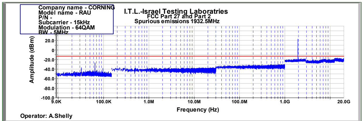
Figure 867: Spurious Emissions at Antenna Terminal 64QAM 5MHz B.W.; 1932.5MHz, 15kHz
