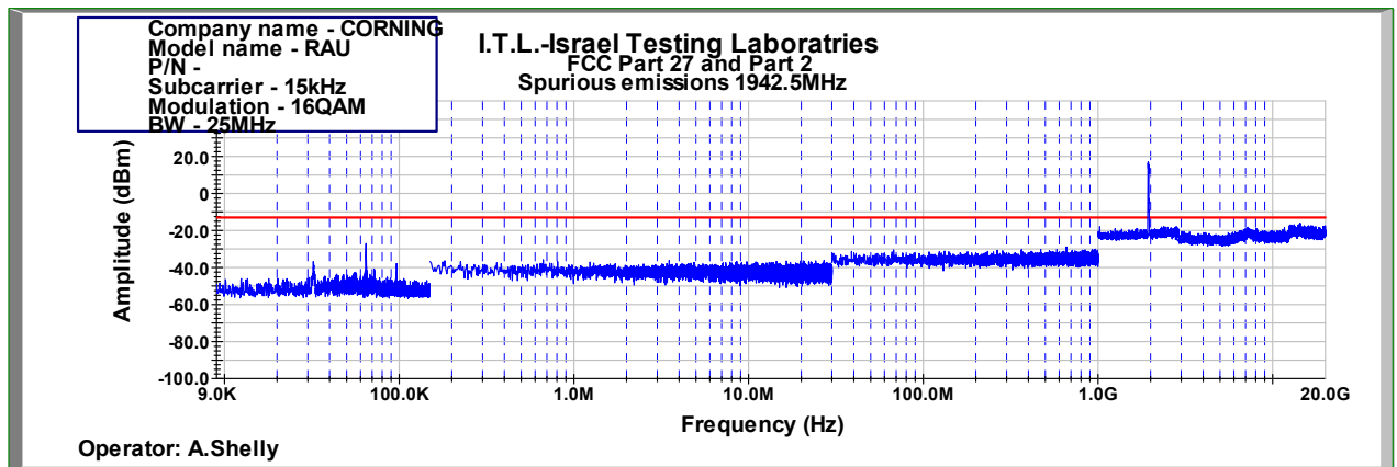
Figure 834: Spurious Emissions at Antenna Terminal 16QAM 25MHz B.W.; 1942.5MHz, 15kHz
