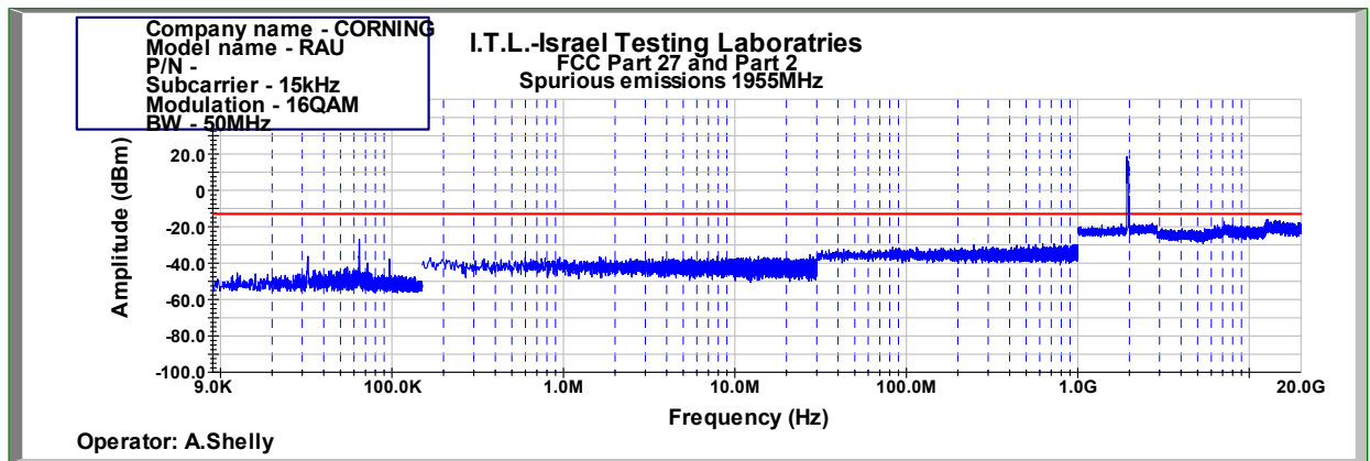
Figure 852: Spurious Emissions at Antenna Terminal 16QAM 50MHz B.W.; 1955.0MHz, 15kHz
