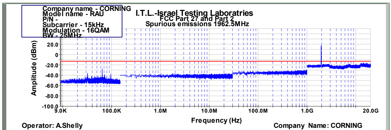
Figure 835: Spurious Emissions at Antenna Terminal 16QAM 25MHz B.W.; 1962.5MHz, 15kHz
