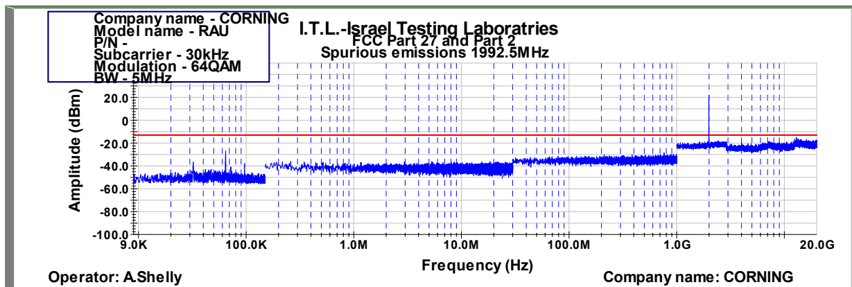
Figure 872: Spurious Emissions at Antenna Terminal 64QAM 5MHz B.W.; 1992.5MHz, 30kHz
