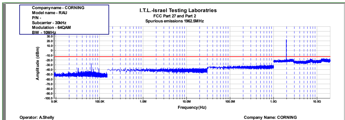
Figure 877: Spurious Emissions at Antenna Terminal 64QAM 10MHz B.W.; 1962.5MHz, 30kHz
