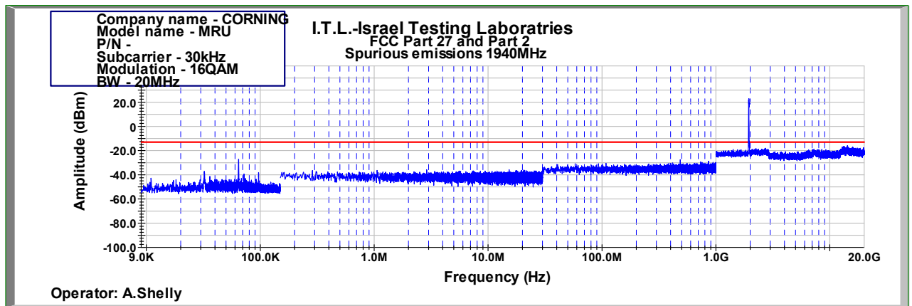
Figure 828: Spurious Emissions at Antenna Terminal 16QAM 20MHz B.W.; 1940.0MHz, 30kHz
