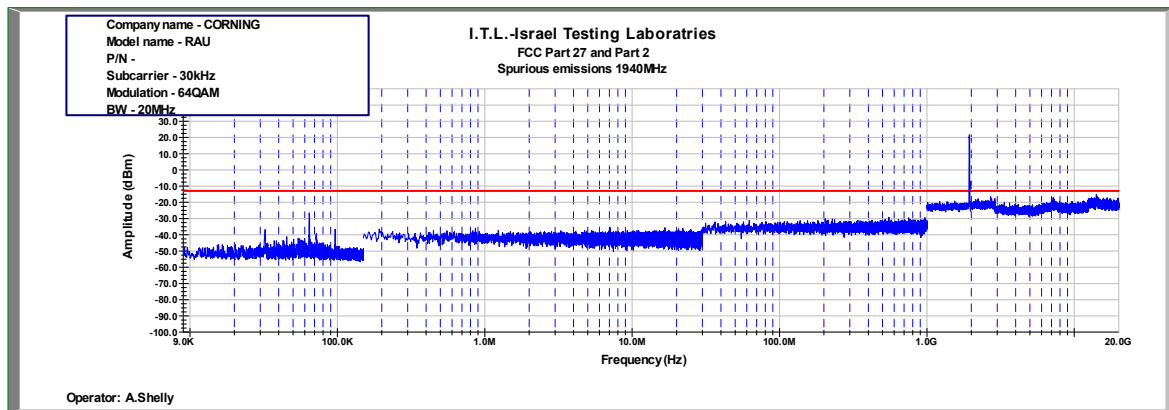
Figure 894: Spurious Emissions at Antenna Terminal 64QAM 20MHz B.W.; 1940.0MHz, 30kHz
