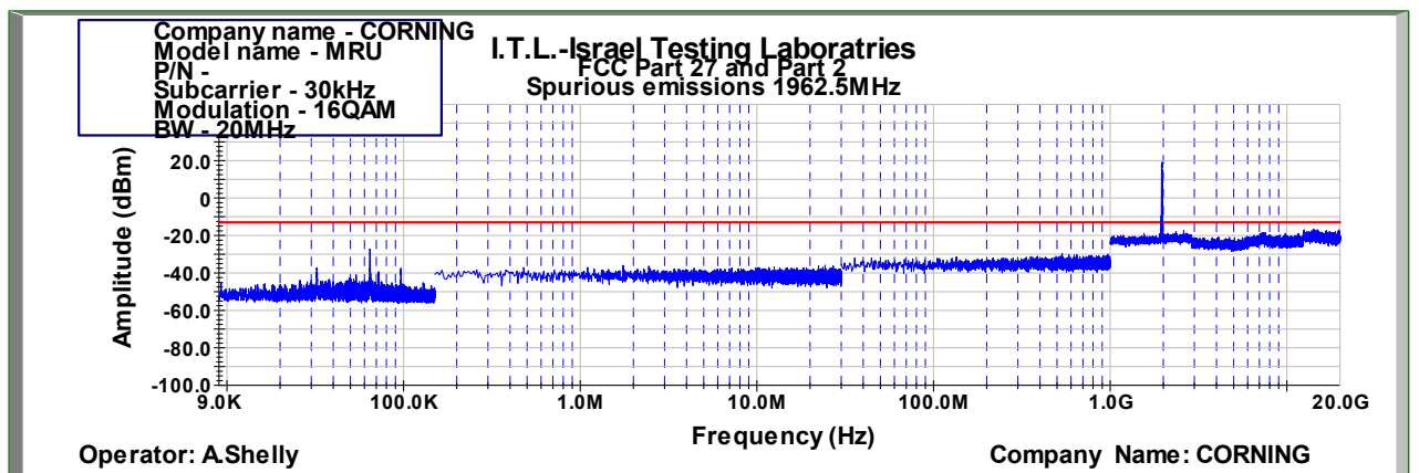
Figure 829: Spurious Emissions at Antenna Terminal 16QAM 20MHz B.W.; 1962.5MHz, 30kHz
