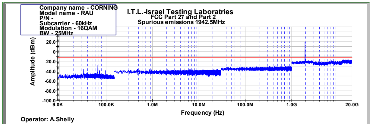
Figure 840: Spurious Emissions at Antenna Terminal 16QAM 25MHz B.W.; 1942.5MHz, 60kHz
