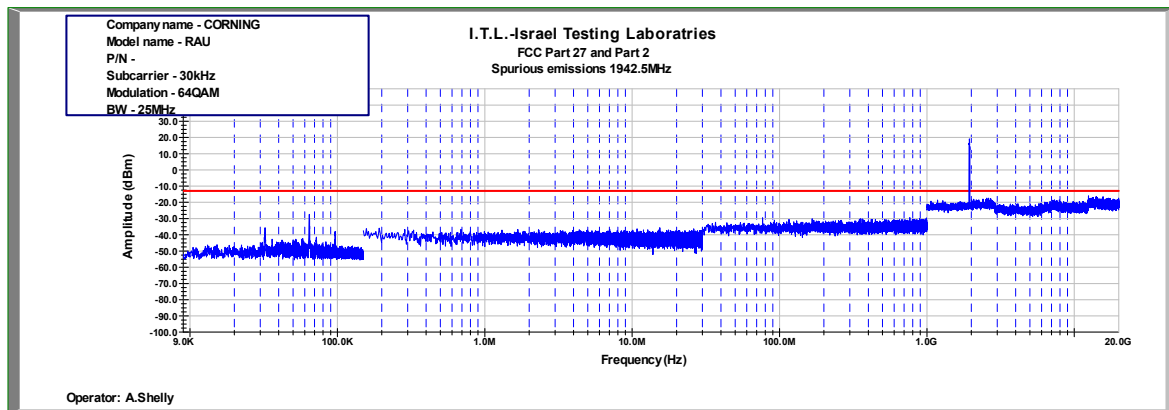
Figure 903: Spurious Emissions at Antenna Terminal 64QAM 25MHz B.W.; 1942.5MHz, 30kHz
