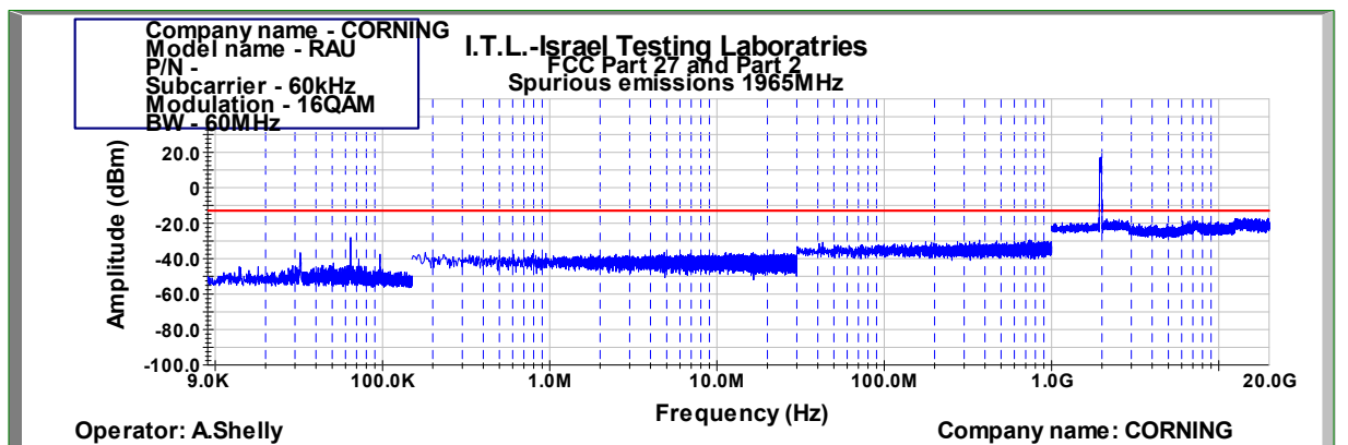
Figure 866: Spurious Emissions at Antenna Terminal 16QAM 60MHz B.W.; 1965.0MHz, 60kHz
