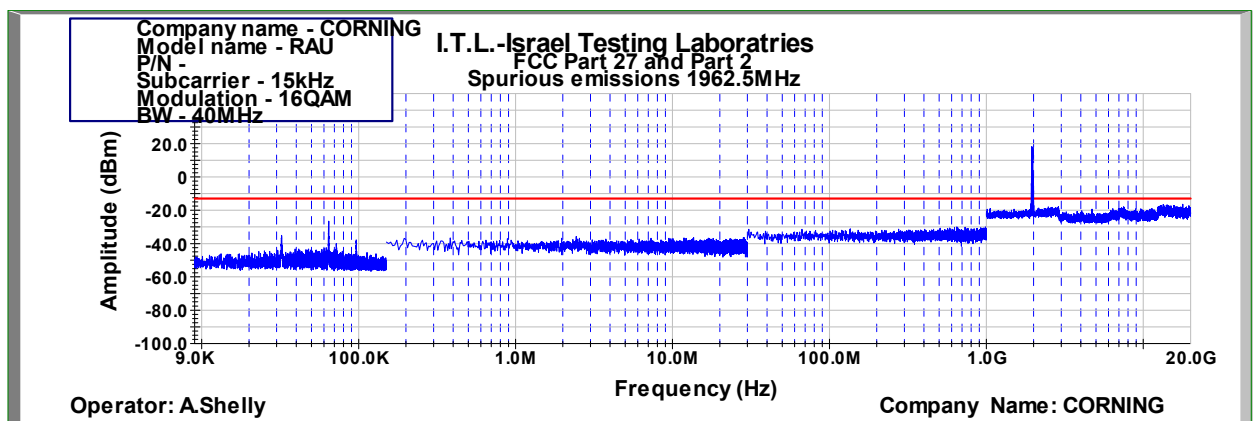
Figure 844: Spurious Emissions at Antenna Terminal 16QAM 40MHz B.W.; 1962.5MHz, 15kHz
