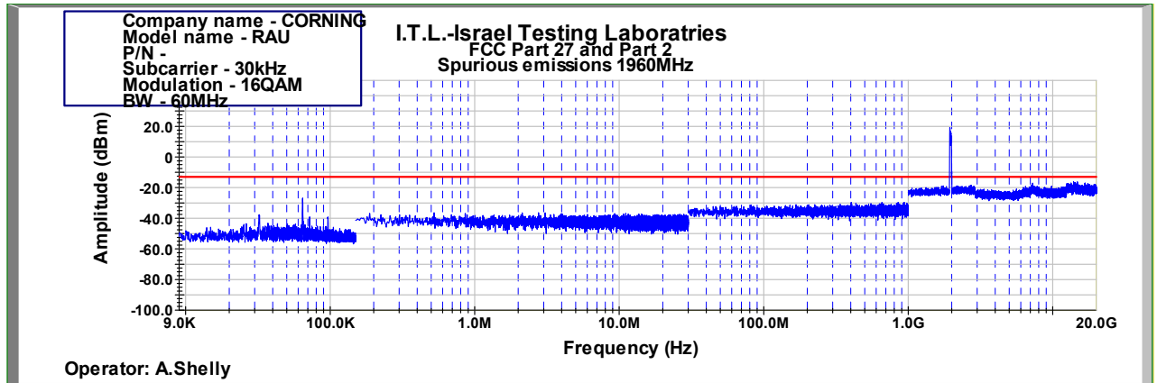
Figure 861: Spurious Emissions at Antenna Terminal 16QAM 60MHz B.W.; 1960.0MHz, 30kHz
