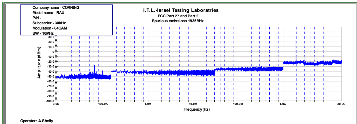
Figure 876: Spurious Emissions at Antenna Terminal 64QAM 10MHz B.W.; 1935.00MHz, 30kHz
