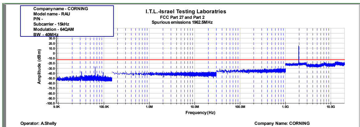
Figure 910: Spurious Emissions at Antenna Terminal 64QAM 40MHz B.W.; 1962.5MHz, 15kHz
