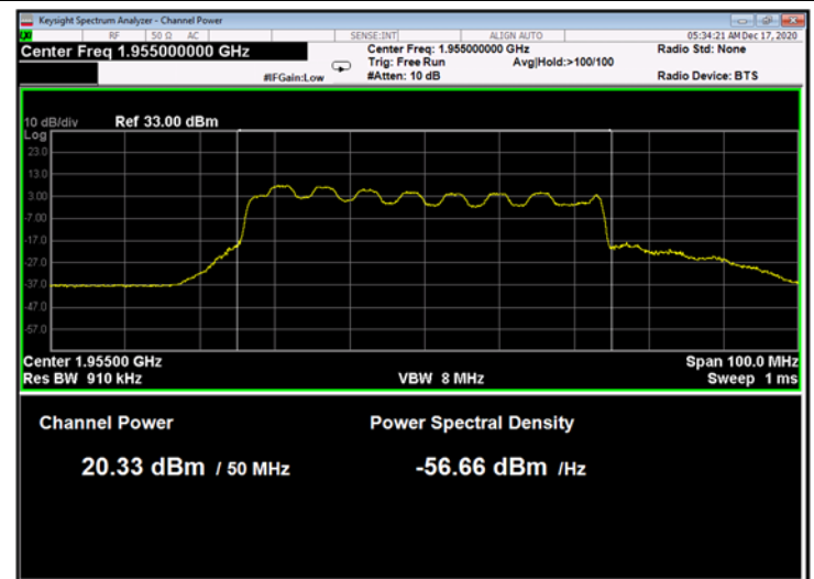
Figure 62: 16QAM 50MHz B.W.; 1955.0MHz, 60kHz
