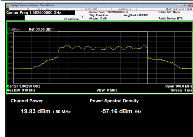
Figure 63: 16QAM 50MHz B.W.; 1962.5MHz, 15kHz
