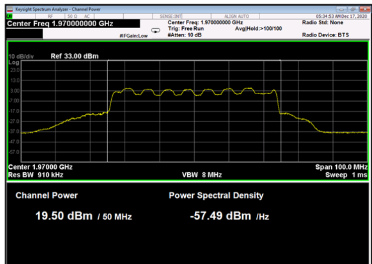
Figure 68: 16QAM 50MHz B.W.; 1970.0MHz, 60kHz
