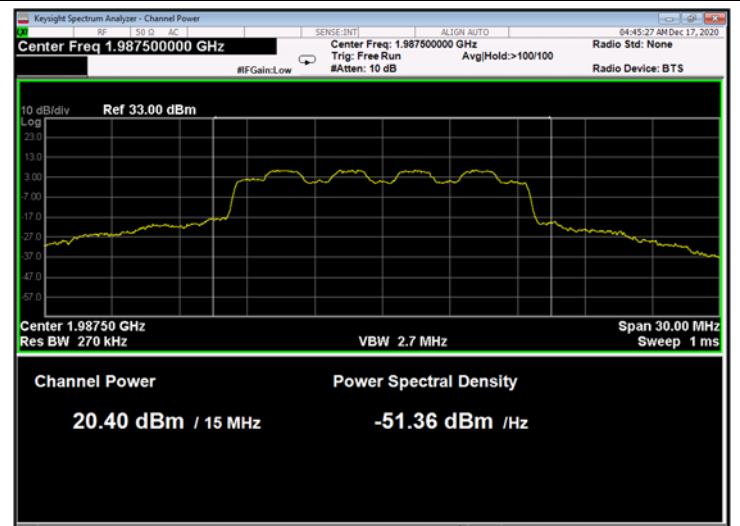
Figure 32: 16QAM 15MHz B.W.; 1987.5MHz, 60kHz
