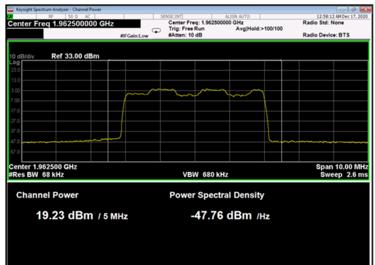
Figure 12: 16QAM 5MHz B.W.; 1962.5MHz, 30kHz
