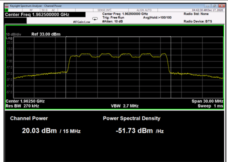
Figure 28: 16QAM 15MHz B.W.; 1962.5MHz, 30kHz
