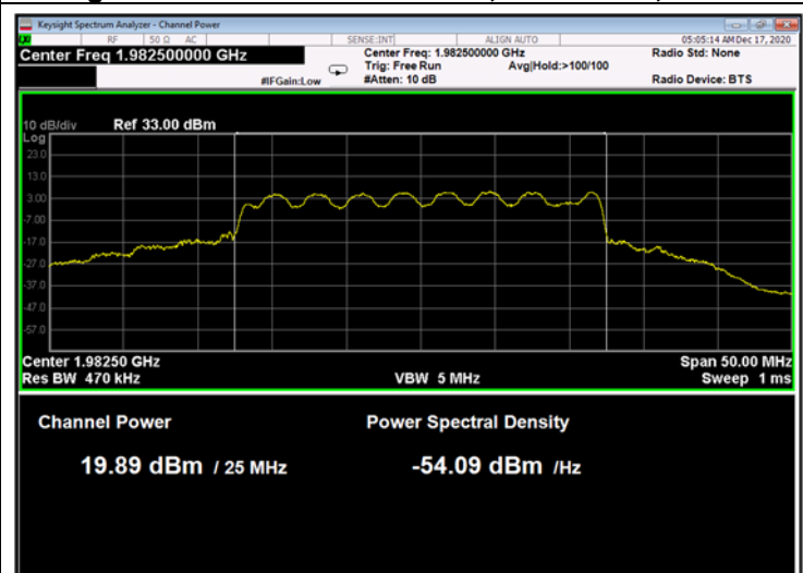
Figure 48: 16QAM 25MHz B.W.; 1982.5MHz, 15kHz
