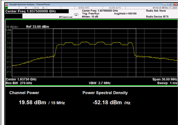
Figure 25: 16QAM 15MHz B.W.; 1937.5MHz, 30kHz
