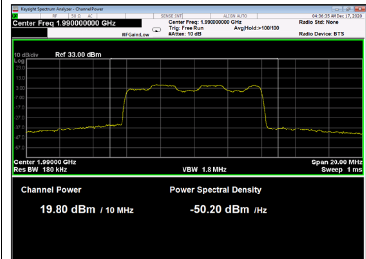
Figure 23: 16QAM 10MHz B.W.; 1990.0MHz, 60kHz
