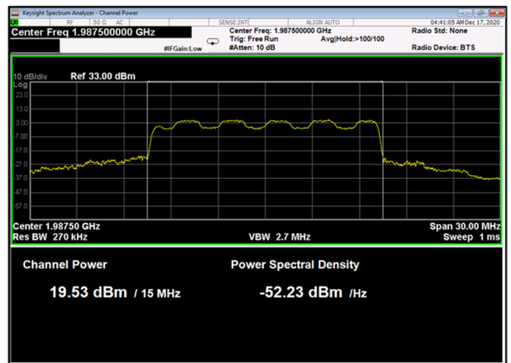
Figure 30: 16QAM 15MHz B.W.; 1987.5MHz, 15kHz
