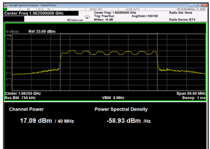
Figure 54: 16QAM 40MHz B.W.; 1962.5MHz, 15kHz
