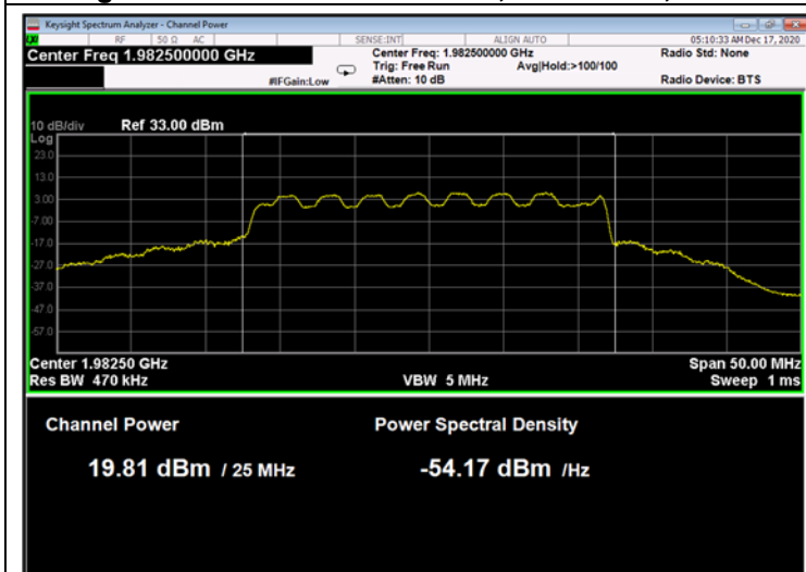
Figure 49: 16QAM 25MHz B.W.; 1982.5MHz, 30kHz
