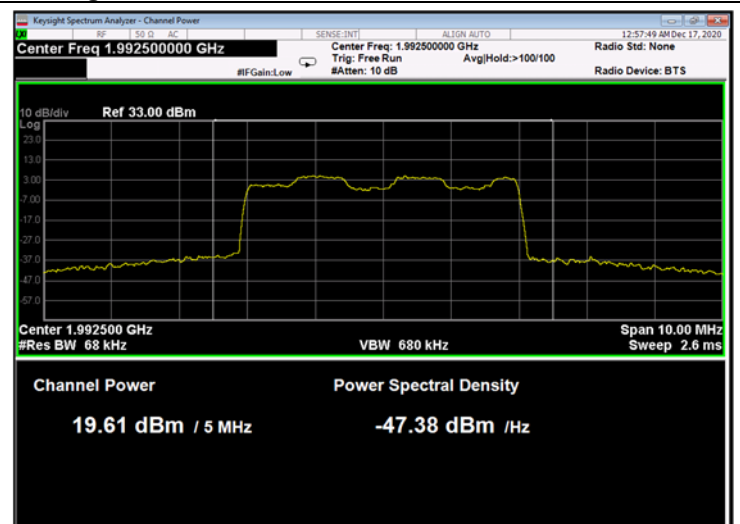
Figure 14: 16QAM 5MHz C.S.; 1992.5MHz, 30kHz
