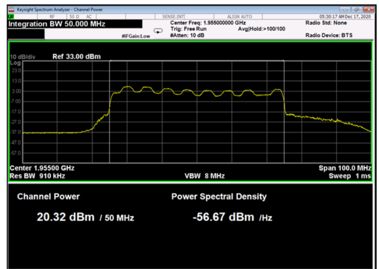
Figure 60: 16QAM 50MHz B.W.; 1955.0MHz, 15kHz
