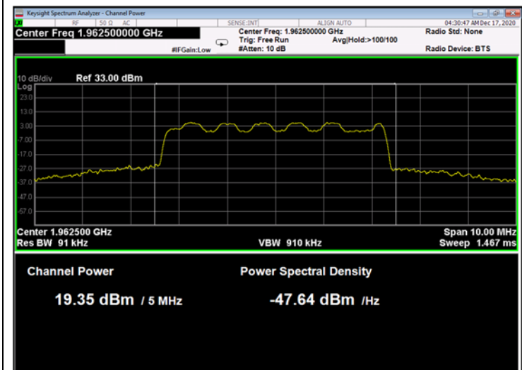
Figure 11: 16QAM 5MHz B.W.; 1962.5MHz, 15kHz
