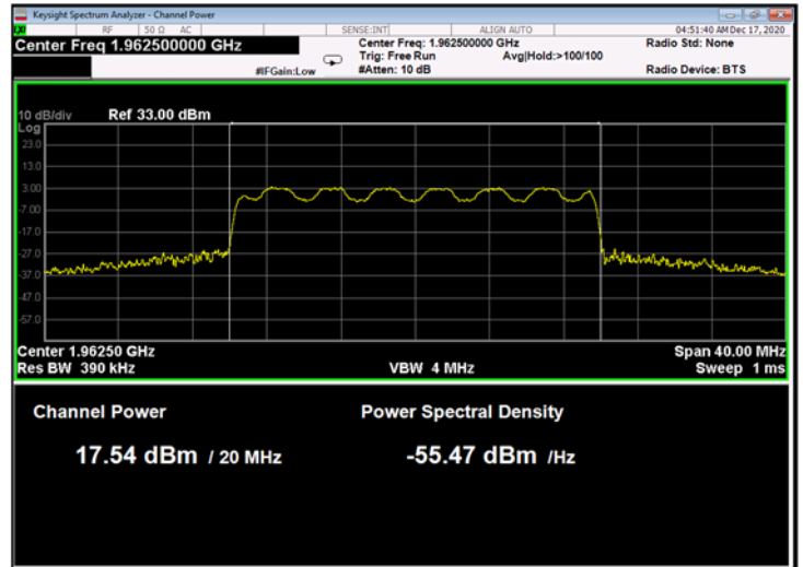
Figure 36: 16QAM 20MHz B.W.; 1962.5MHz, 15kHz
