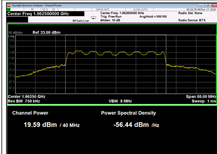
Figure 55: 16QAM 40MHz B.W.; 1962.5MHz, 30kHz
