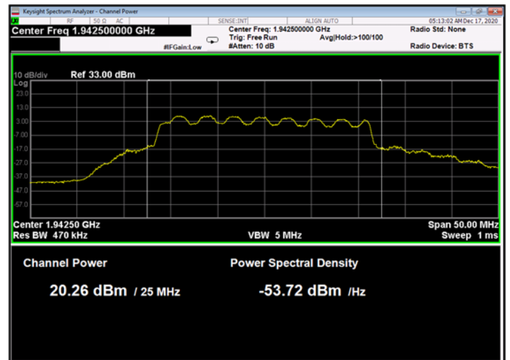
Figure 44: 16QAM 25MHz B.W.; 1942.5MHz, 60kHz
