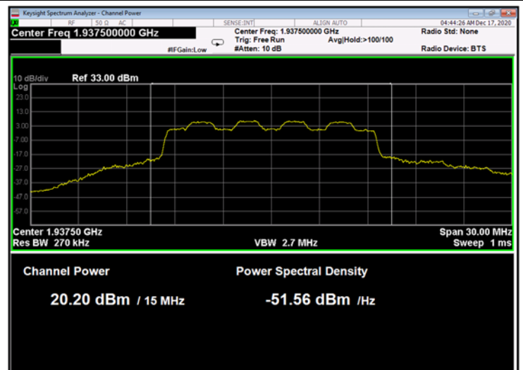
Figure 26: 16QAM 15MHz B.W.; 1937.5MHz, 60kHz
