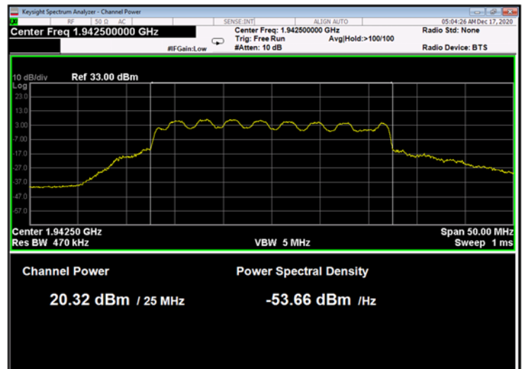
Figure 42: 16QAM 25MHz B.W.; 1942.5MHz, 15kHz
