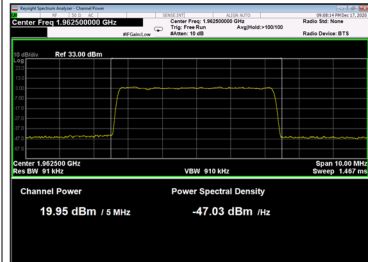
Figure 77: 64QAM 5MHz B.W.; 1962.5MHz, 15kHz
