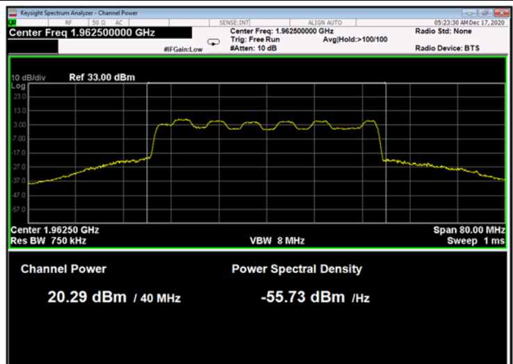
Figure 56: 16QAM 40MHz B.W.; 1962.5MHz, 60kHz
