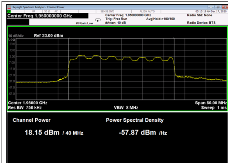
Figure 51: 16QAM 40MHz B.W.; 1950.0MHz, 15kHz
