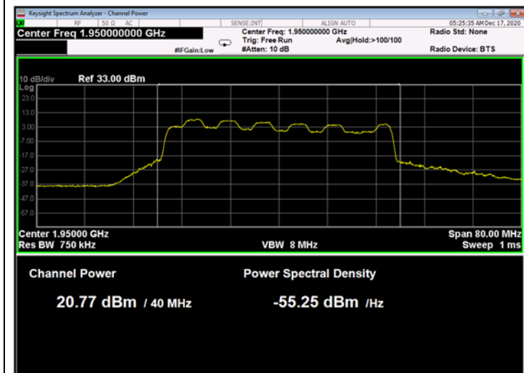
Figure 53: 16QAM 40MHz B.W.; 1950.0MHz, 60kHz
