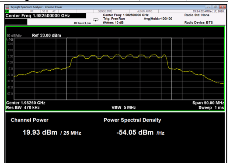
Figure 50: 16QAM 25MHz B.W.; 1982.5MHz, 60kHz
