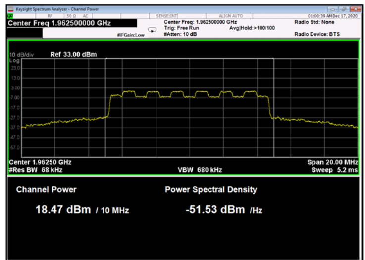
Figure 18: 16QAM 10MHz B.W.; 1962.5MHz, 15kHz
