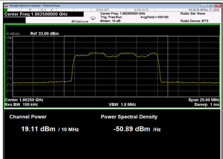
Figure 20: 16QAM 10MHz B.W.; 1962.5MHz, 60kHz
