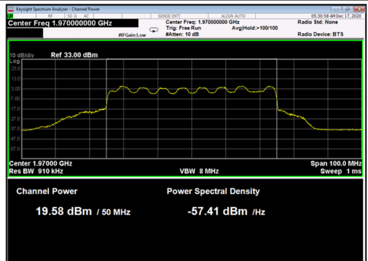
Figure 66: 16QAM 50MHz B.W.; 1970.0MHz, 15kHz
