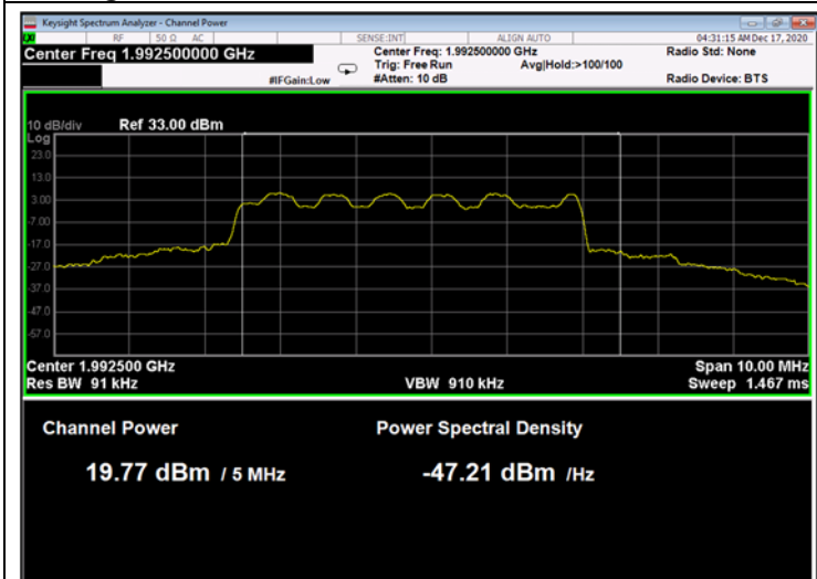
Figure 13: 16QAM 5MHz B.W.; 1992.5MHz, 15kHz
