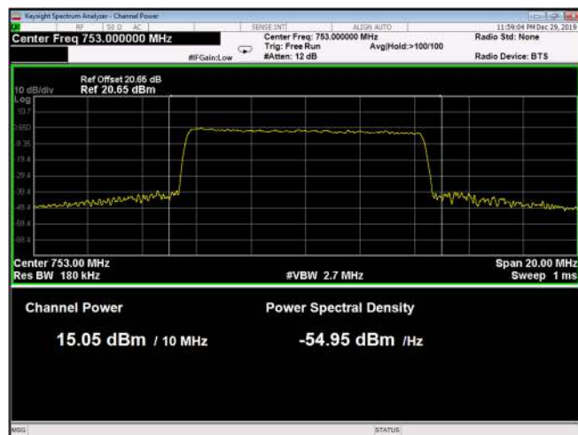
Figure 88: 256QAM 10MHz B.W.; 753.0MHz, 30kHz
