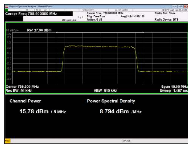
Figure 80: 256QAM 5MHz B.W.; 755.5MHz, 30kHz
