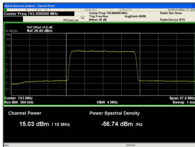
Figure 62: 64QAM 15MHz B.W.; 743.0MHz, 60kHz
