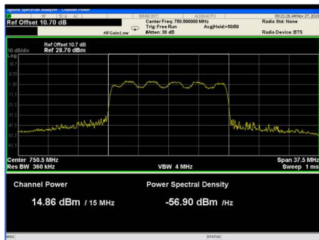
Figure 30: 16QAM 15MHz B.W.; 750.5MHz, 15kHz
