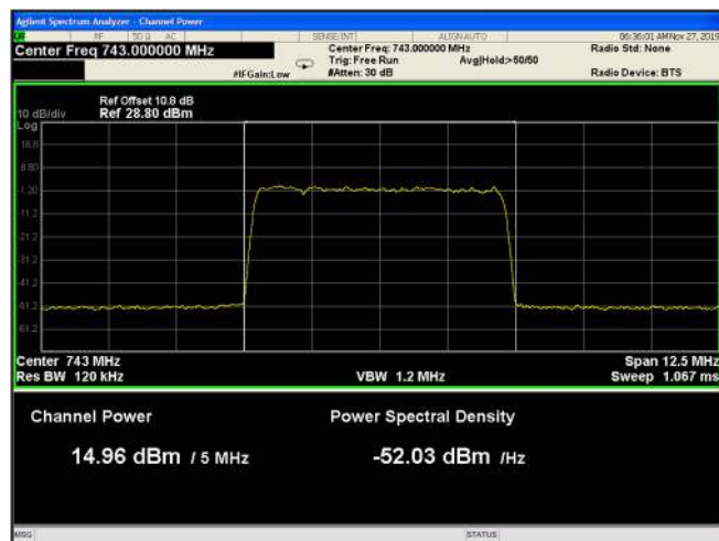
Figure 44: 64QAM 5MHz B.W.; 743.0MHz, 15kHz
