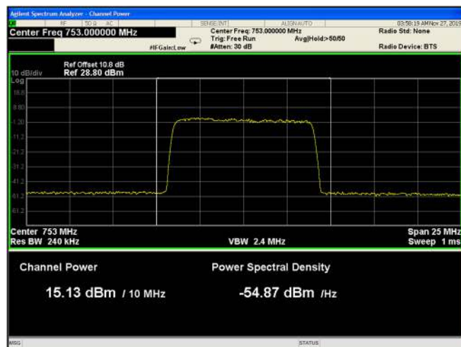
Figure 56: 64QAM 10MHz B.W.; 753.0 MHz, 60kHz
