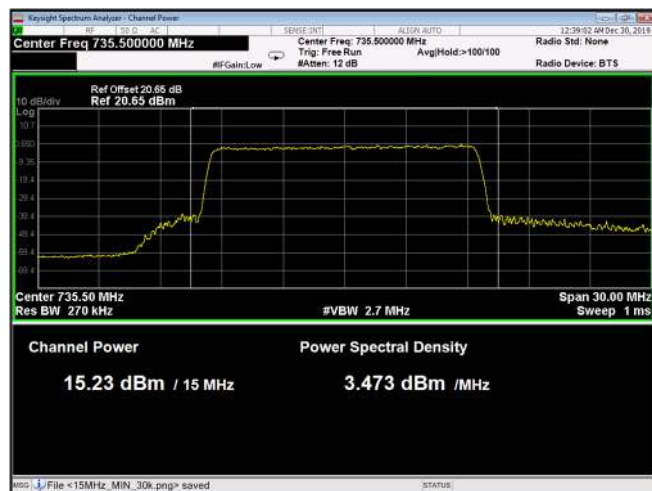
Figure 92: 256QAM 15MHz B.W.; 735.5MHz, 60kHz
