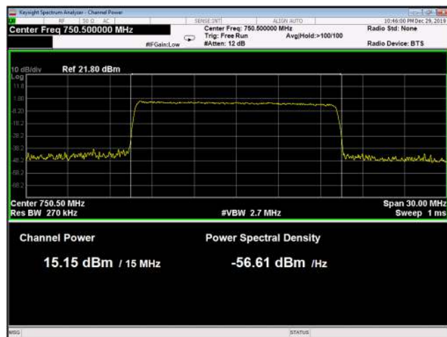
Figure 126: QPSK 15MHz B.W.; 750.5MHz, 15kHz
