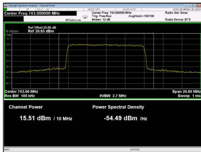
Figure 86: 256QAM 10MHz B.W.; 743.0MHz, 60kHz
