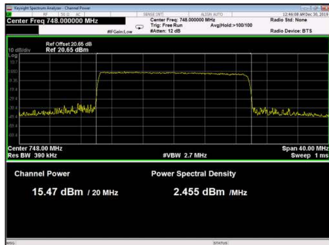
Figure 102: 256QAM 20MHz B.W.; 748.0MHz, 15kHz
