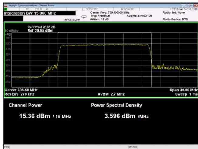
Figure 90: 256QAM 15MHz B.W.; 735.5MHz, 15kHz
