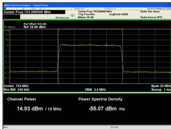
Figure 54: 64QAM 10MHz B.W.; 753.0MHz, 15kHz
