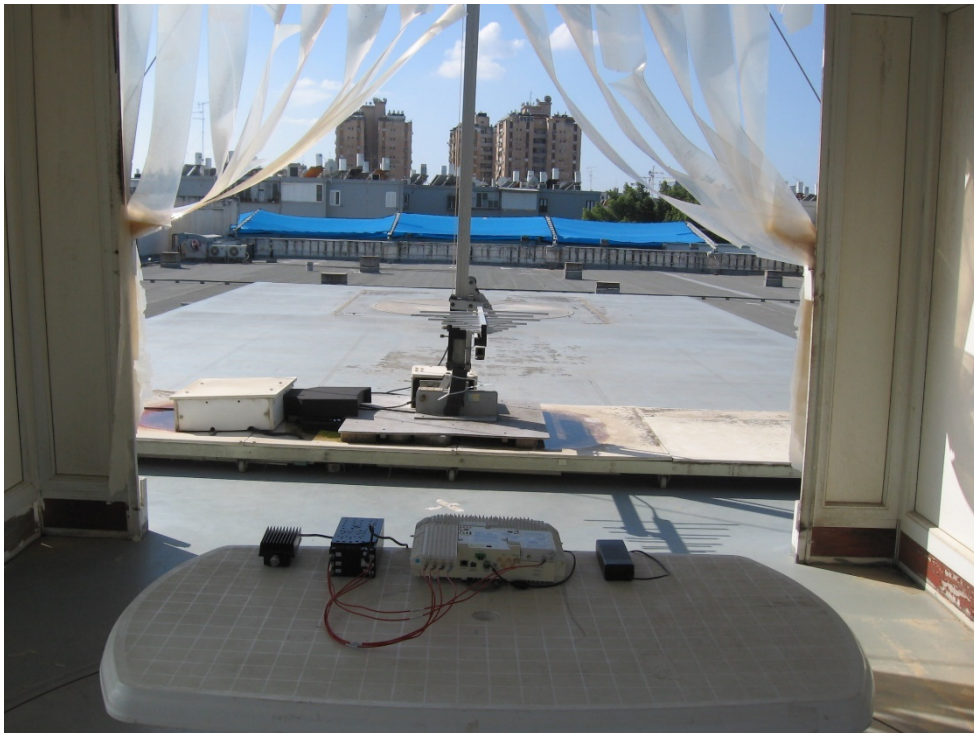
Figure 4. Radiated Emission Test 200 - 1000MHz
