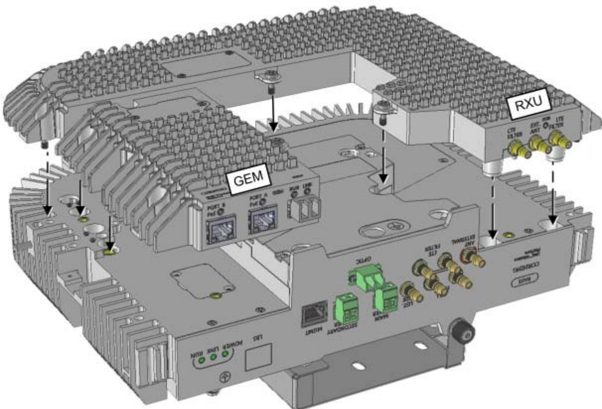
Figure 6-2. Plugging-in RxU and GEM
