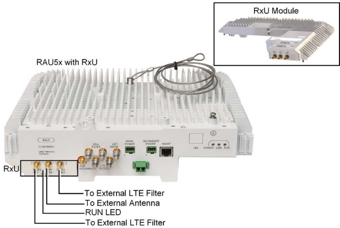
Figure 2-2. RxU Interfaces
