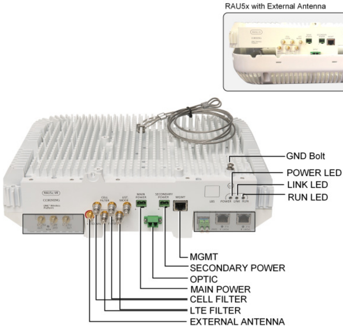
Figure 2-1. RAU5x Interfaces
