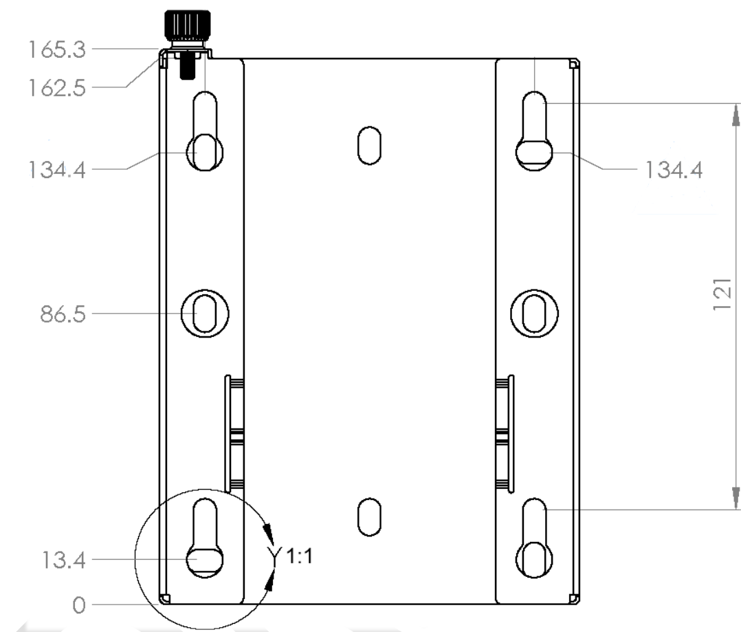
Figure 5-1. Standoff Mount Dimensions
