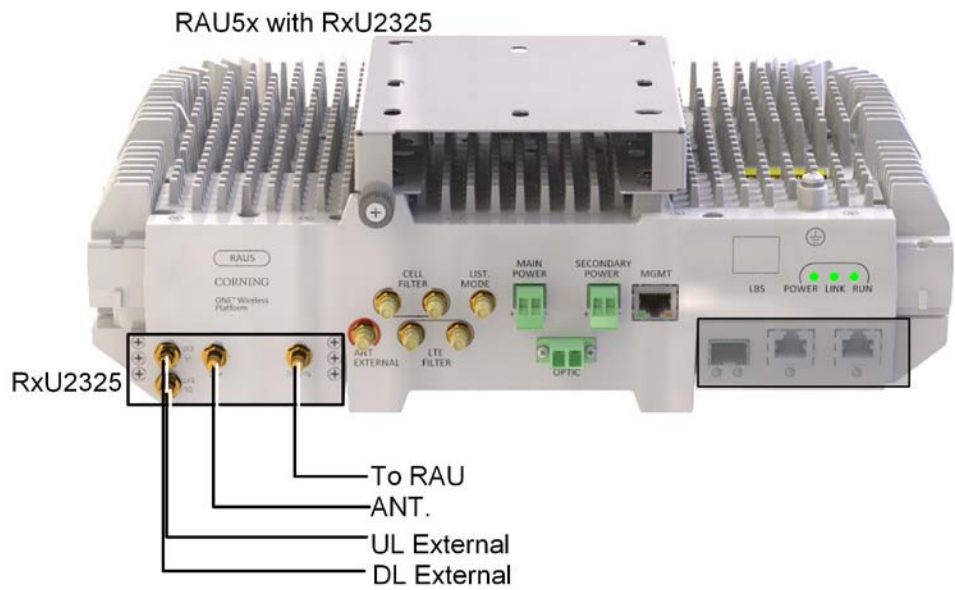
Figure 2-3. RxU2325 Interfaces
