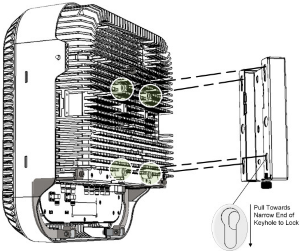
Figure 4-3. Mounting RAU5x onto Bracket
