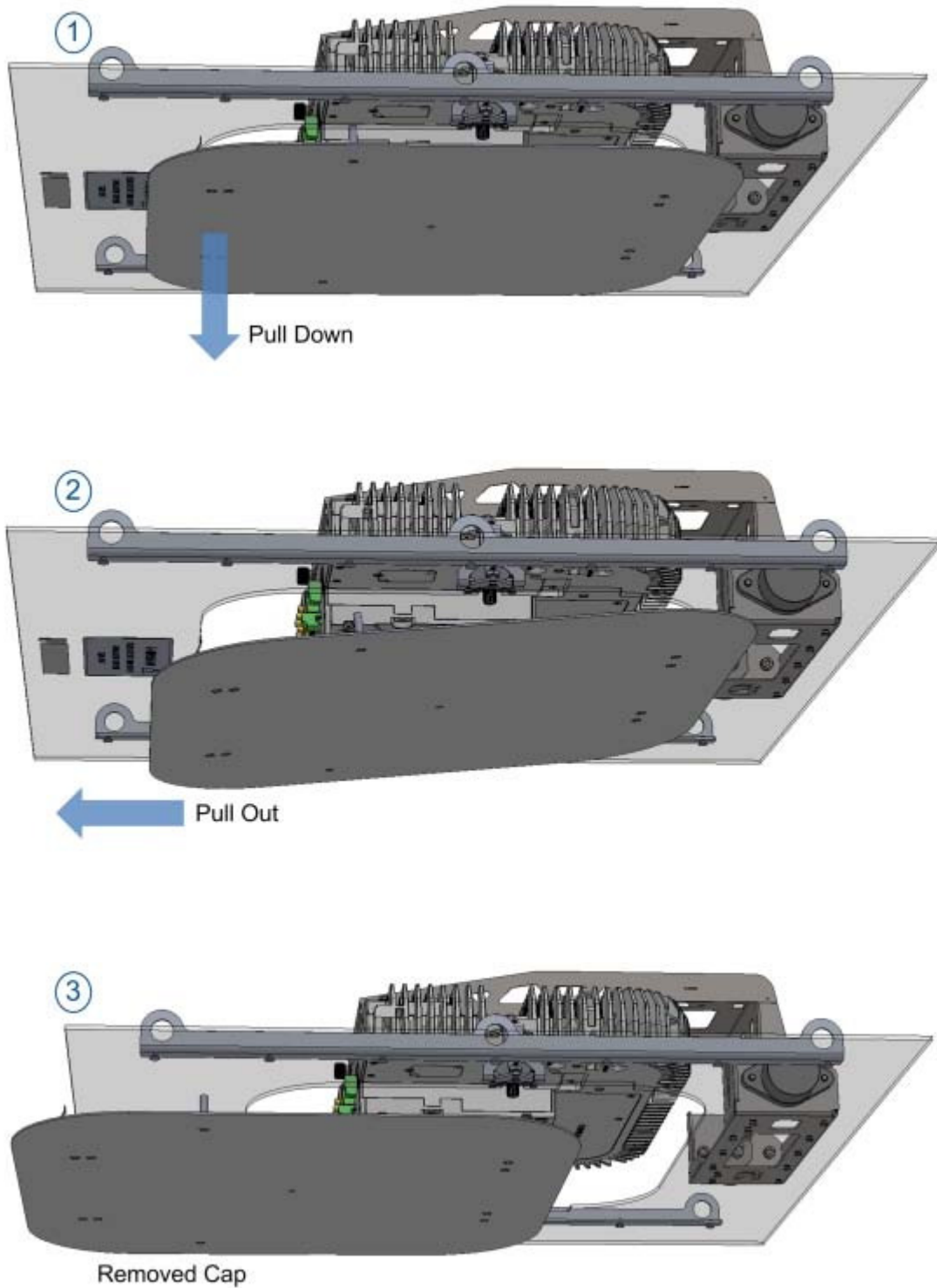
Figure 4-17. Removing Cap
