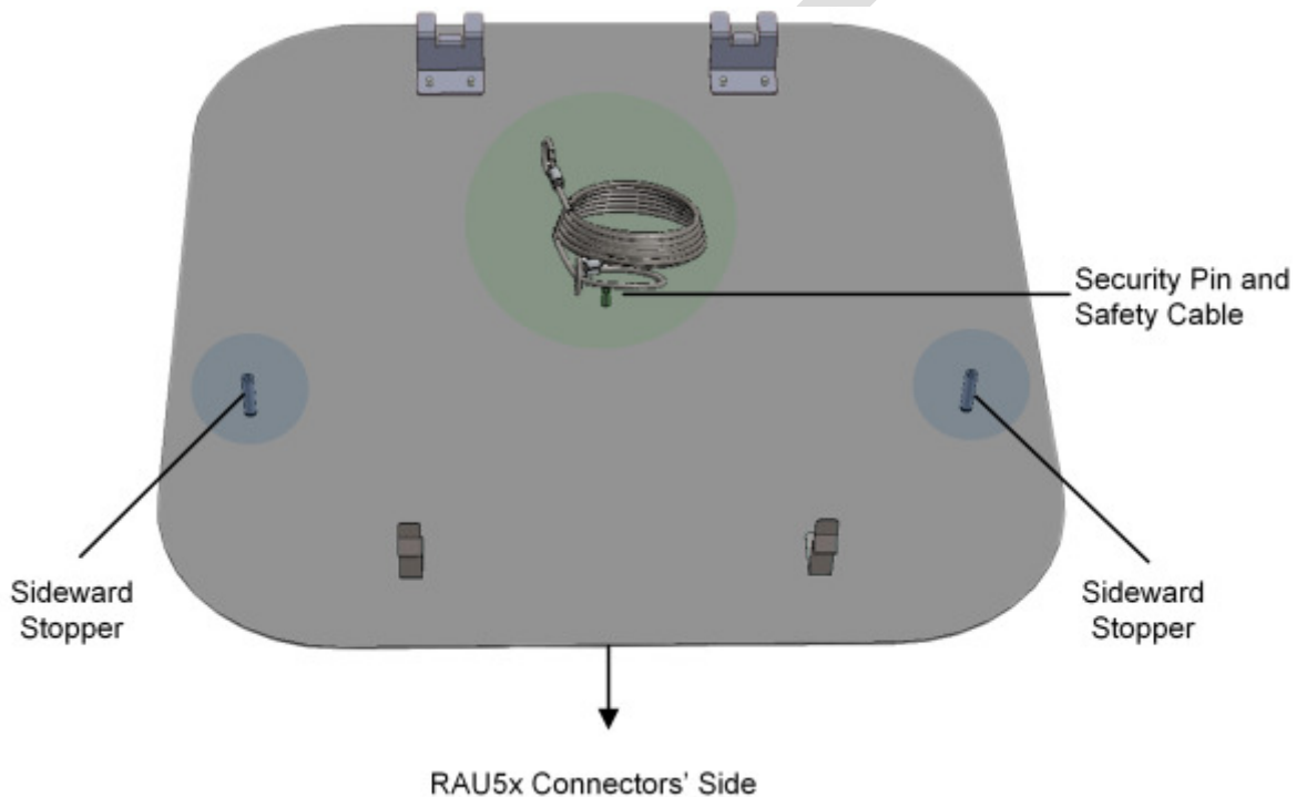
Figure 4-14. BR-TOP-CAP
