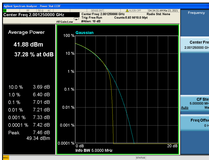
DL_1S_f0_Pre-AGC_PAPR
