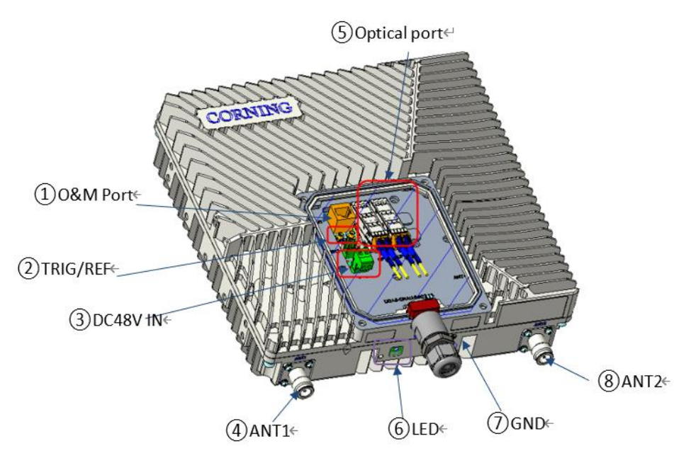
Figure 21. dLRU-G2-678
