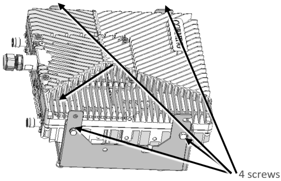
Figure 42. 4 Screws
