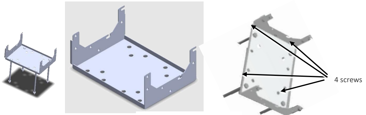
Figure 41. 4 Screws
