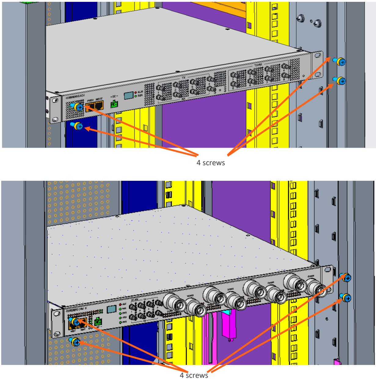
Figure 28. RIU Rack Installation
