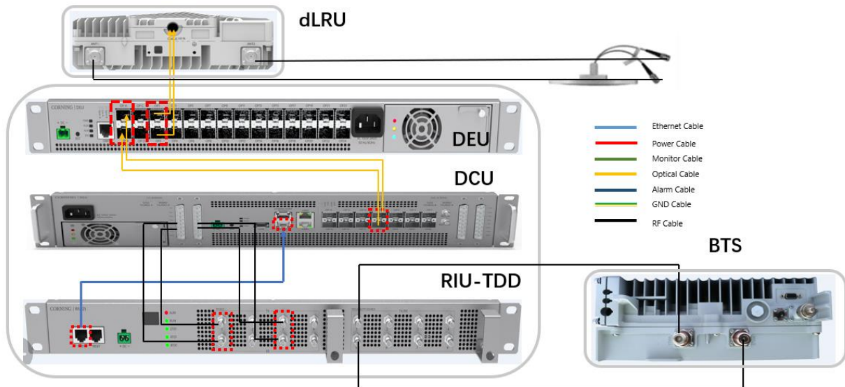
Figure 27. dLRU-TDD Architecture Image
