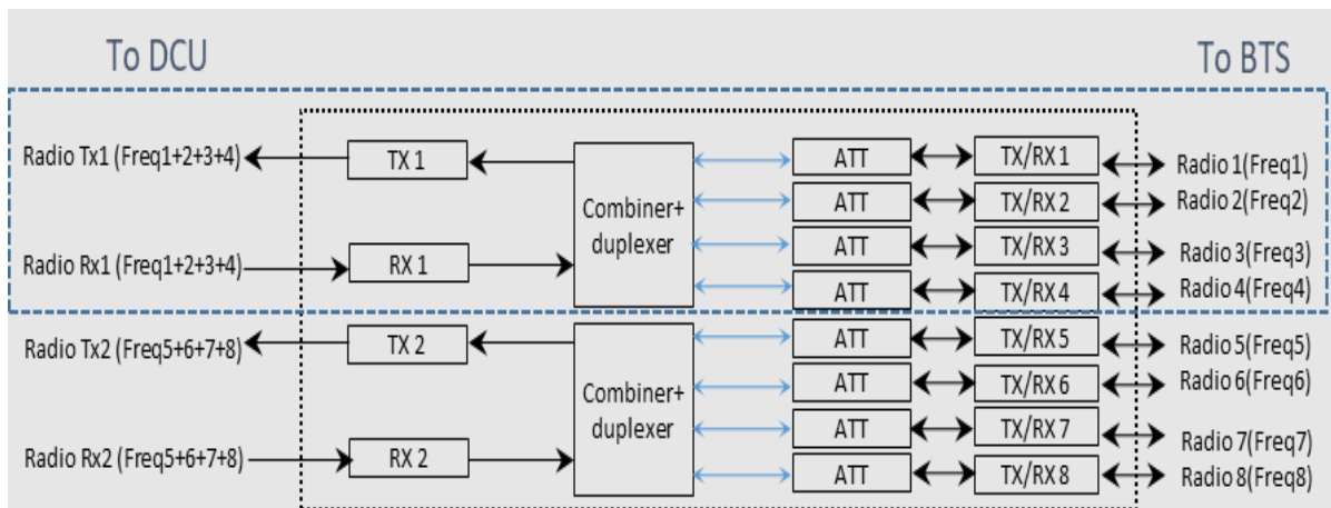
Figure 4. 4 TO 1 Matrix
