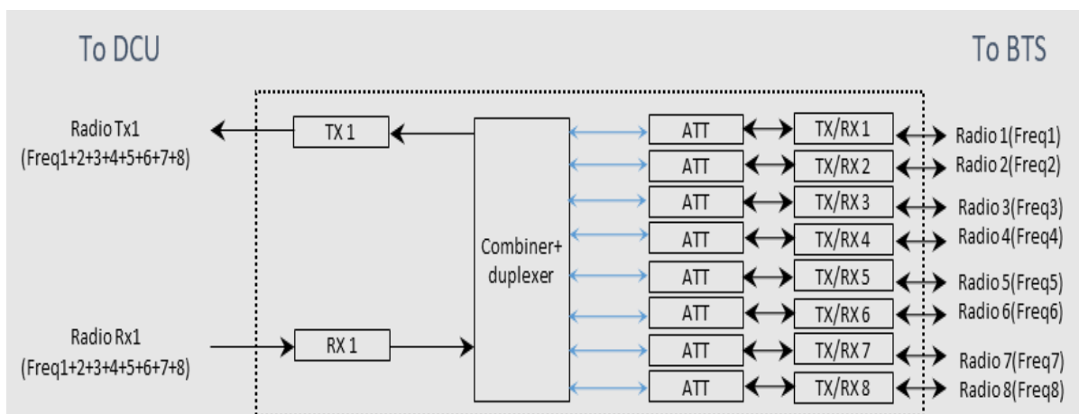
Figure 5. 8 TO 1 Matrix
