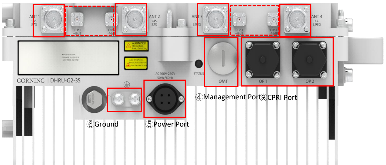
Figure 105. dHRU TDD-35 Front View
