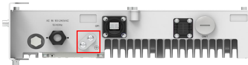
Figure 99. GND Connection
