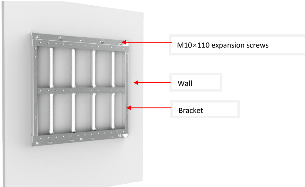
Figure 110.Wall mounted installation
