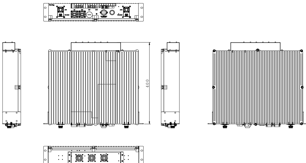
Figure 72. dMRU Dimensions - with Fan
