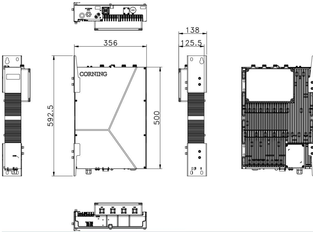
Figure 86.dHRU-700 Dimension
