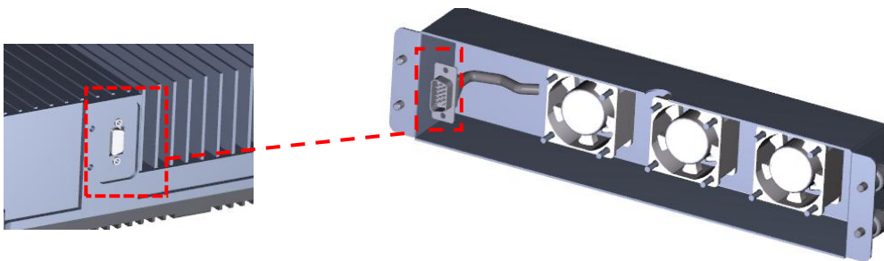
Figure 78. Fan Connection with DB15
