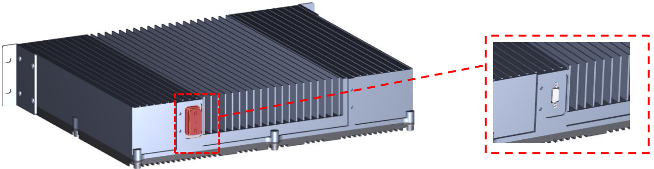
Figure 77. Fan Connection
