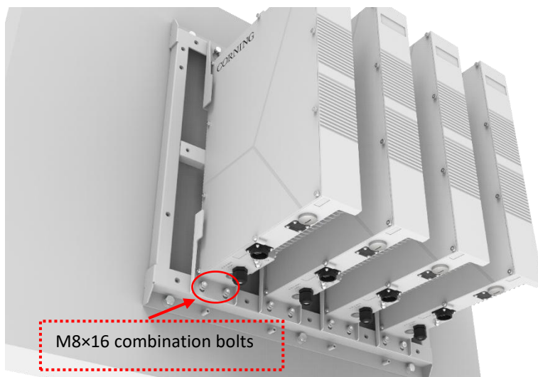
Figure 97. Tighten screw M8×16 combination bolts
