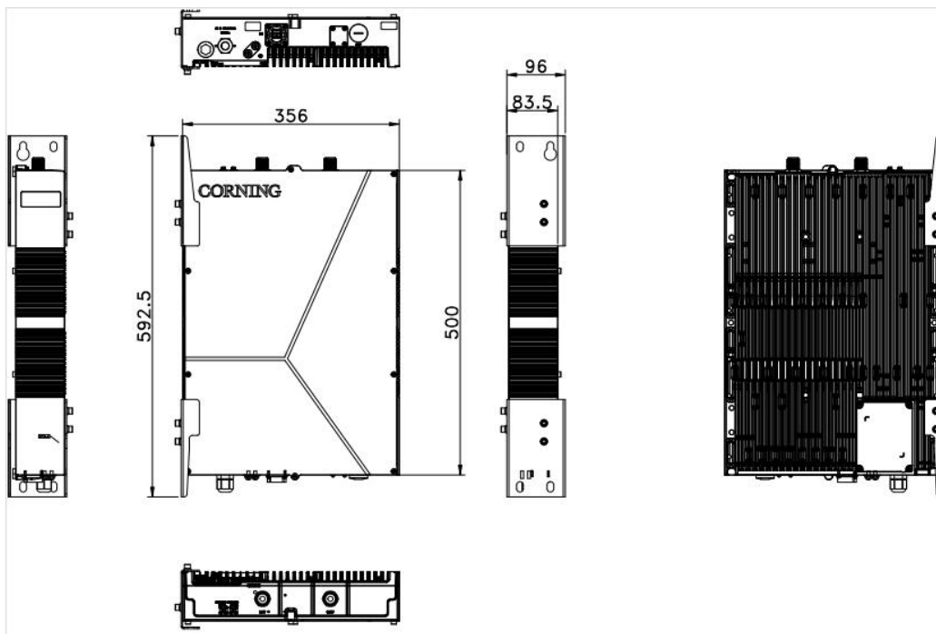
Figure 87. dHRU-600 Dimension
