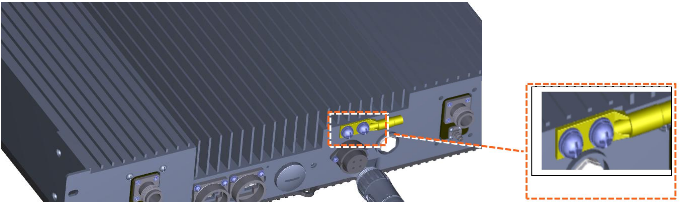
Figure 83. GND Connection
