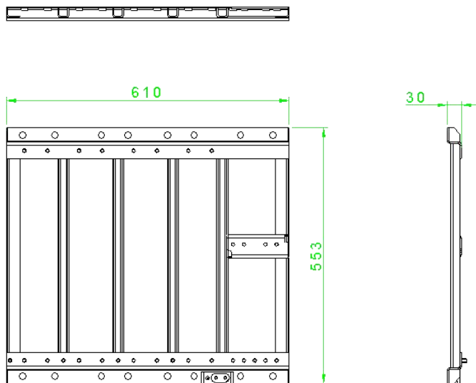
Figure 81.dMRU bracket dimensions
