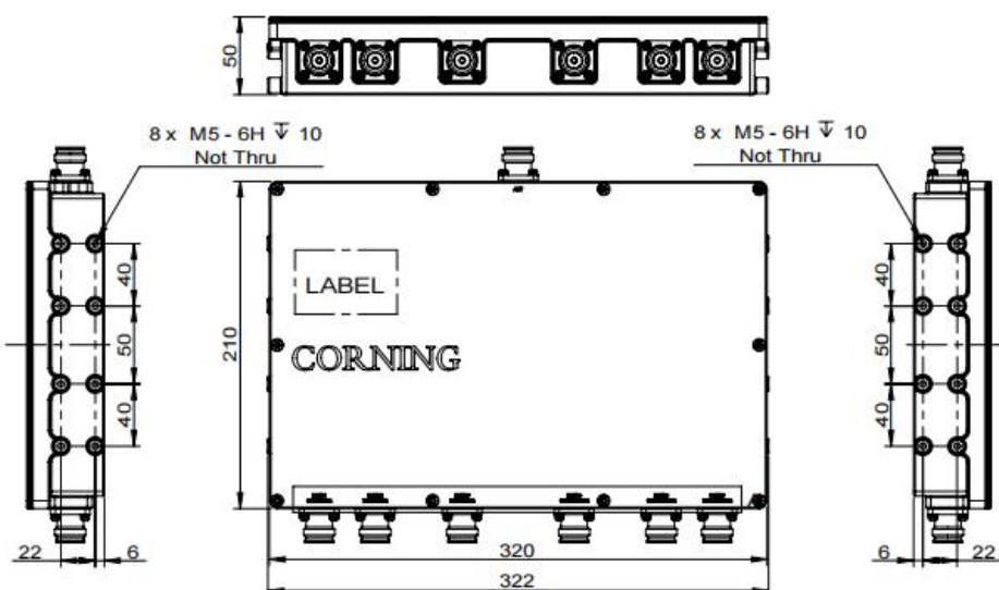
Figure 89.dHRU-G2-COMB-L combiner
