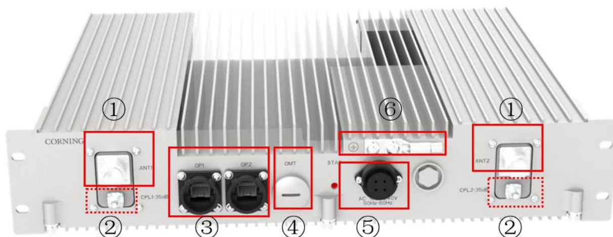
Figure 73. dMRU Front View
