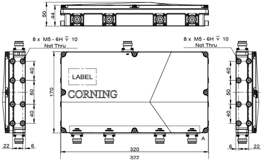
Figure 103. dHRU TDD Combiner Dimensions
