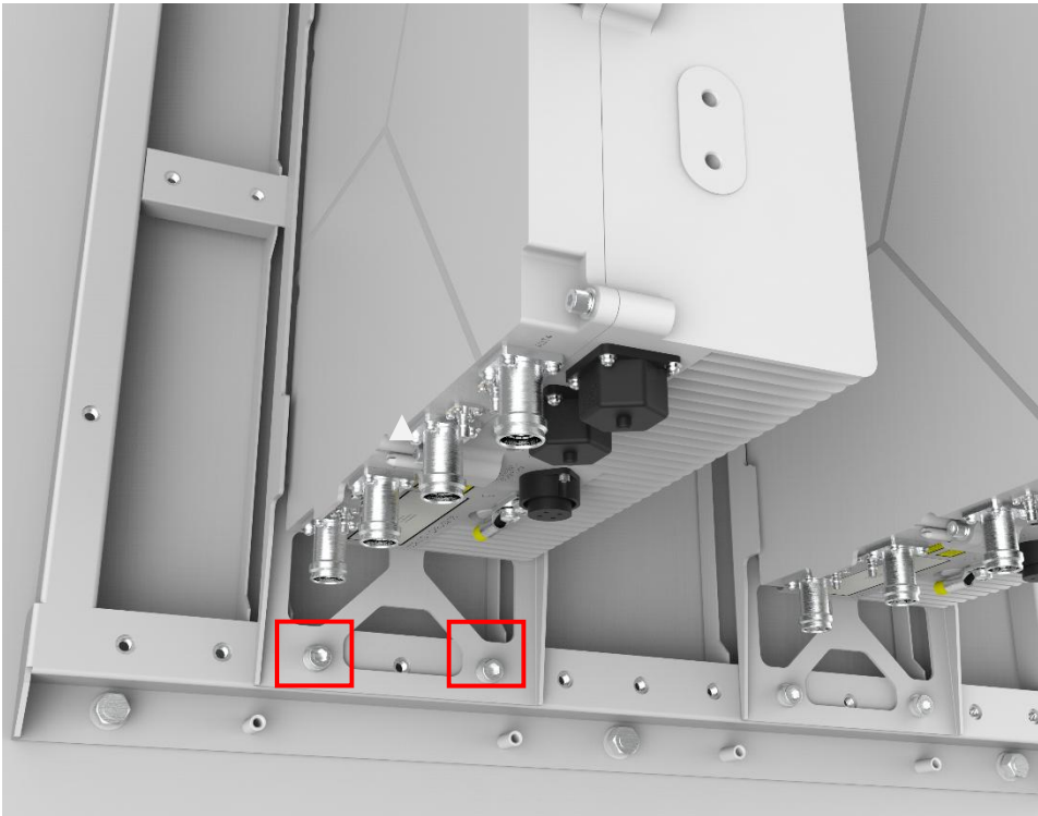
Figure 112. Fasten screws M8×16 combination bolts
