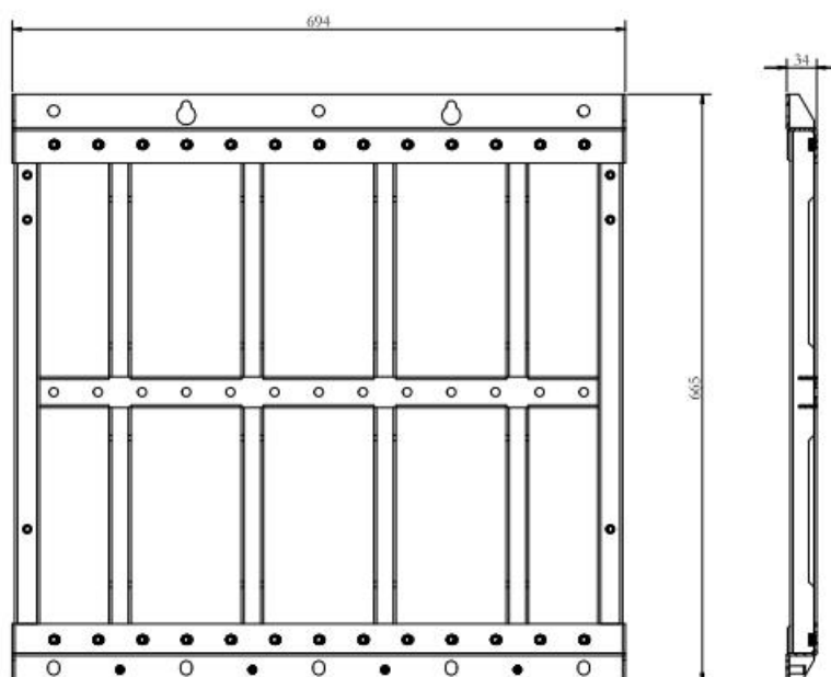
Figure 88.dHRU Bracket Dimension
