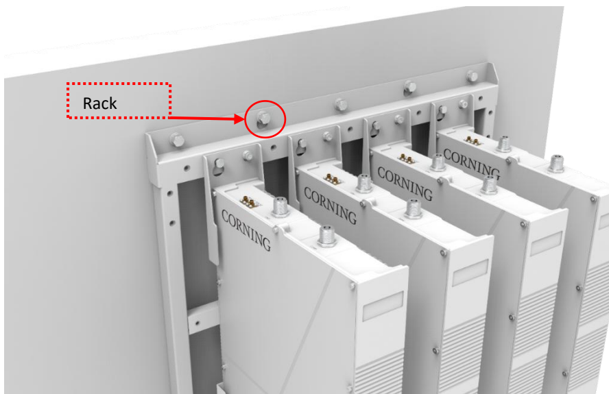
Figure 96. Wall mounted installation
