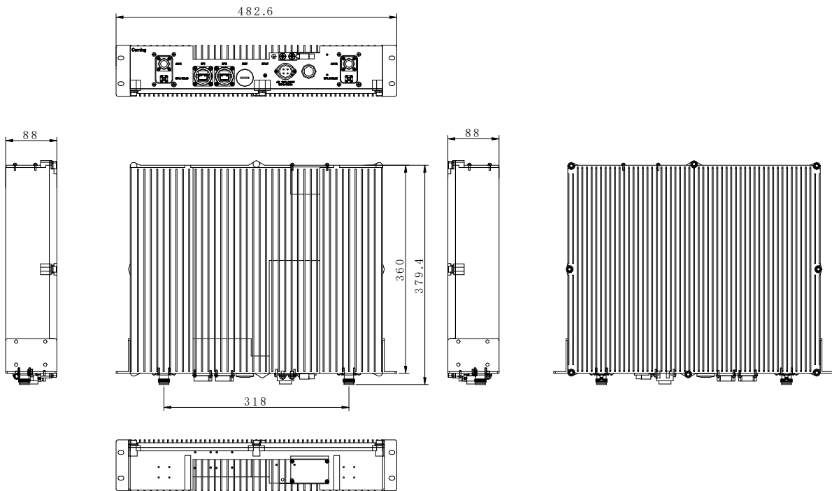
Figure 71. dMRU Dimensions - Without Fan
