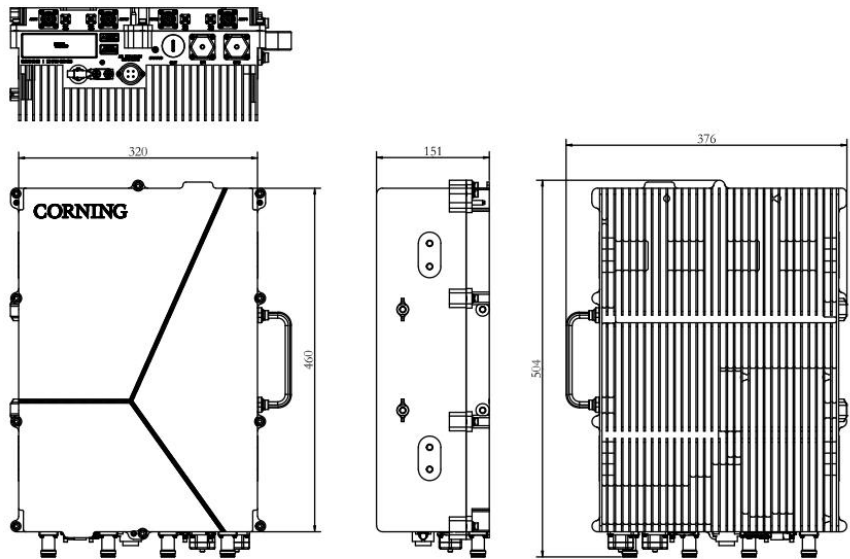
Figure 102. dHRU TDD Dimensions
