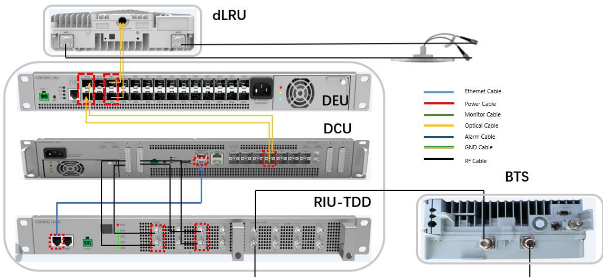
Figure 30.dLRU-TDD Architecture Image
