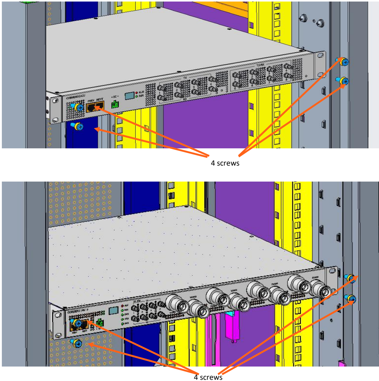
Figure 31. RIU Rack Installation
