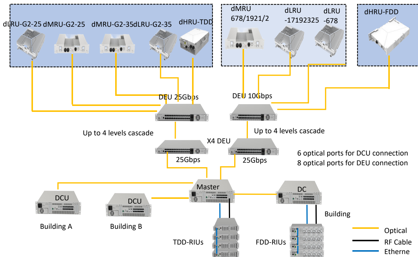
Figure 27. System Topology
