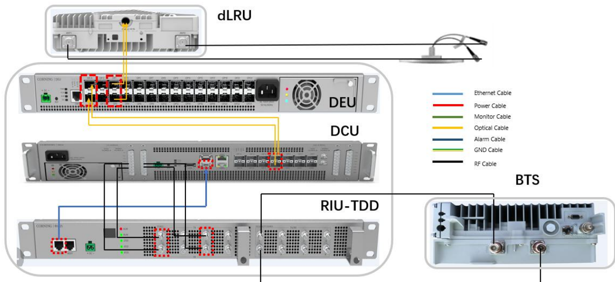
Figure 30.dLRU-TDD Architecture Image
