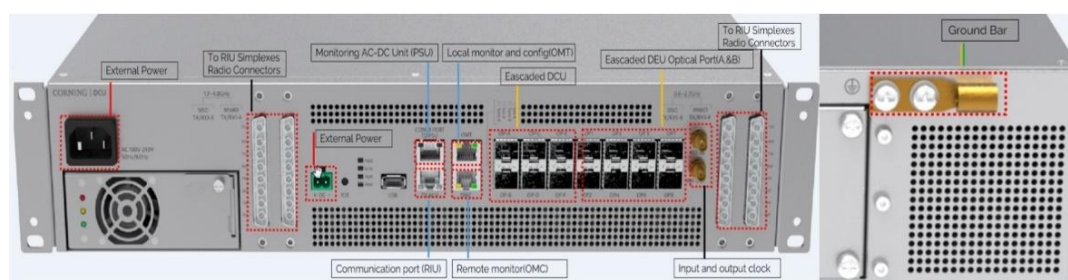
Figure 38. DCU Cable Connection
