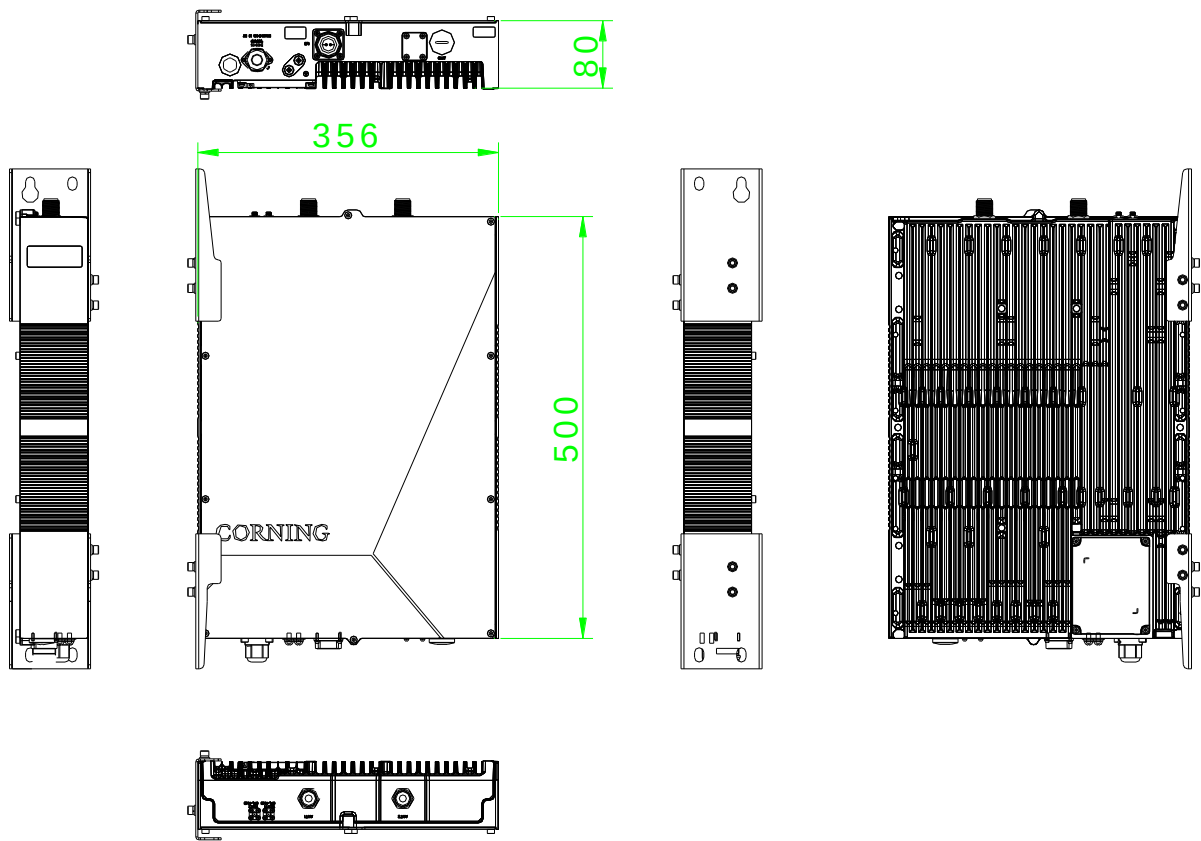
Figure 83. dHRU Dimensions
