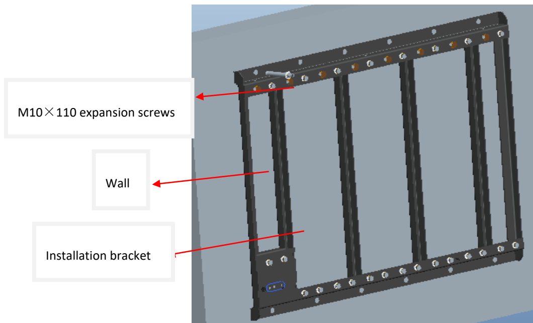
Figure 89. Wall mounted installation
