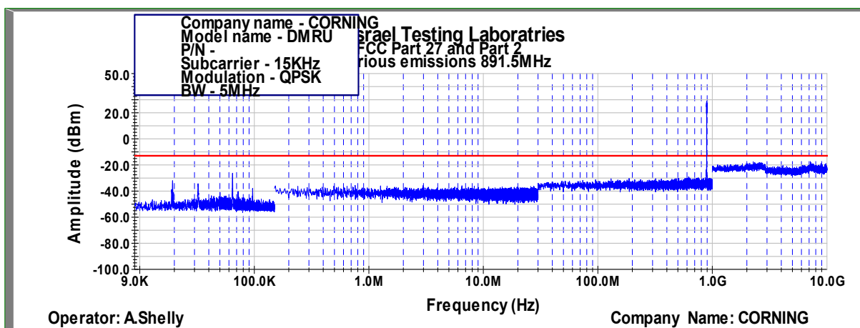
Figure 438: Spurious Emissions at Antenna Terminal QPSK, 891.5MHz, B.W. 5MHz, Sub Carrier 15kHz
