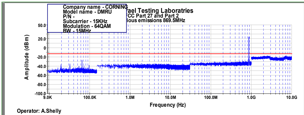
Figure 412: Spurious Emissions at Antenna Terminal 64QAM, 869.5MHz, B.W. 15MHz, Sub Carrier 15kHz
