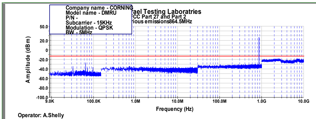
Figure 436: Spurious Emissions at Antenna Terminal QPSK, 864.5MHz, B.W. 5MHz, Sub Carrier 15kHz
