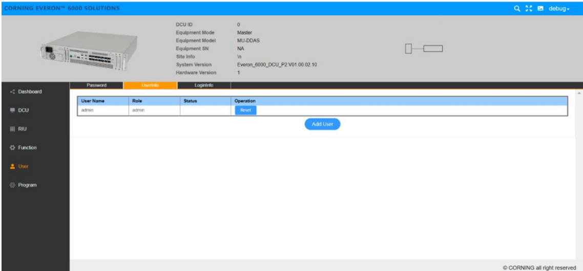
Figure 95 DCU→User→UserInfo
