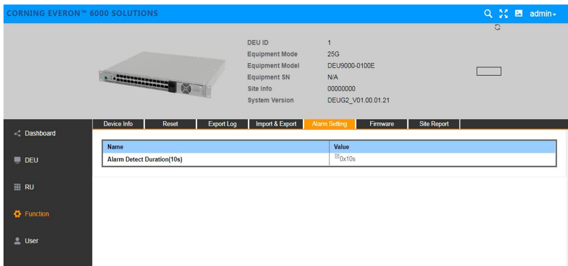
Figure 109 DEU→Function→Alarm Setting
