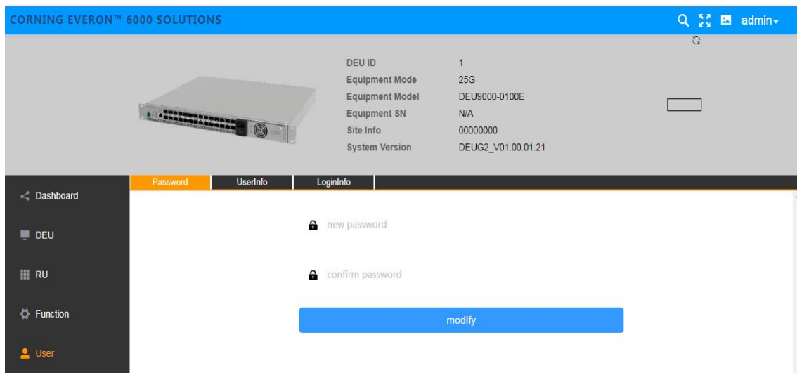
Figure 112 DEU→User→Password
