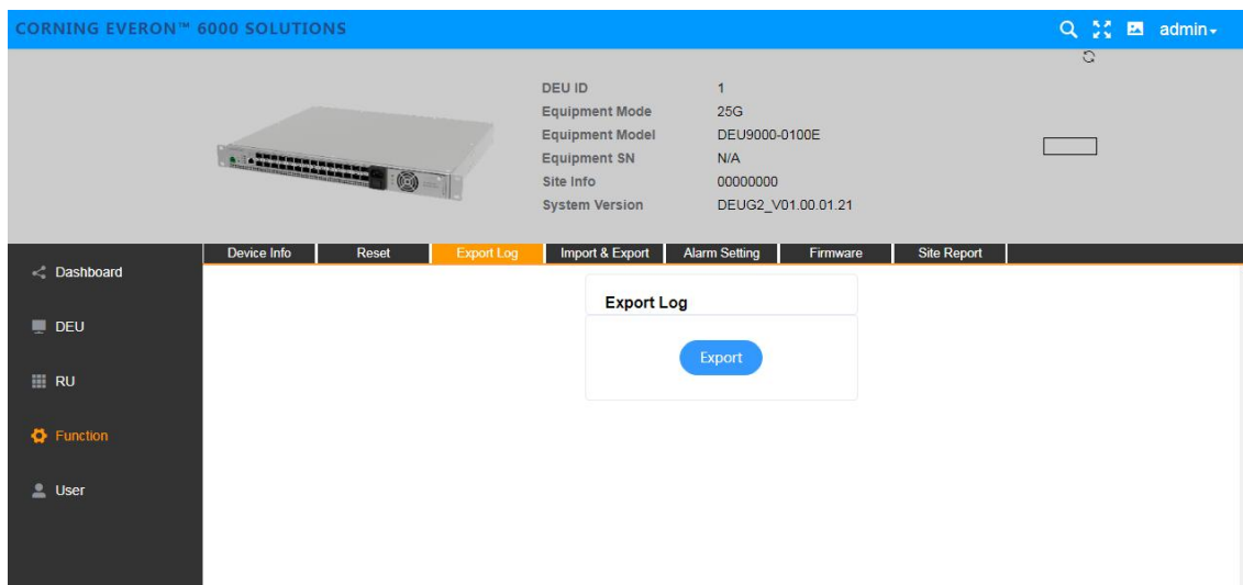
Figure 107 DEU→Function→Export Log
