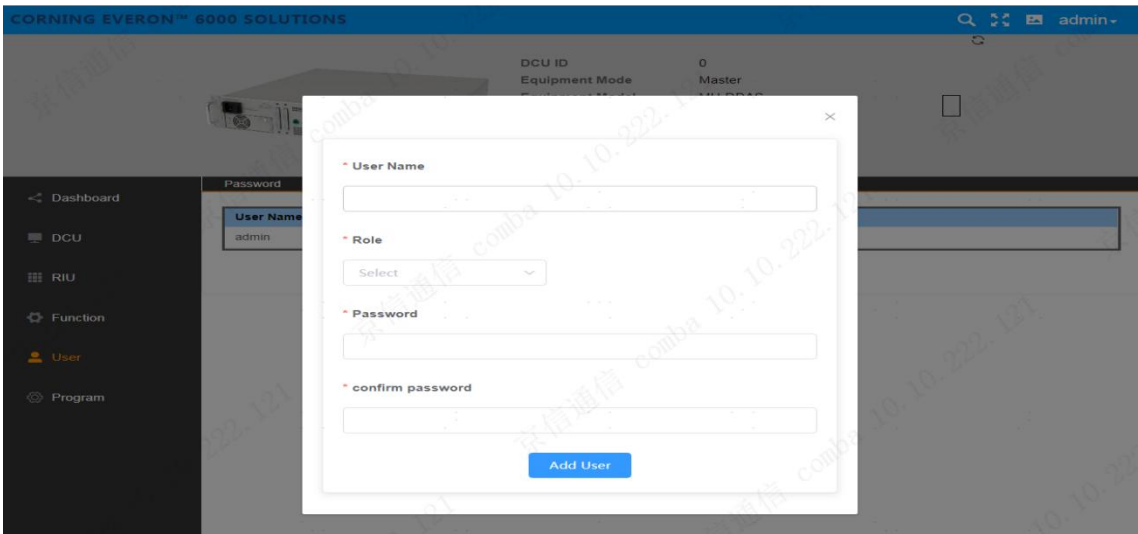
Figure 96 DCU→User→UserInfo→Add User
