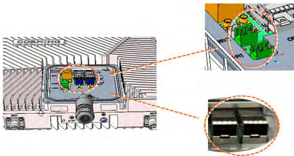
Figure 55 Power socket
