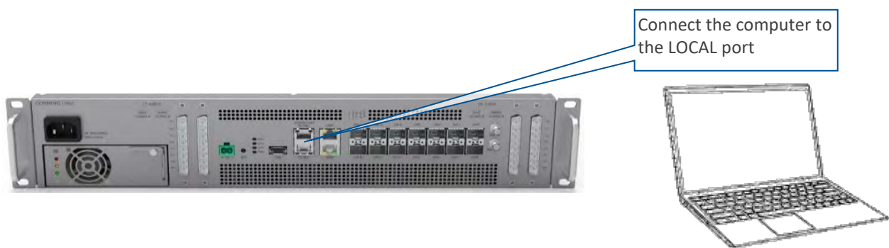
Figure 63 GUI connection
