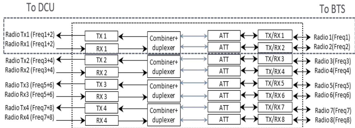
Figure 3. 2 TO 1 matrix
