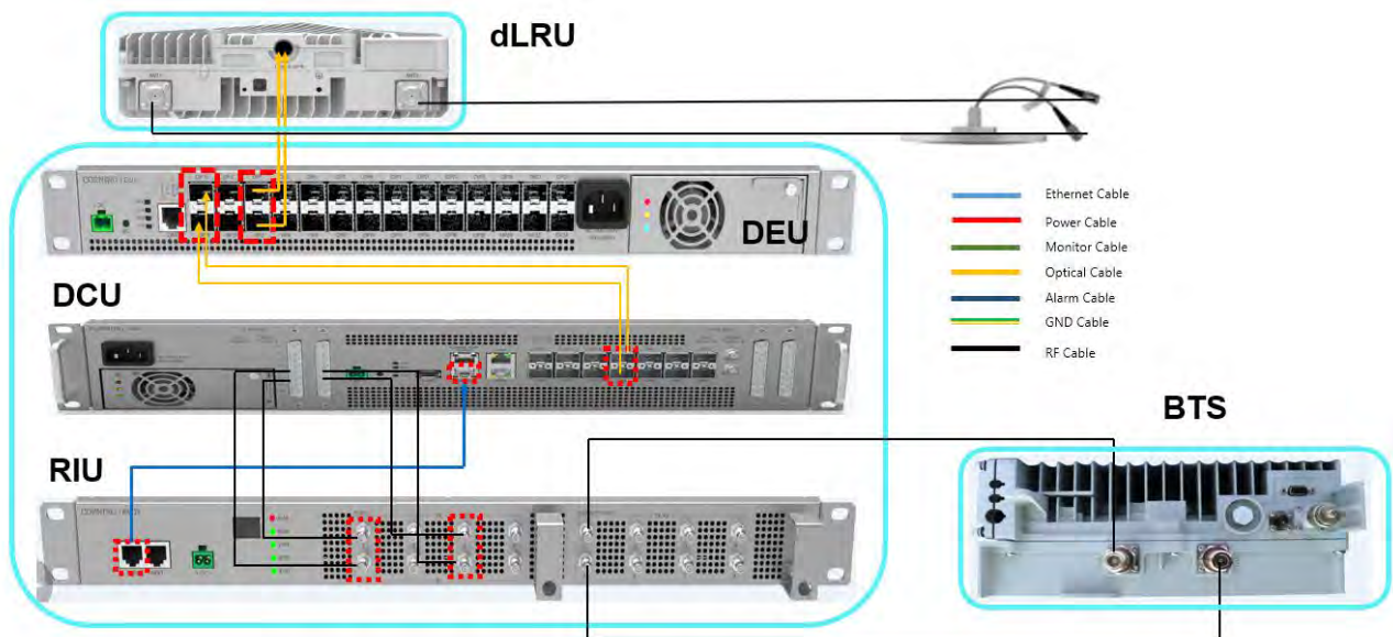
Figure 25 dLRU architecture image
