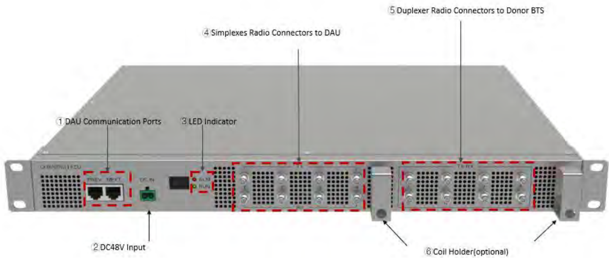
Figure 7. RIU Interface(front view)
