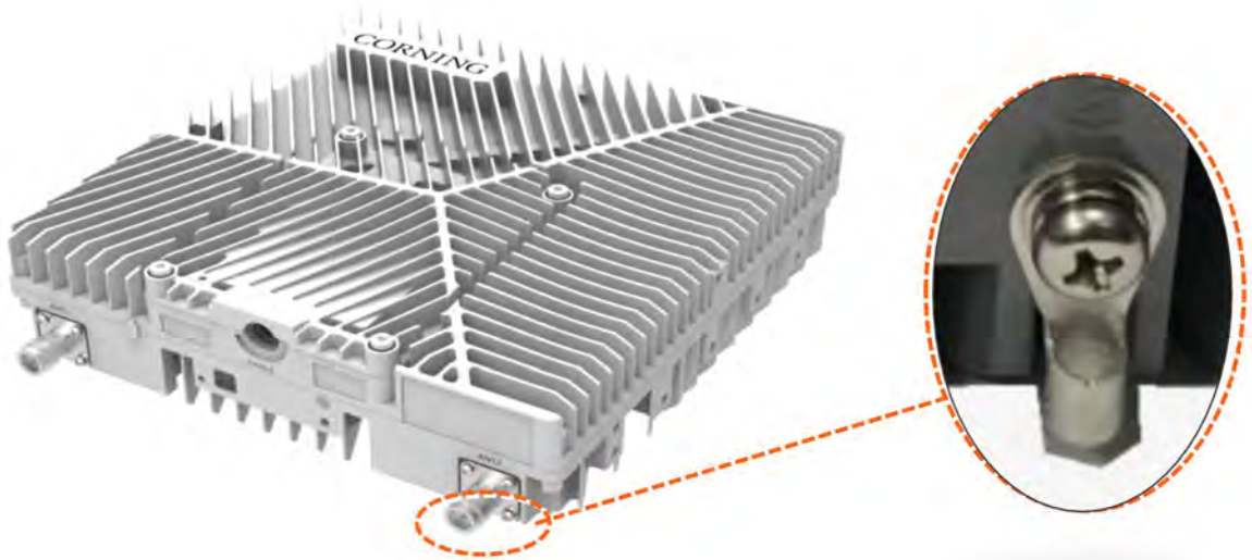
Figure 57 The ground
