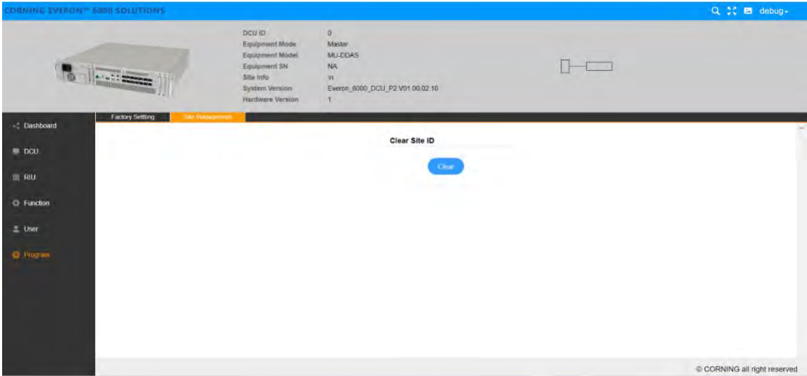
Figure 99 DCU→ Program
