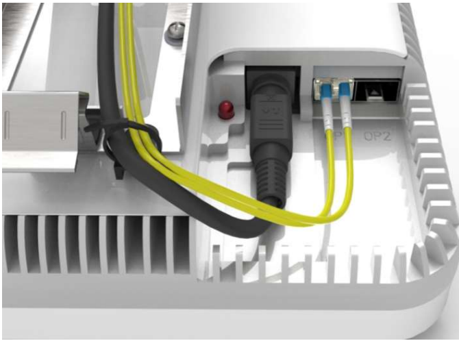
Figure 74. Wire Connection Diagram
