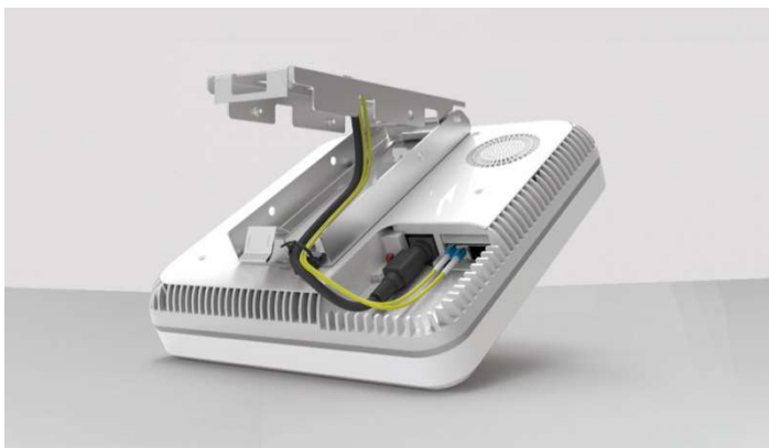
Figure 47. Unlock Rotary Hook Diagram 2
