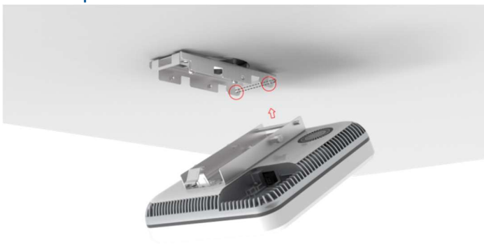
Figure 53. Connecting Bar over Hooks on Bracket II
