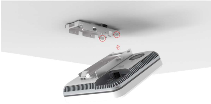
Figure 42. Connecting Bar over Hooks on Bracket II
