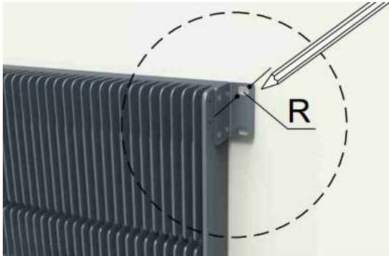
Figure 31. Marking the Position of Mounting Holes
