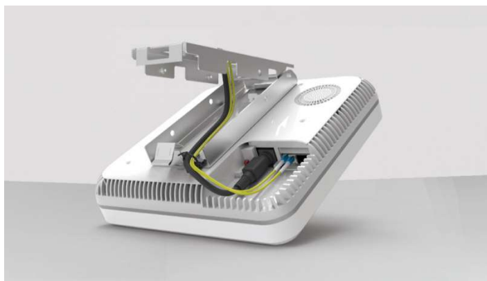
Figure 58. Top Panel of E62-N2RU Exposed
