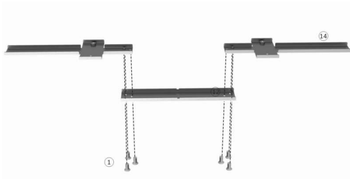
Figure 61. Assembling Bracket I & VI
