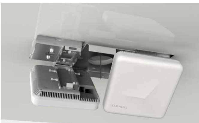
Figure 72. Buckle the Bracket 2
