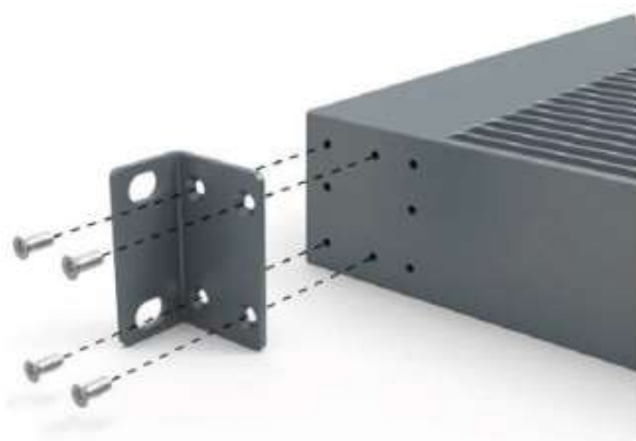
Figure 6. Attaching a 19-in Mounting Bracket
