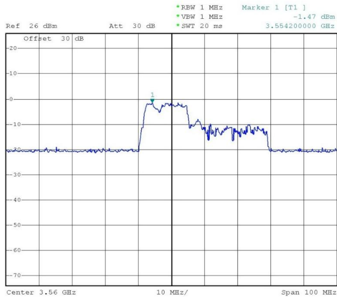
Figure 8.26-5: Granted maxEIRP = 5 dBm/MHz
