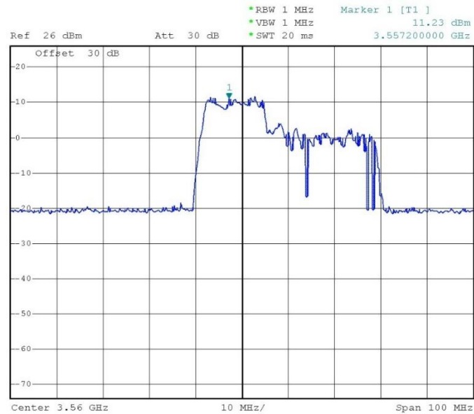
Figure 8.26-2: Granted maxEIRP = 20 dBm/MHz
