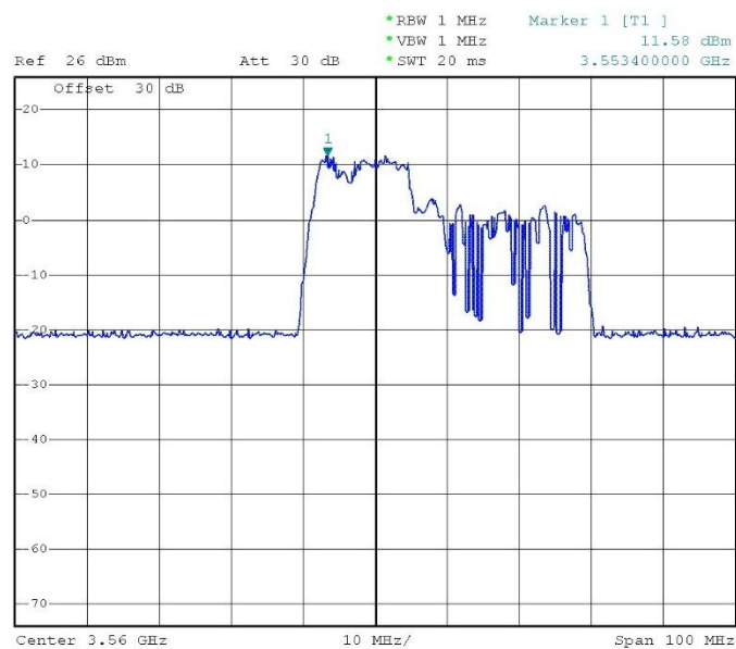
Figure 8.26-1: Granted maxEIRP = 25 dBm/MHz
