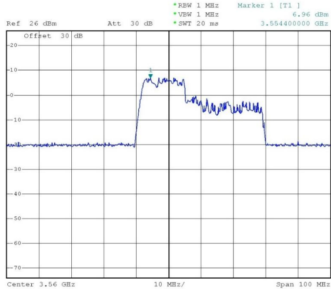
Figure 8.26-3: Granted maxEIRP = 15 dBm/MHz
