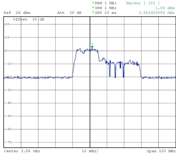
Figure 8.26-4: Granted maxEIRP = 10 dBm/MHz
