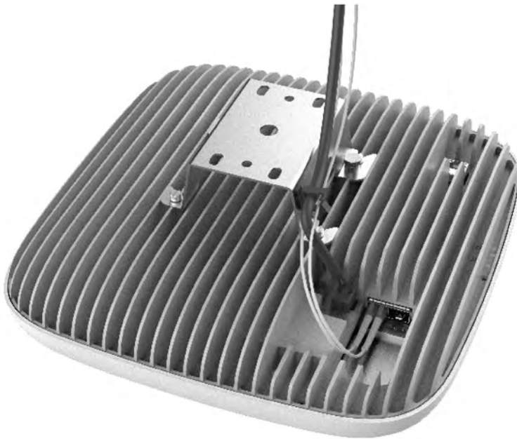
Figure 33. Connect power cable and fiber cable
