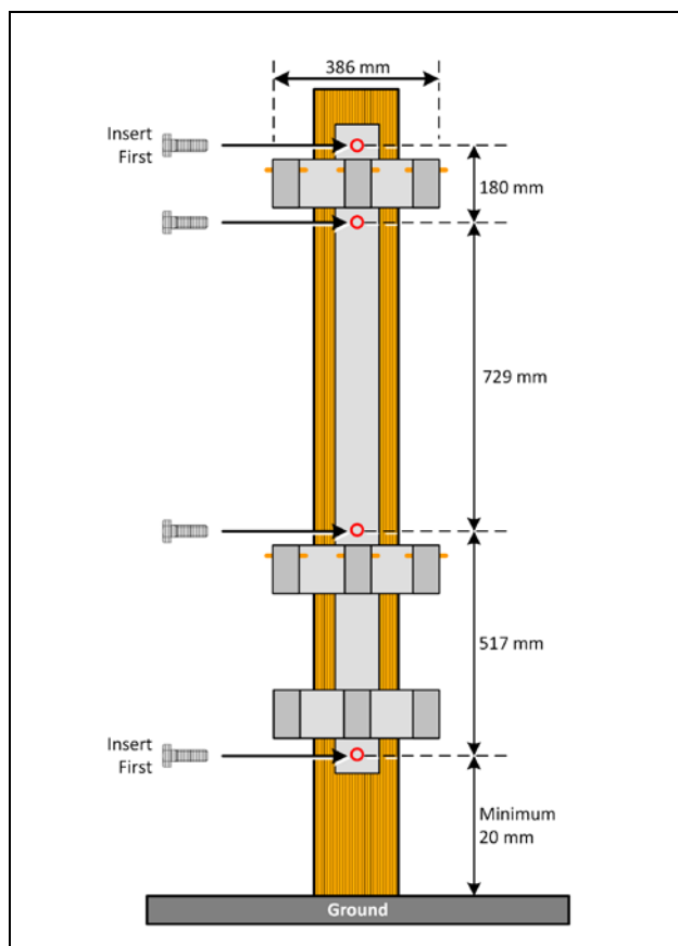
Mounting the Bracket | Figure 3.13
