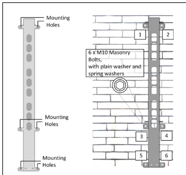
GX Bracket Wall-Mountable Option | Figure 3.5
