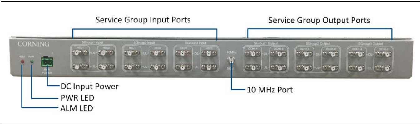
IFB Interfaces | Figure 1.8
