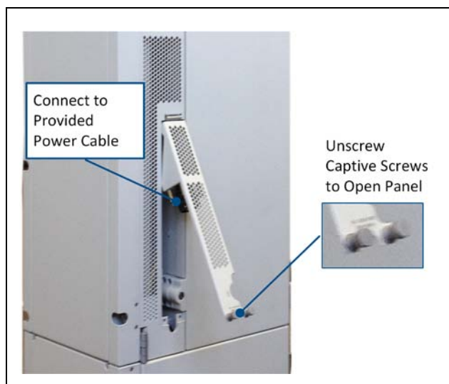
GX AC Model Power Connector | Figure 3.21
