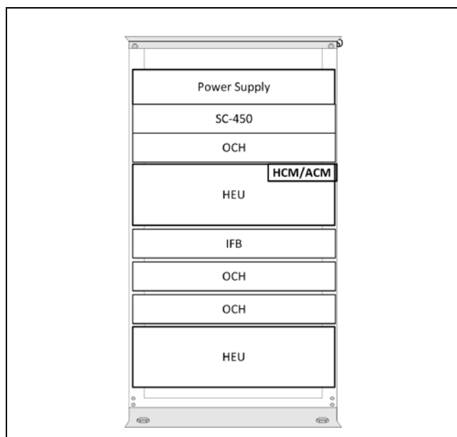
Example of Rack Configuration with HEU | Figure 3.1
