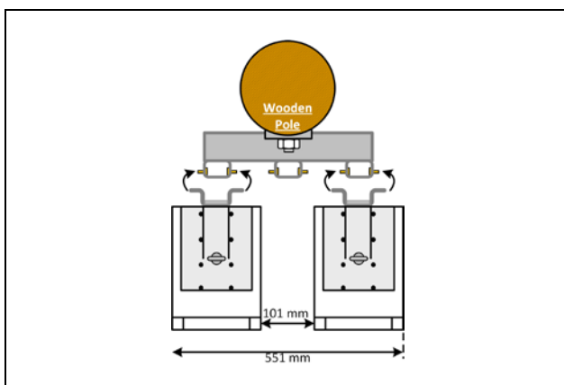
Dual-Mounted GX Units | Figure 3.16
