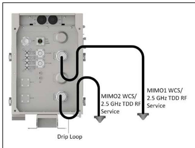
Illustration of GX Dual-Band (MIMO) Direct RF Connection to DAS | Figure 3.19
