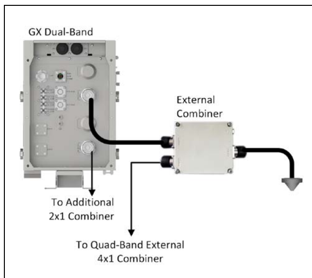
Illustration of GX and Dual-Band External Combiner Connections | Figure 3.20
