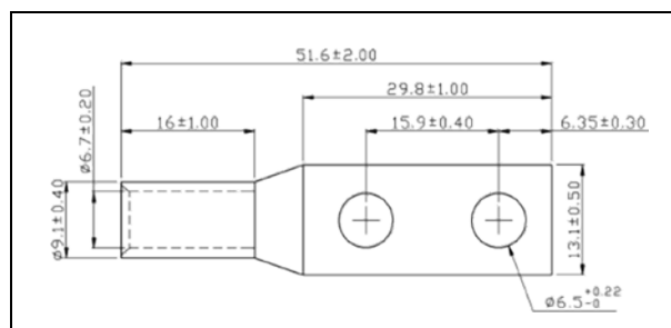
Example of Compliant DC Cable Lug | Figure 3.22
