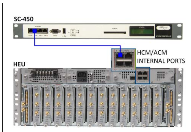
HCM-to-SC-450 Management Connection | Figure 3.4
