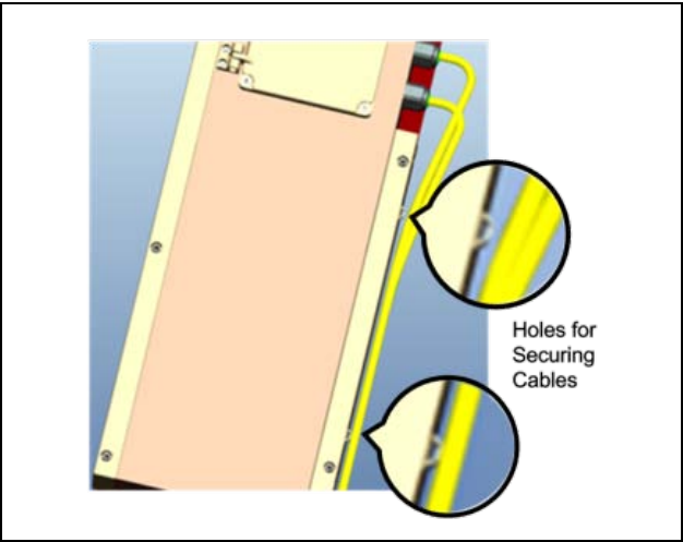
Fixed Power Cable | Figure 3.27
