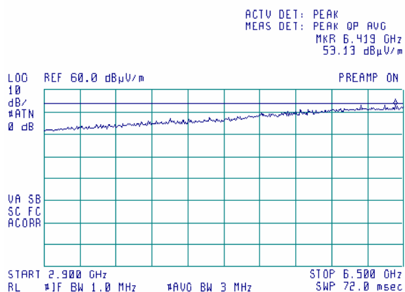
Plot 9.2.8 Radiated emission measurements in 2900 - 6500 MHz range, horizontal antenna polarization
