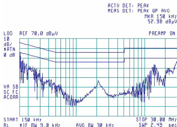
Plot 9.1.2 Conducted emission measurements
