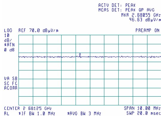
Plot 7.4.28 Radiated emission measurements at the forth harmonic of low carrier frequency
