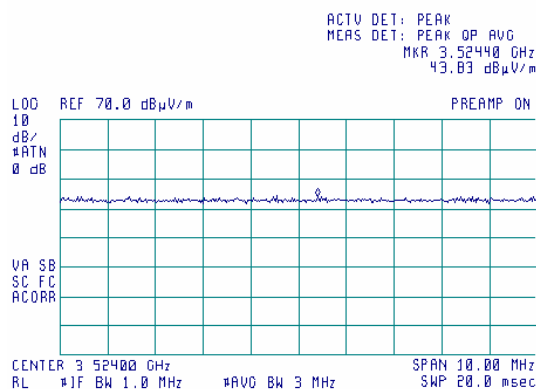
Plot 7.4.30 Radiated emission measurements at the forth harmonic of high carrier frequency
