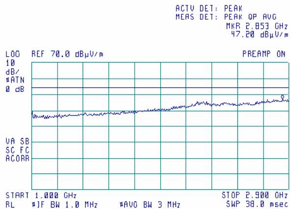
Plot 9.2.4 Radiated emission measurements in 1000 - 2900 MHz range, horizontal antenna polarization
