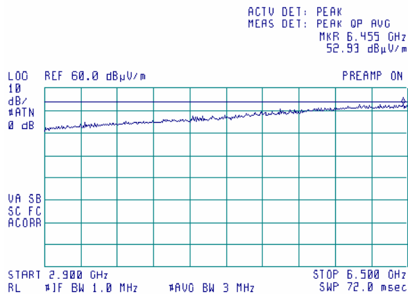
Plot 9.2.6 Radiated emission measurements in 2900 - 6500 MHz range, vertical antenna polarization
