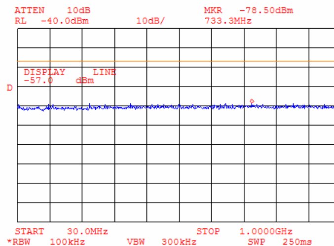
Plot 9.3.5 Spurious emission test results at antenna port 4 in 30 – 1000 MHz range
