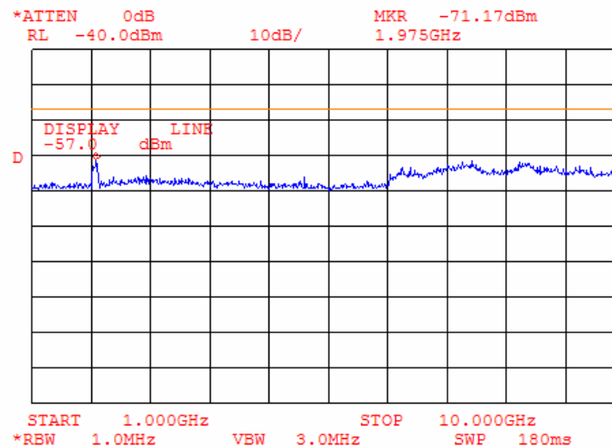
Plot 9.3.12 Spurious emission test results at antenna port 4 in 1.0 – 10.0 GHz range
