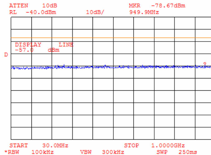
Plot 9.3.4 Spurious emission test results at antenna port 3 in 30 – 1000 MHz range
