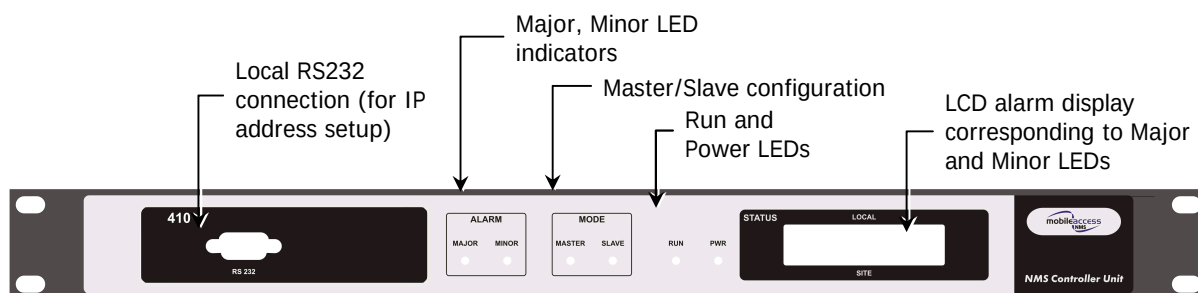
Figure 2-13. MobileAccess 410 Front Panel
