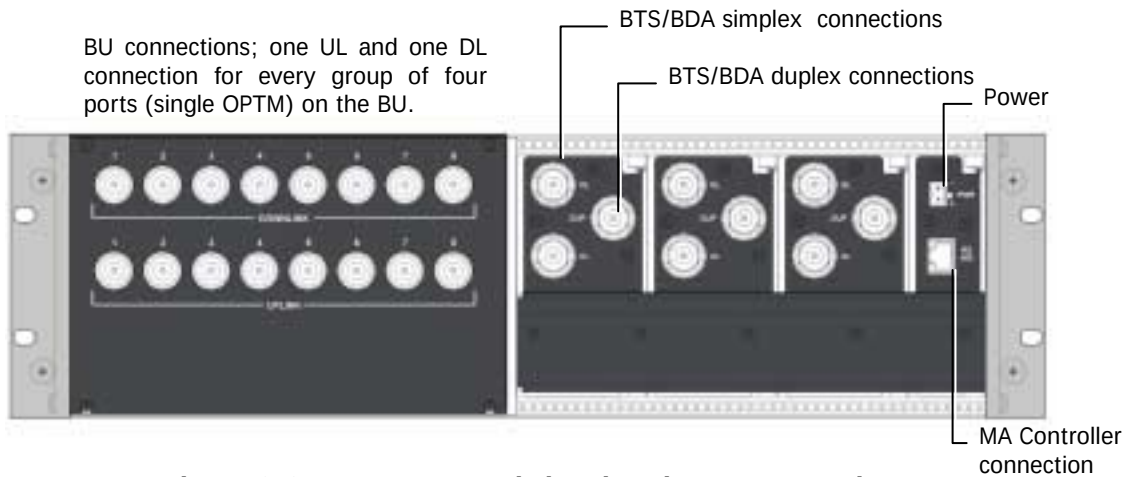
Figure 2-9. RIU Rear Panel showing the RF Connection
