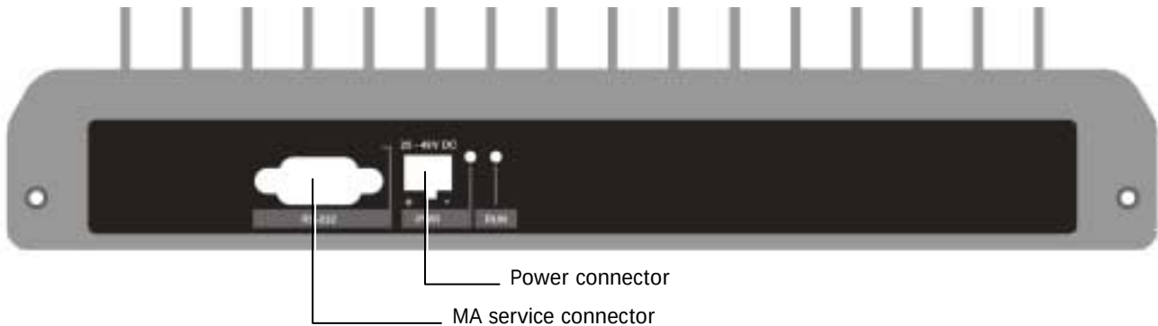
Figure 2-3. RHU 1200 Front panels
