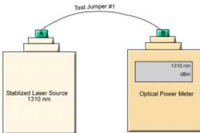
Figure 5-1. Set Up
