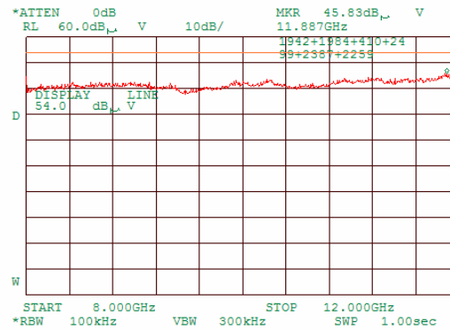
Plot 8.1.20 Radiated emission measurements in 8000- 12000 MHz range, horizontal antenna polarization, iDEN uplink mode
