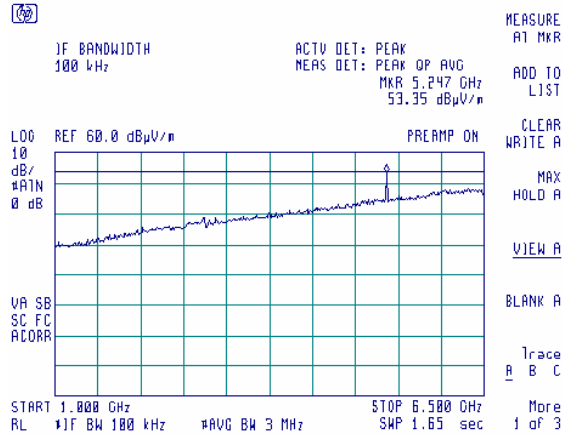
Plot 8.1.4 Radiated emission measurements in 1000- 6500 MHz range, horizontal antenna polarization, SMR uplink mode
