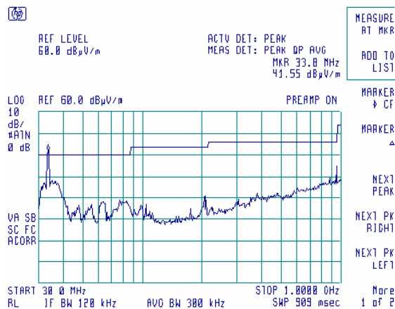
Plot 8.1.14 Radiated emission measurements in 30- 1000 MHz range, horizontal antenna polarization, iDEN uplink mode
