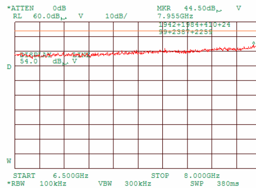
Plot 8.1.18 Radiated emission measurements in 6500- 8000 MHz range, horizontal antenna polarization, iDEN uplink mode
