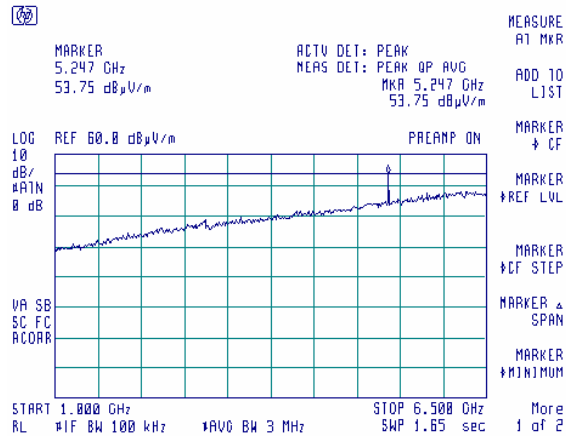
Plot 8.1.16 Radiated emission measurements in 1000- 6500 MHz range, horizontal antenna polarization, iDEN uplink mode
