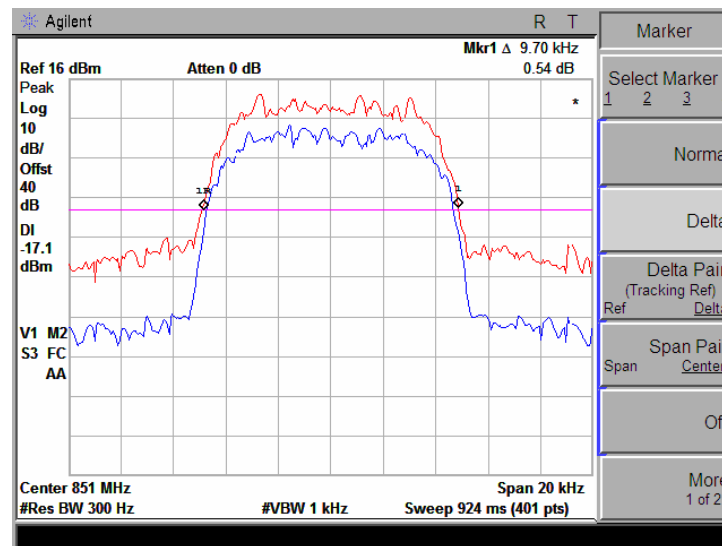
Plot 7.2.2 Occupied bandwidth measurements at mid frequency carrier. Port 1
