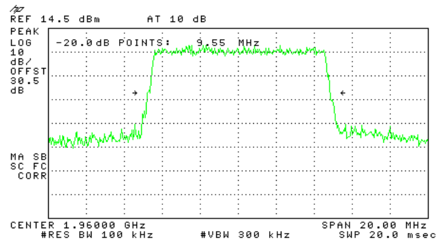
Figure 72.— Input 1960 MHz
