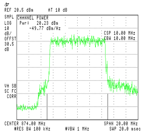
Figure 7.— 874 MHz
