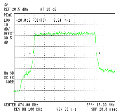
Figure 27.— Input 874
