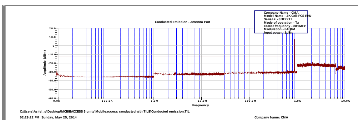
Figure 41.— 881 MHz
