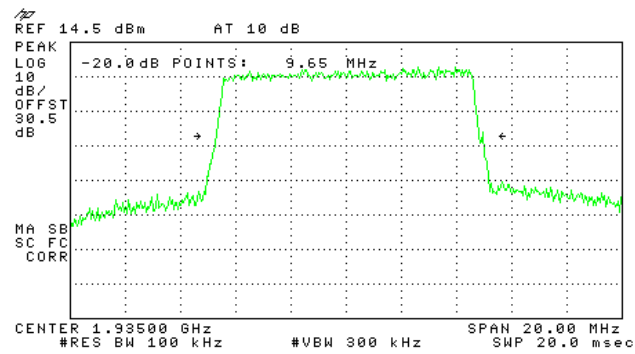
Figure 70.— Input 1935 MHz
