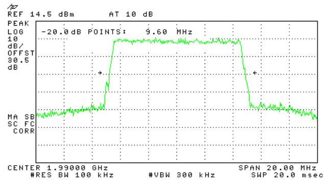
Figure 80.— Input 1990 MHz
