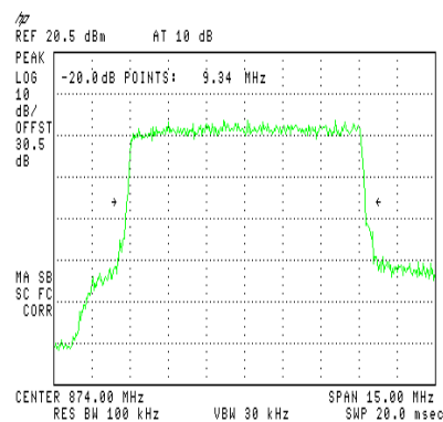
Figure 21.— Input 874
