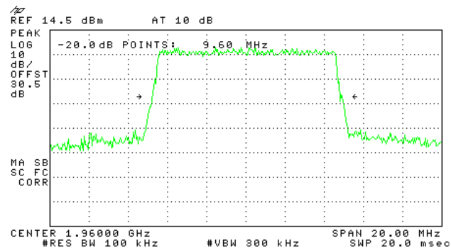
Figure 78.— Input 1960 MHz
