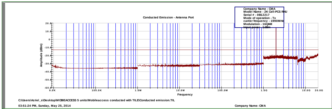
Figure 88.— 1990MHz
