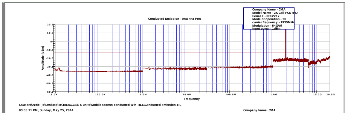
Figure 89.— 1935MHz
