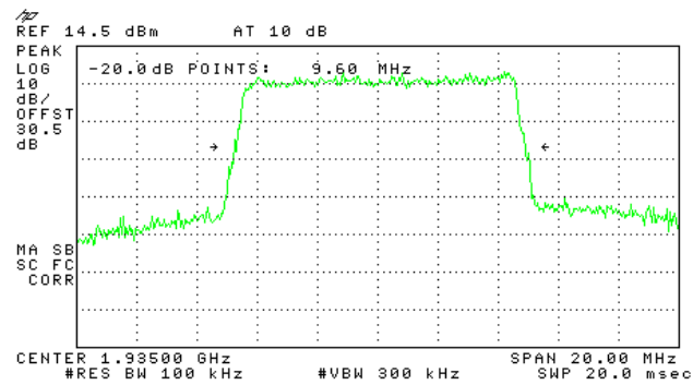
Figure 76.— Input 1935 MHz
