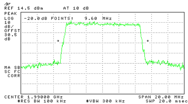
Figure 74.— Input 1990 MHz
