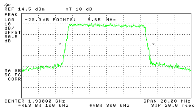
Figure 68.— Input 1990 MHz
