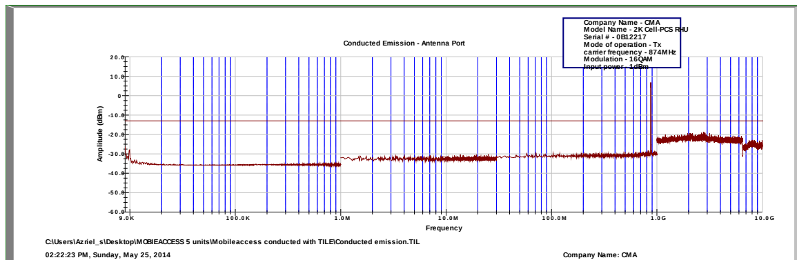
Figure 37.— 874 MHz
