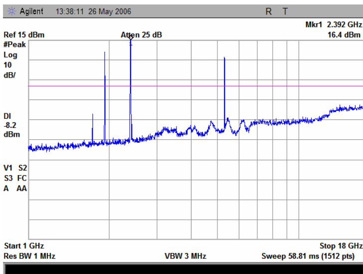
Plot 7.3.64 Spurious emission measurements in 1000 - 18000 MHz range at low carrier frequency, DSSS modulation
