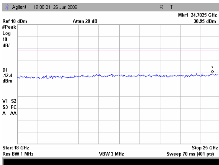
Plot 7.3.144 Spurious emission measurements in 18 - 25 GHz range at high carrier frequency, OFDM modulation
