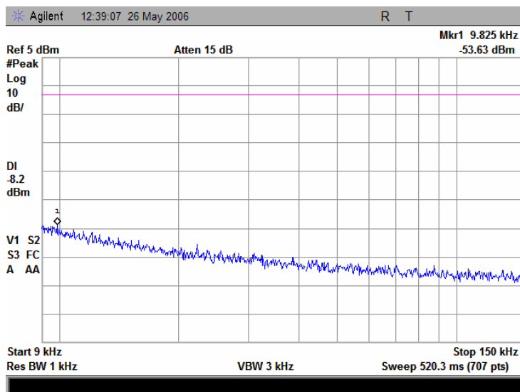
Plot 7.3.74 Spurious emission measurements in 9 - 150 kHz range at mid carrier frequency, OFDM modulation
