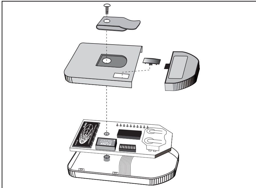
Figure 5: CMD-HHCP-xxx Assembly
