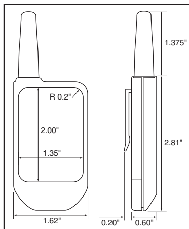
Figure 1: Physical Dimensions
