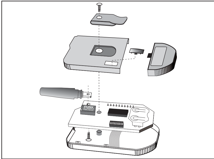
Figure 5: CMD-HHLR-xxx Assembly
