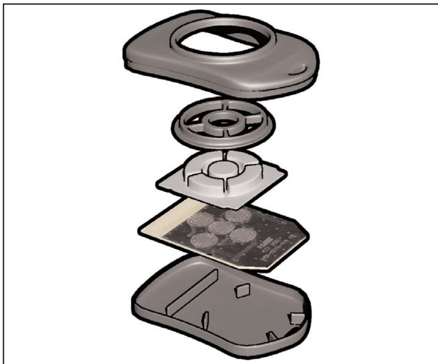
Figure 5: CMD-KEY#-xxx Assembly
