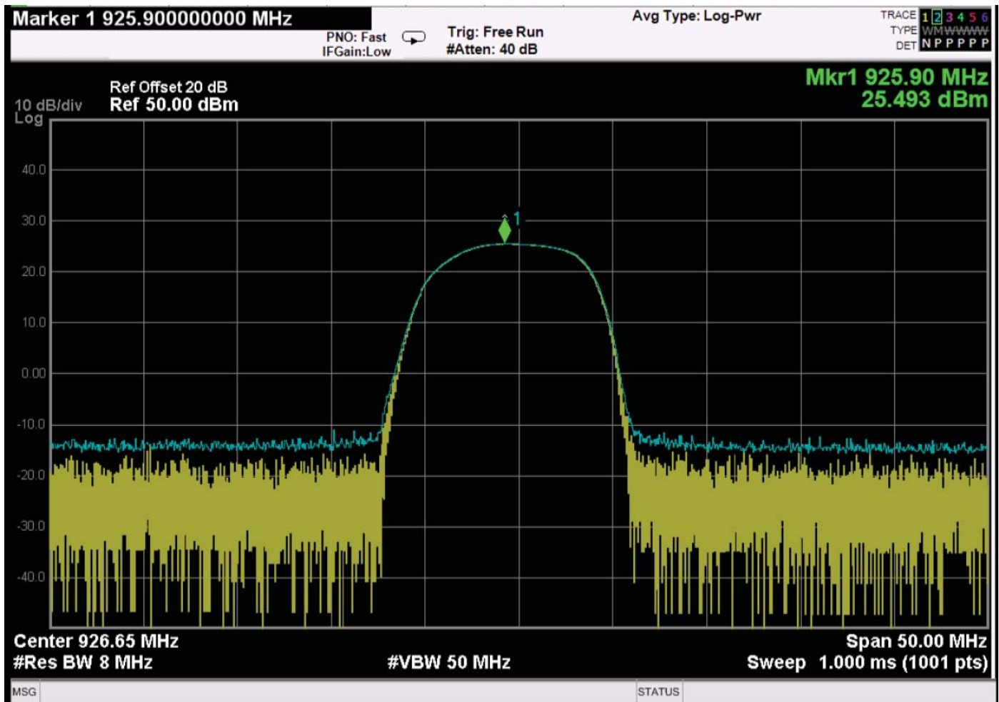
Peak Power Output – High Channel – Edge Mount – Low Data Rate
