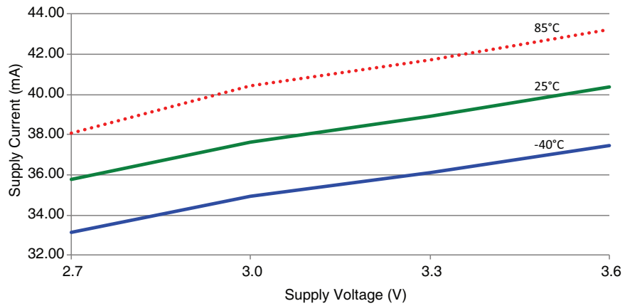
Figure 11: HumPRO-A™ Series Transceiver RX Scan Current vs. Supply Voltage, 115.2kbps
