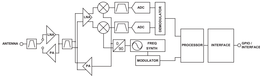
Figure 19: HumPRO-A™ Series Transceiver RF Section Block Diagram
