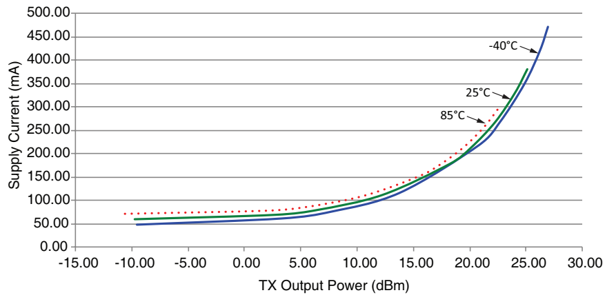
Figure 7: HumPRO-A™ Series Transceiver Average TX Current vs. Transmitter Output Power at 3.3V
