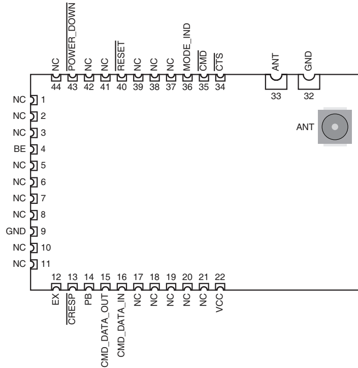
Figure 14: HumPRO-A™ Series Transceiver Pin Assignments (Top View)
