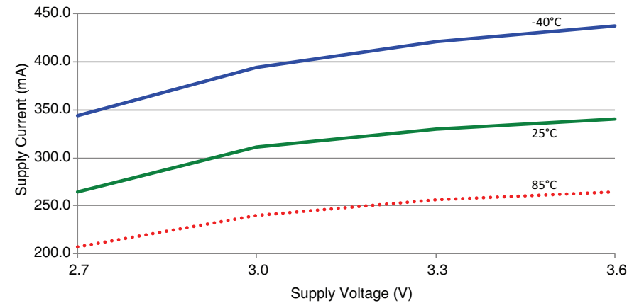
Figure 8: HumPRO-A™ Series Transceiver TX Current vs. Supply Voltage at 24dBm
