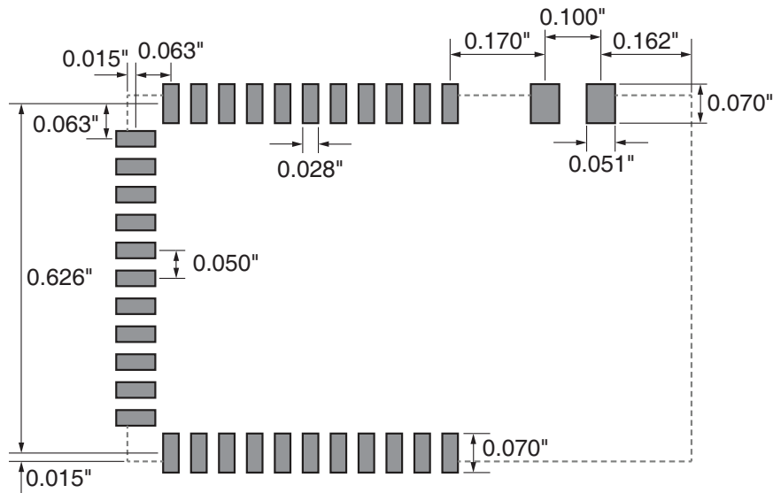
Figure 109: HUM-A-***-PRO Recommended PCB Layout
