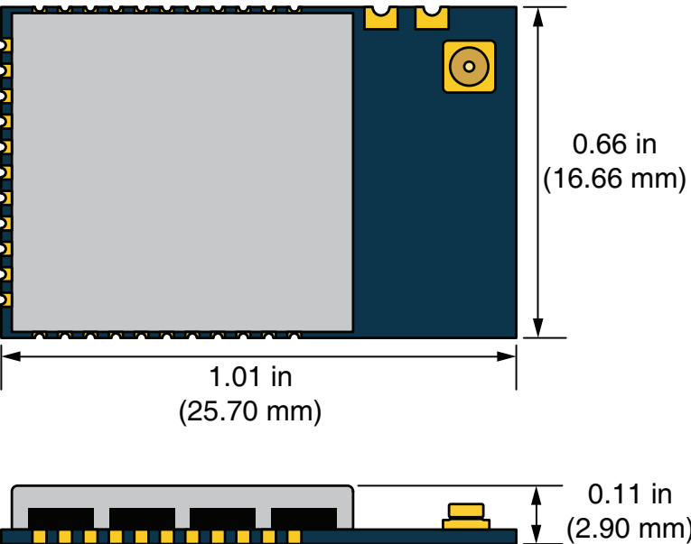
Figure 18: HumPRO-A™ Series Transceiver Pre-certified Version Dimensions
