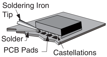
Figure 113: Soldering Technique
