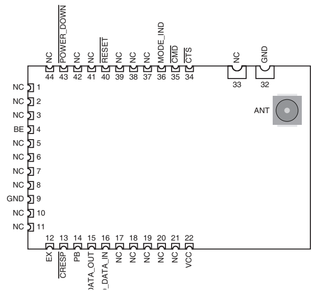
Figure 17: HumPRO-A™ Series Transceiver Pre-certified Version Pin Assignments - UFL Connection (Top View)
