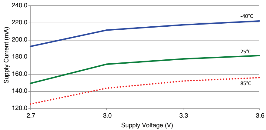
Figure 10: HumPRO-A™ Series Transceiver TX Current vs. Supply Voltage at 20dBm
