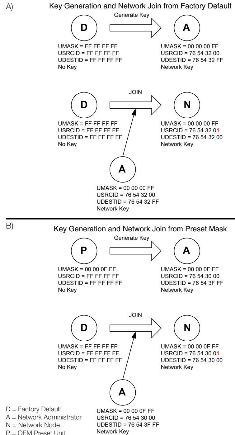
Figure 30: HumPRO-A™ Series JOIN Process
