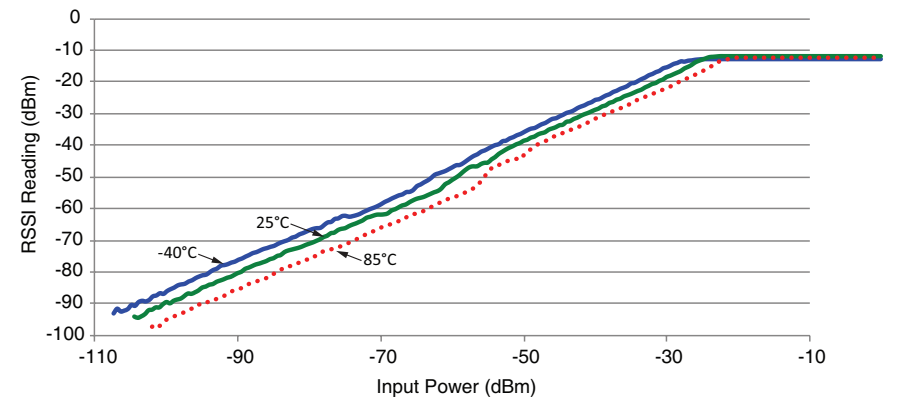
Figure 13: HumPRO-A™ Series Transceiver RSSI Reading vs. Input Power
