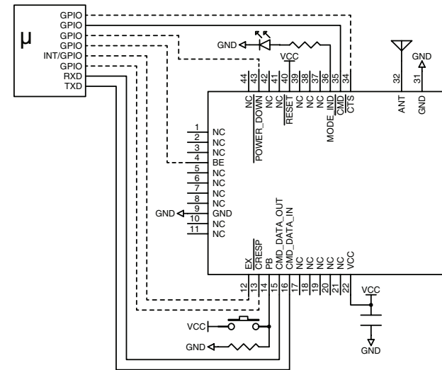
Figure 106: HumPRO-A™ Series Transceiver Basic Application Circuit
