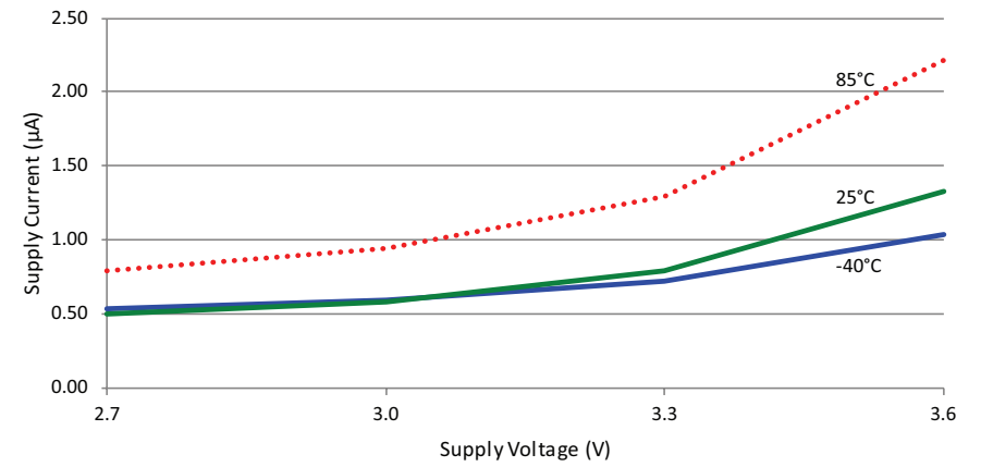
Figure 12: HumPRO-A™ Series Transceiver Standby Current Consumption vs. Supply Voltage
