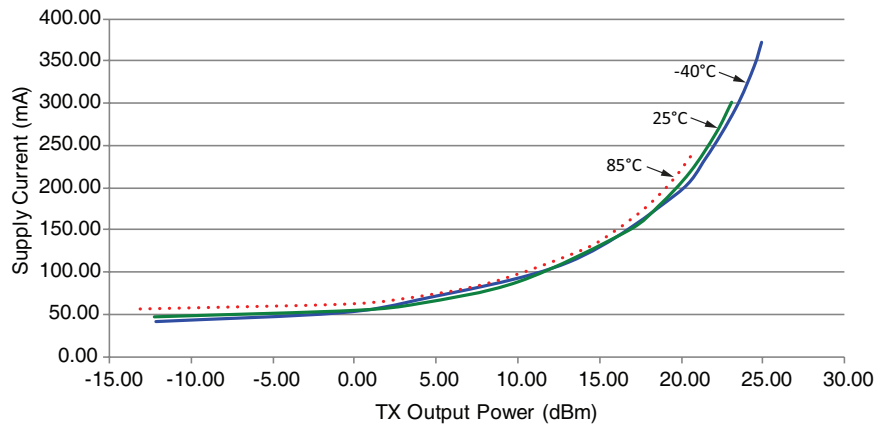
Figure 6: HumPRO-A™ Series Transceiver Average Current vs. Transmitter Output Power at 2.5V
