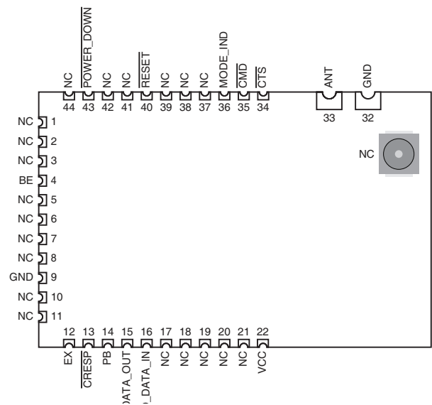
Figure 16: HumPRO-A™ Series Transceiver Pre-certified Version Pin Assignments - Castellation Connection (Top View)
