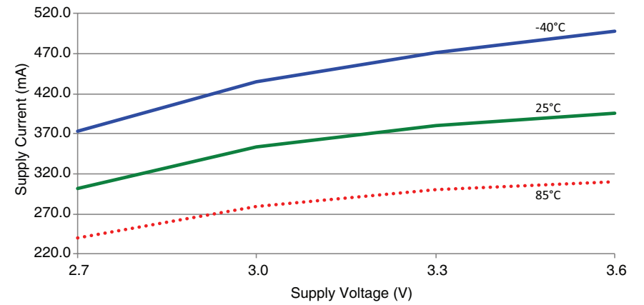
Figure 9: HumPRO-A™ Series Transceiver TX Current vs. Supply Voltage at Max Power
