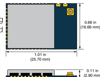
Figure 1: Package Dimensions
