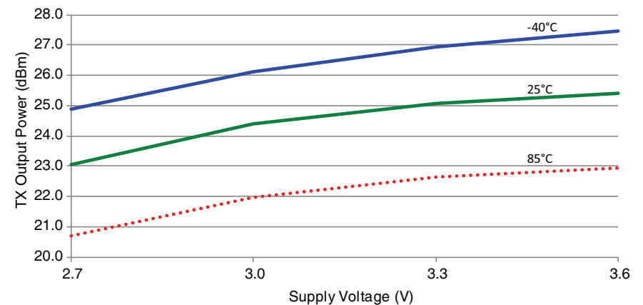
Figure 5: HumPRO-A™ Series Transceiver Max Output Power vs. Supply Voltage
