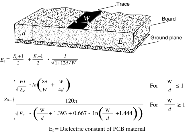
Figure 110: Microstrip Formulas
