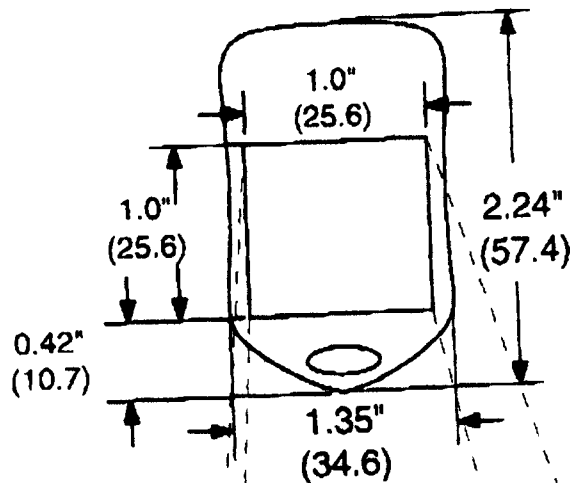
Back of CMD-KEYX-4XX
