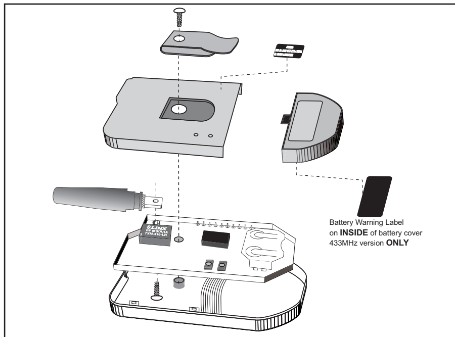
Figure 5: OTX-***-HH-LR8-MS Assembly
