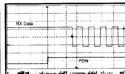
Figure 3: PDN to valid RX data
