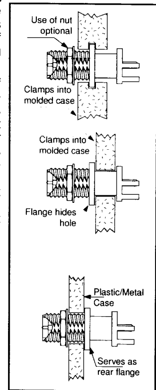
Figure 11: Mounting Options
