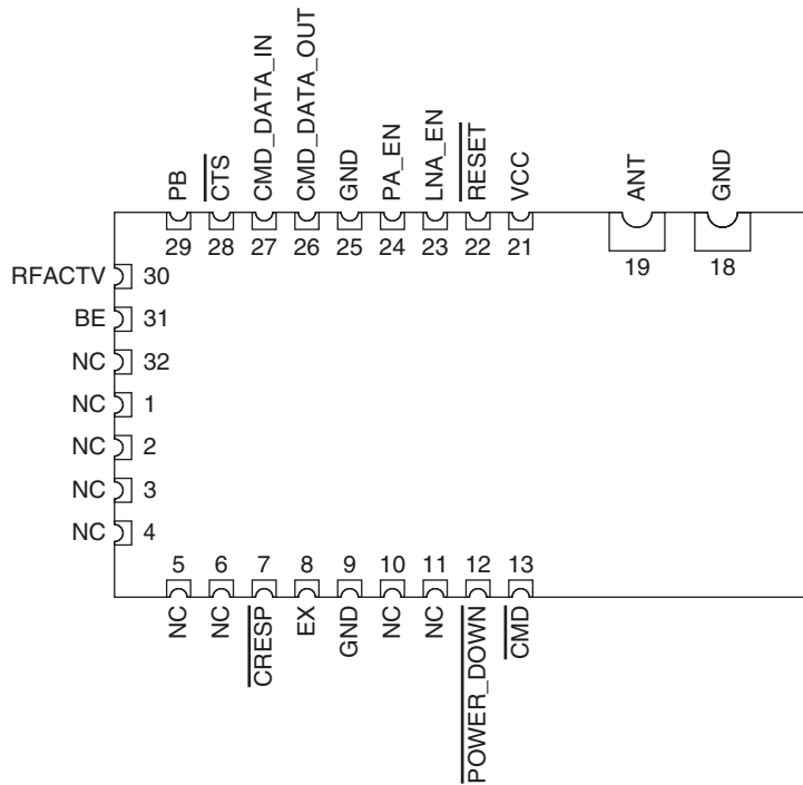
Figure 28: HumRC™ Series Transceiver Pre-certified Version Pin Assignments (Top View)
