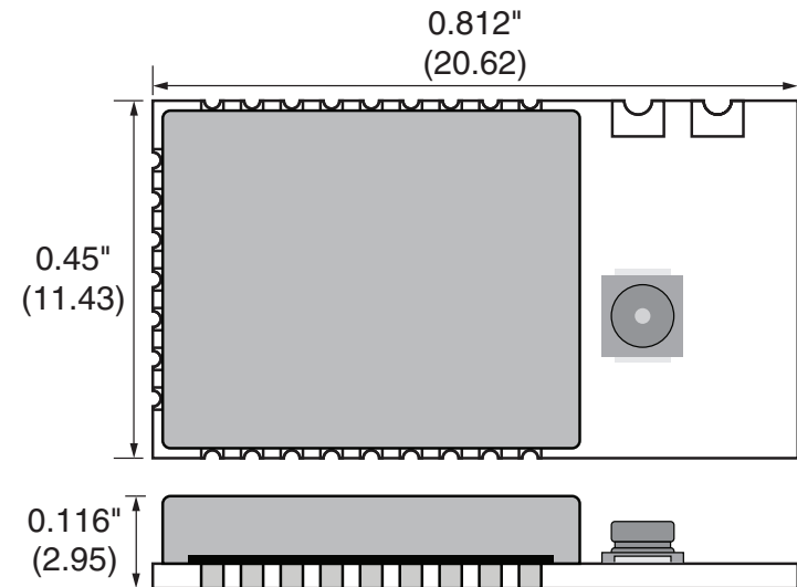
Figure 30: HumRC™ Series Transceiver Pre-certified Version Dimensions
