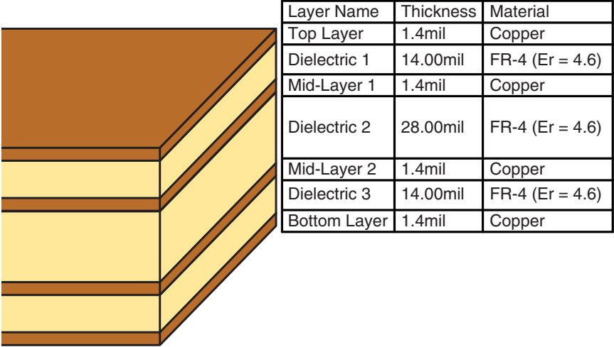
Figure 45: HumRC™ Series Transceiver Castellation Version Reference Design PCB Stack
