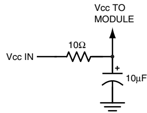
Figure 47: Supply Filter
