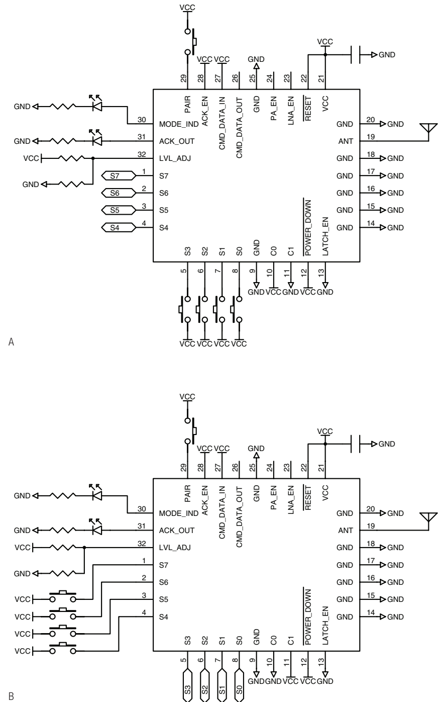
Figure 41: HumRC™ Series Transceiver Basic Application Circuits for Bi-directional Remote Control
