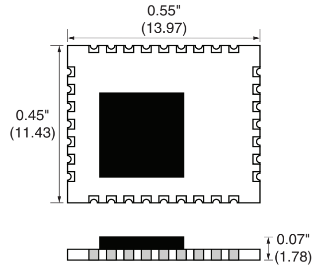
Figure 29: HumRC™ Series Transceiver Dimensions
