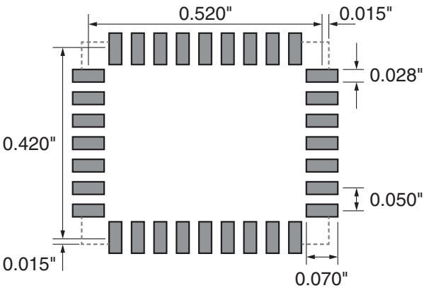
Figure 49: HUM-***-RC Recommended PCB Layout
