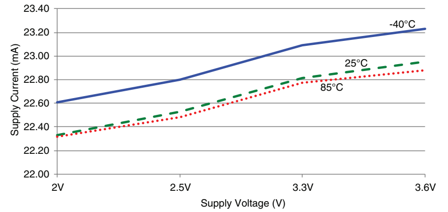
Figure 8: HumPRC™ Series Transceiver TX Current vs. Supply Voltage at 0dBm
