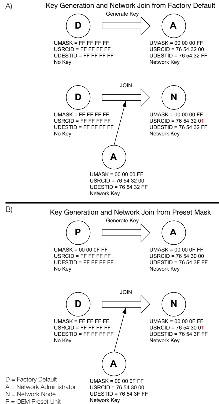
Figure 23: HumPRC™ Series and HumPRO™ Series Join Process Examples
