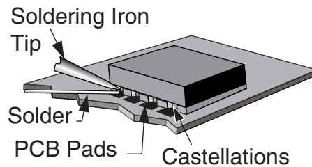
Figure 100: Soldering Technique
