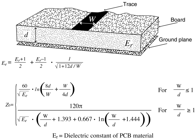
Figure 97: Microstrip Formulas
