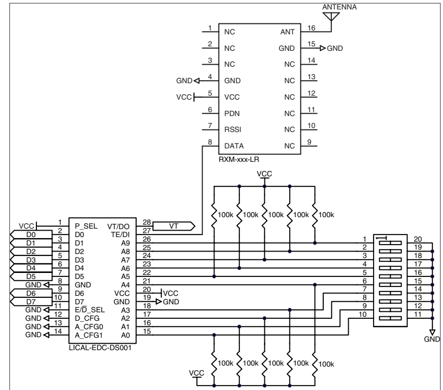
The decoder has ten address lines that must match the transmitter address lines. A DIP switch is commonly used to set these, but they can also be hardwired. As long as the address lines match, when a button on the transmitter is pressed, a corresponding data line on the decoder (D0–D7) goes high. These data lines can then be connected to external circuitry to perform whatever function is required by the application.
