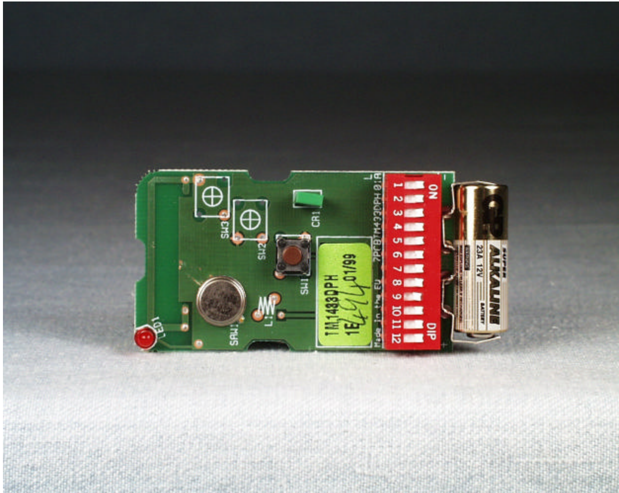
Component Side
