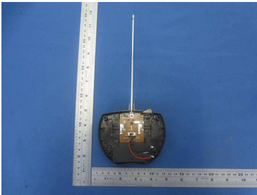
(Antenna Type 2: telescope antenna with unique antenna connector)
