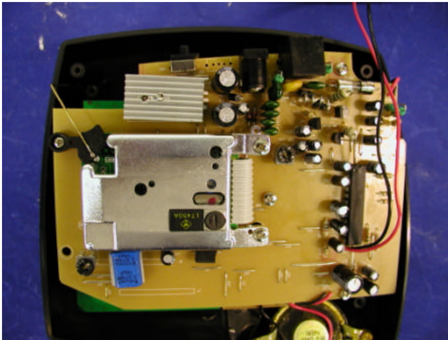
Base Main Board and Housing
