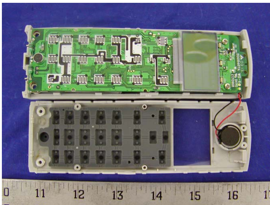
Handset – Housing and Main Board Solder View
