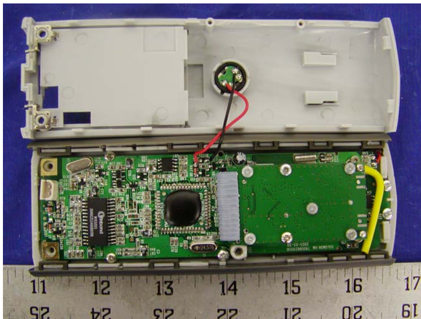
Handset – Housing and Board Component View
