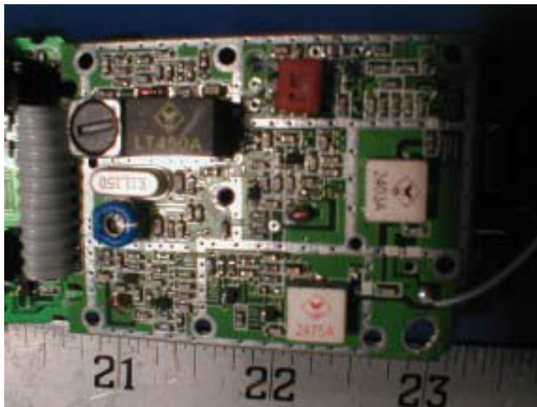
Handset Transmitter - Solder View
