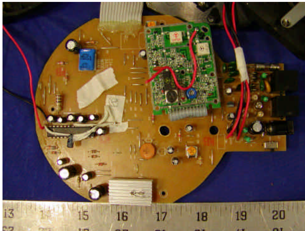
Base – Component
