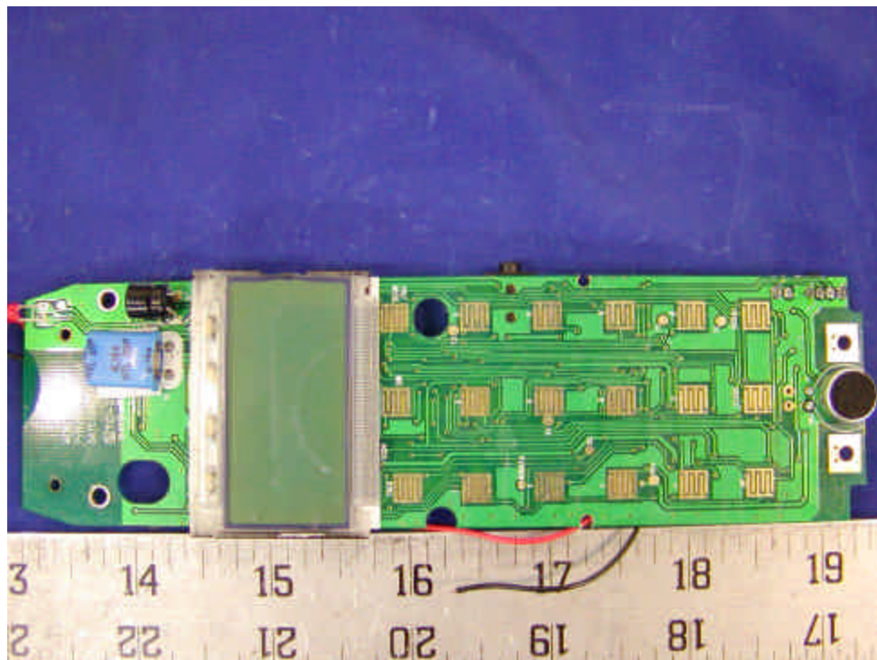
Handset – Solder
