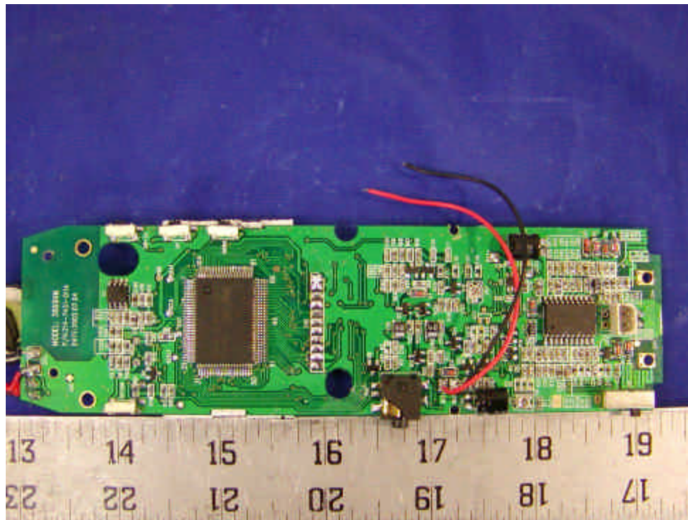
Handset – Solder
