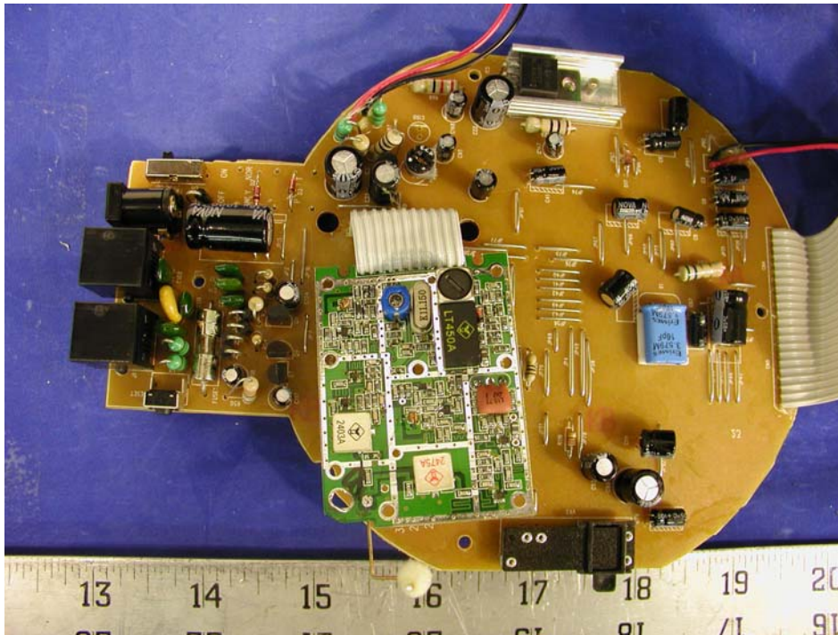
Base Main Board - Component View
