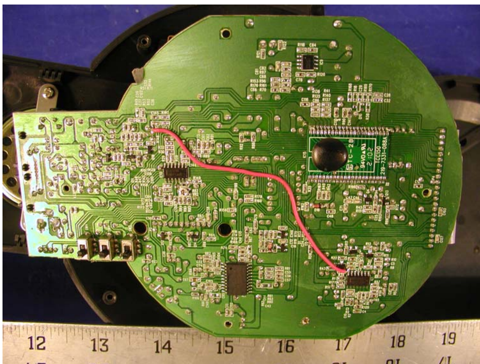
Base Main Board - Solder View
