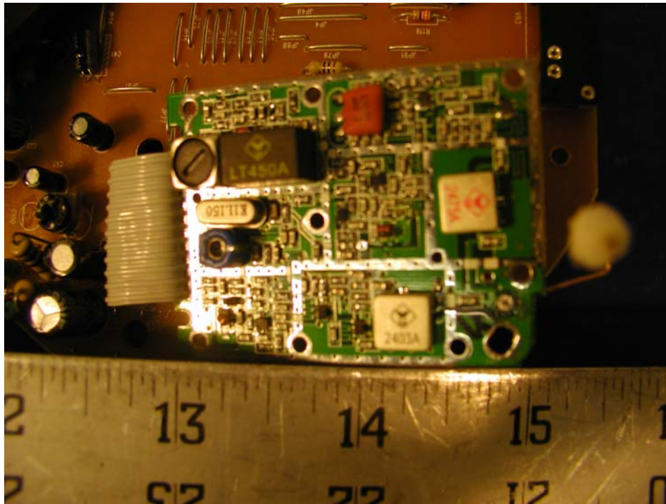
Base Transmitter - Component View
